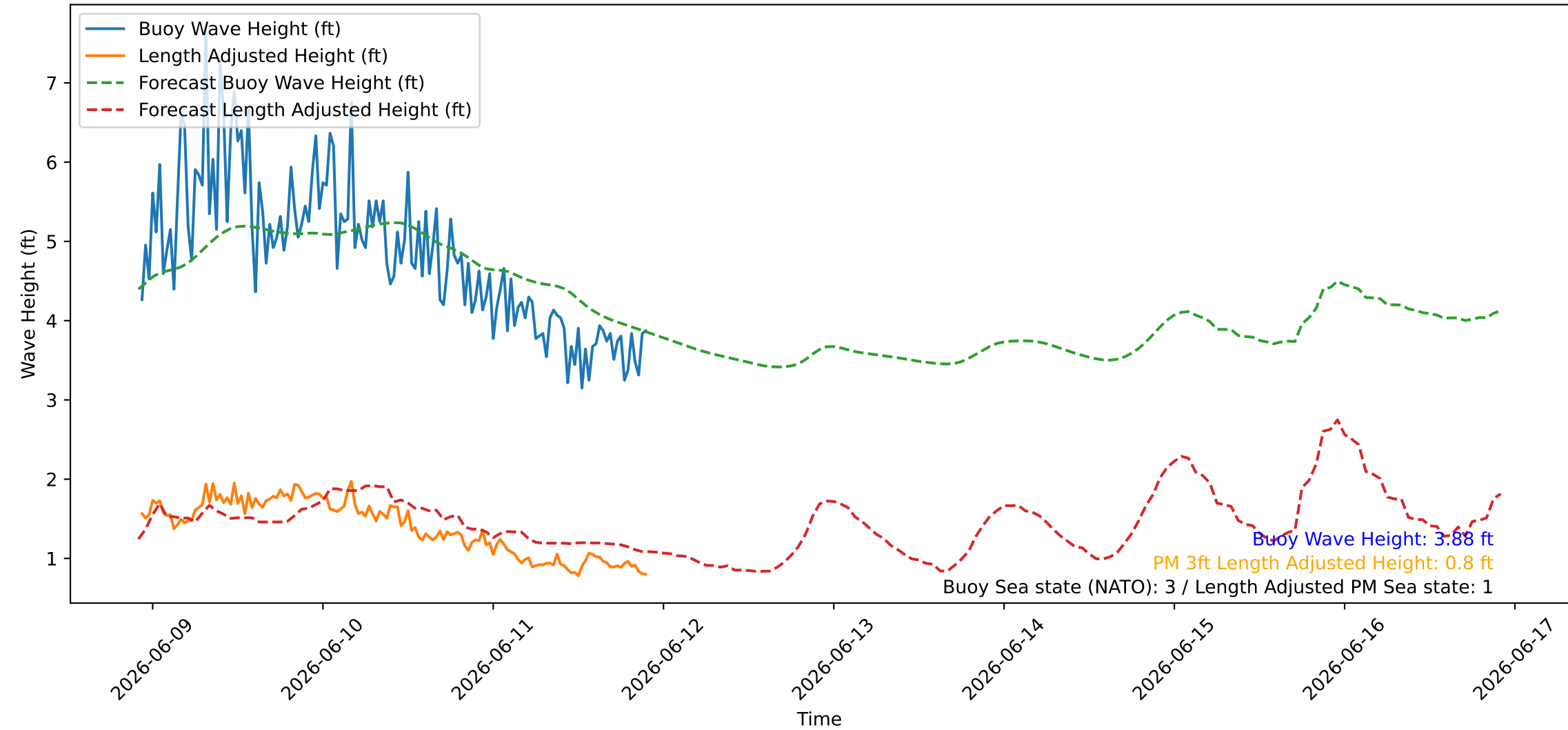
Wave Heights over Time for Red Beach at 2026-06-11 22:20:47
