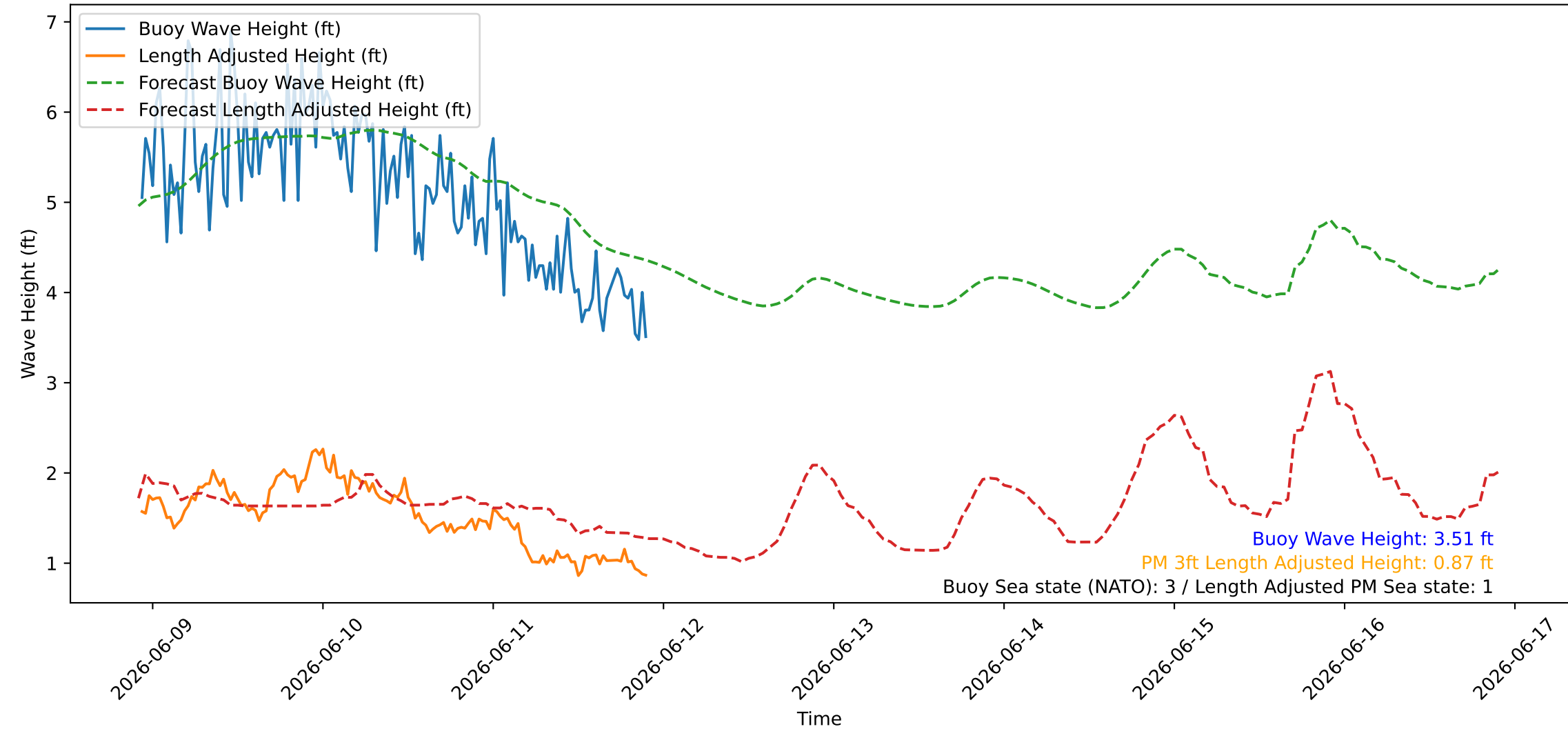
Wave Heights over Time for Green Beach at 2026-06-11 22:21:10
