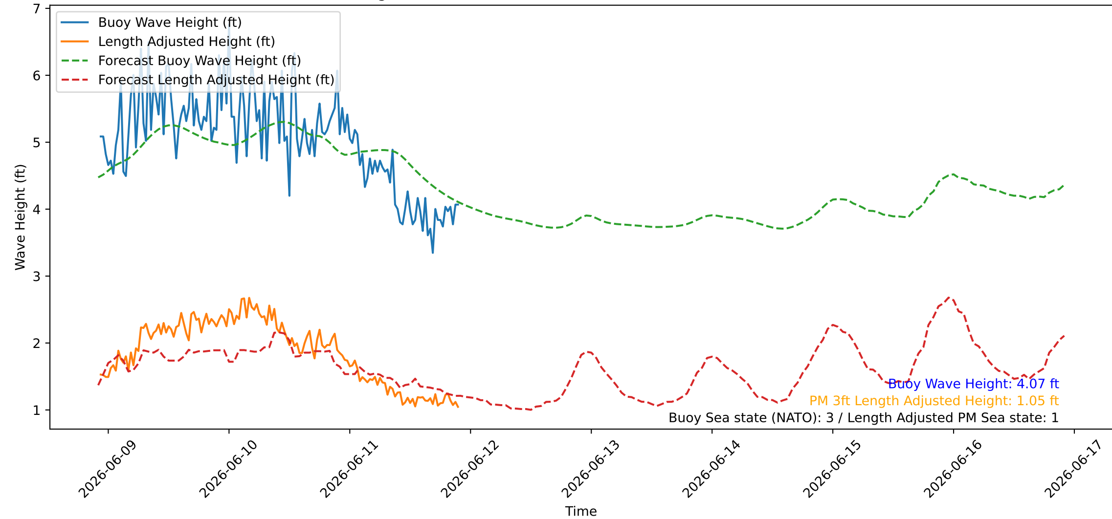
Wave Heights over Time for Oceanside Harbor at 2026-06-11 22:20:26
