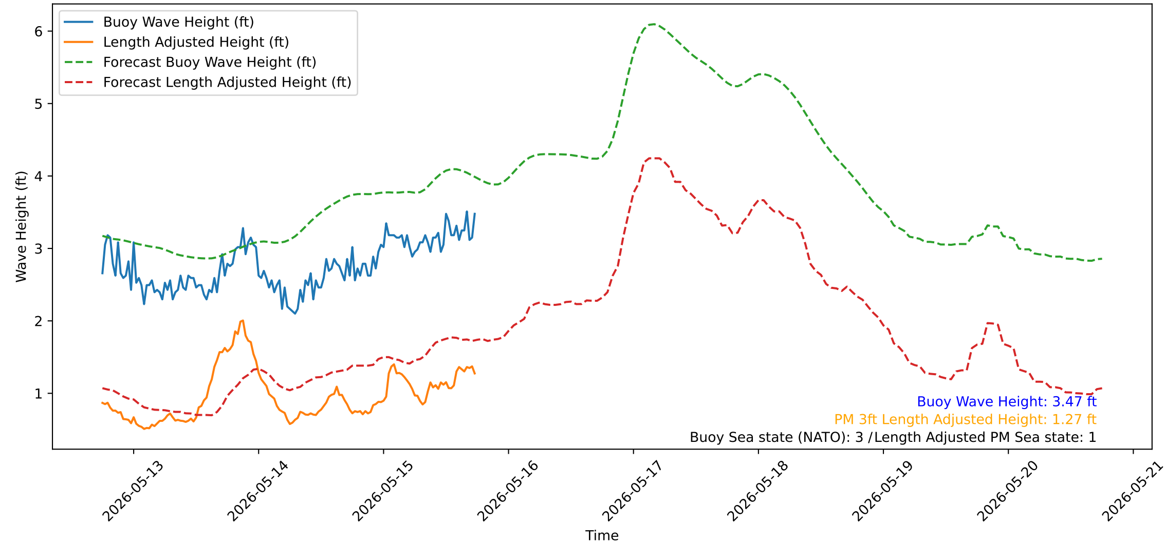
Wave Heights over Time for Green Beach at 2026-05-15 18:11:13
