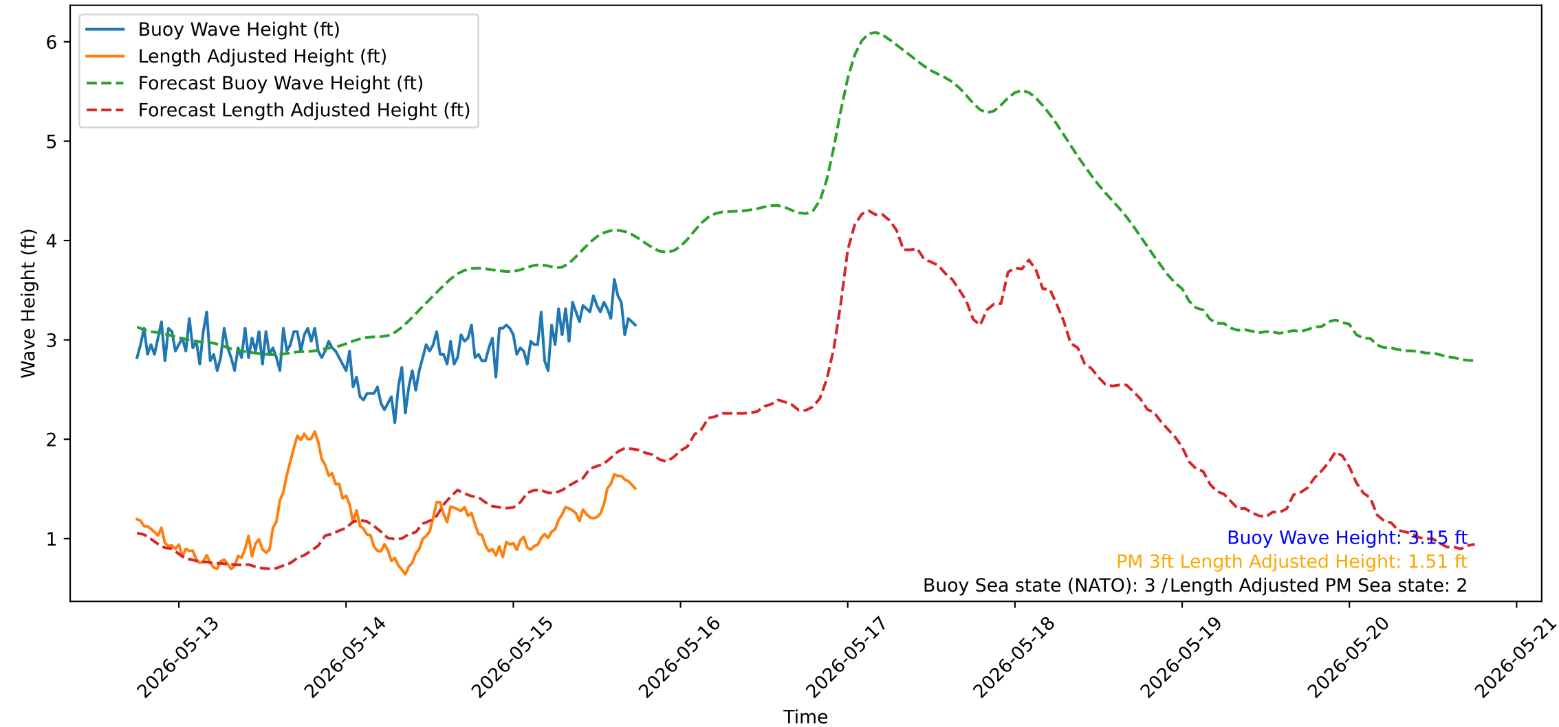
Wave Heights over Time for Oceanside Harbor at 2026-05-15 18:10:32
