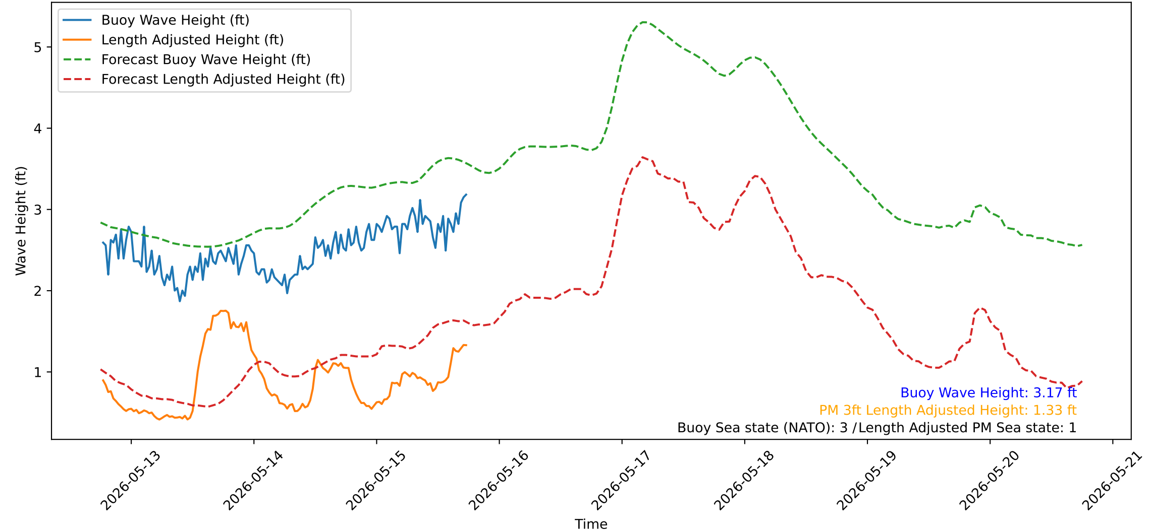
Wave Heights over Time for Red Beach at 2026-05-15 18:10:51
