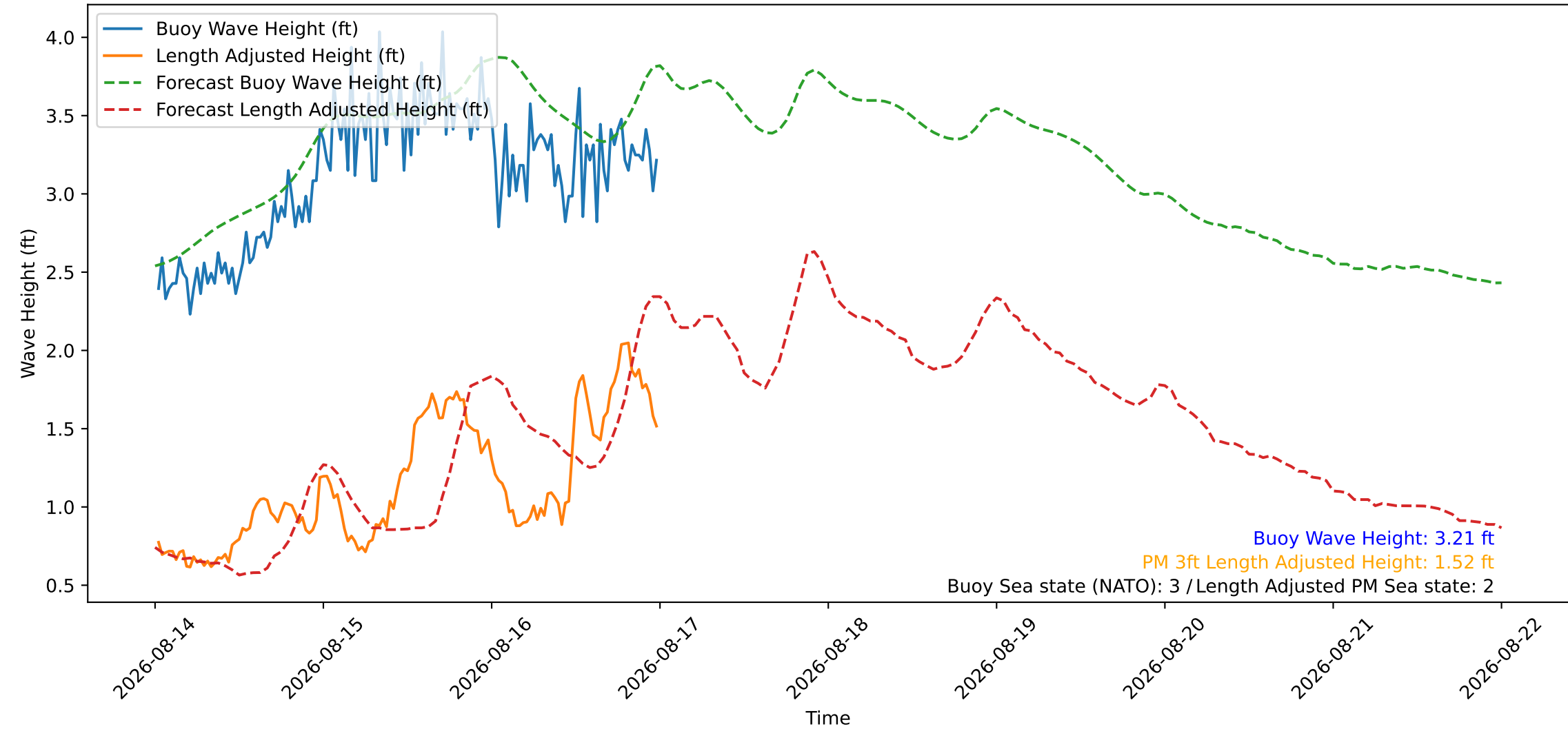
Wave Heights over Time for Red Beach at 2026-08-17 00:10:45
