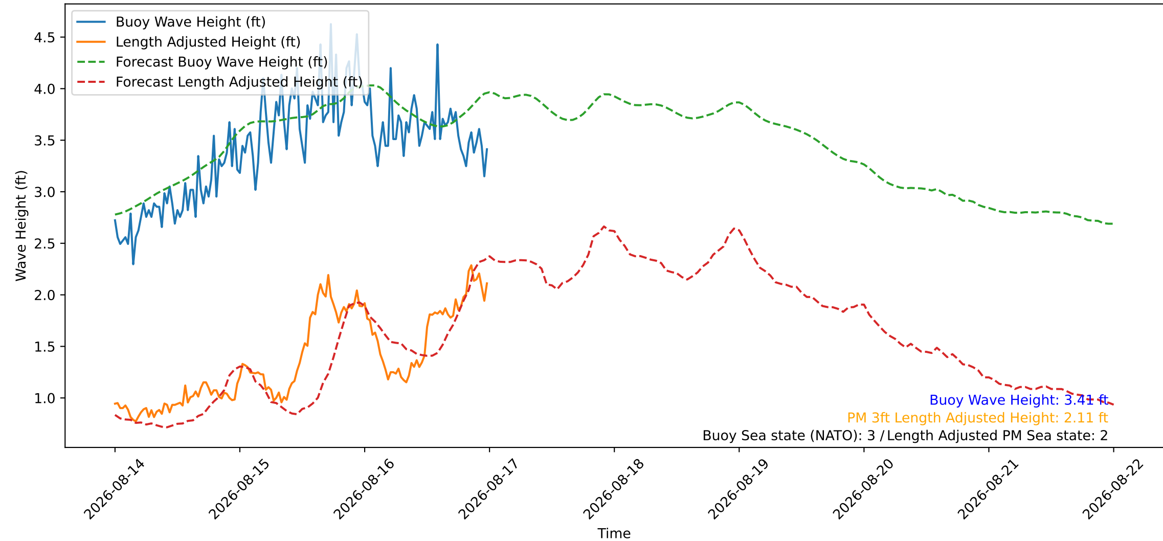
Wave Heights over Time for Oceanside Harbor at 2026-08-17 00:10:26
