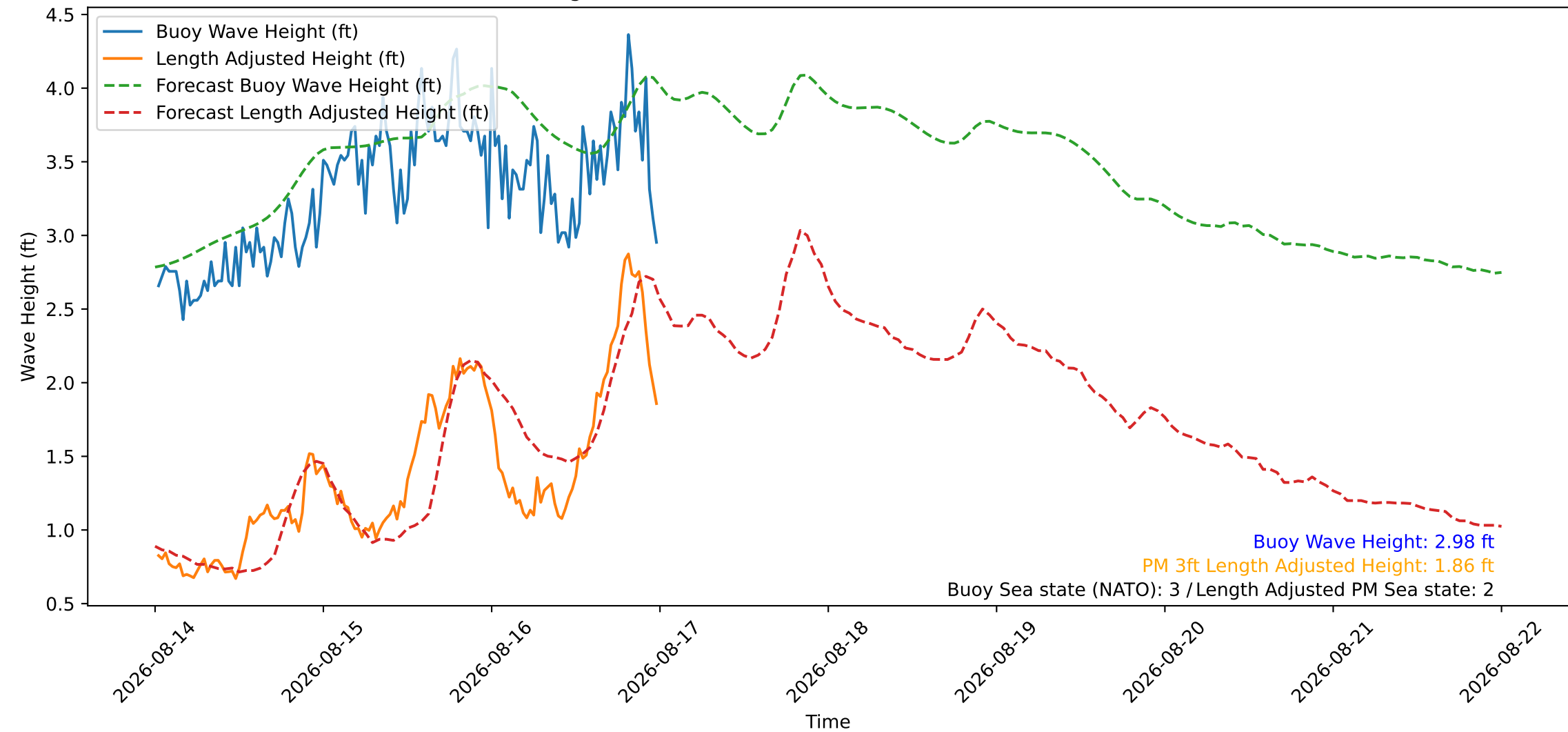
Wave Heights over Time for Green Beach at 2026-08-17 00:11:08
