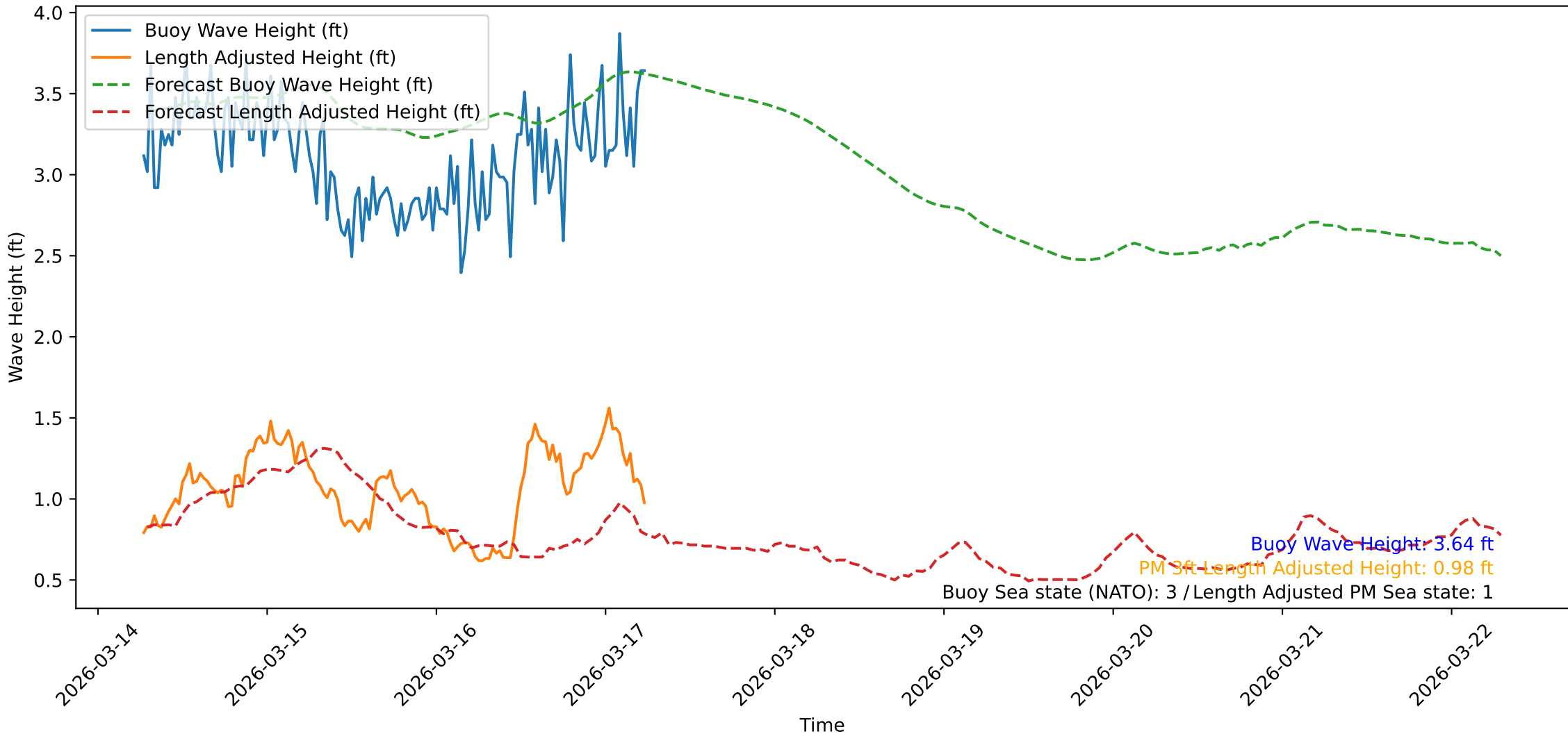
Wave Heights over Time for Oceanside Harbor at 2026-03-17 06:30:46
