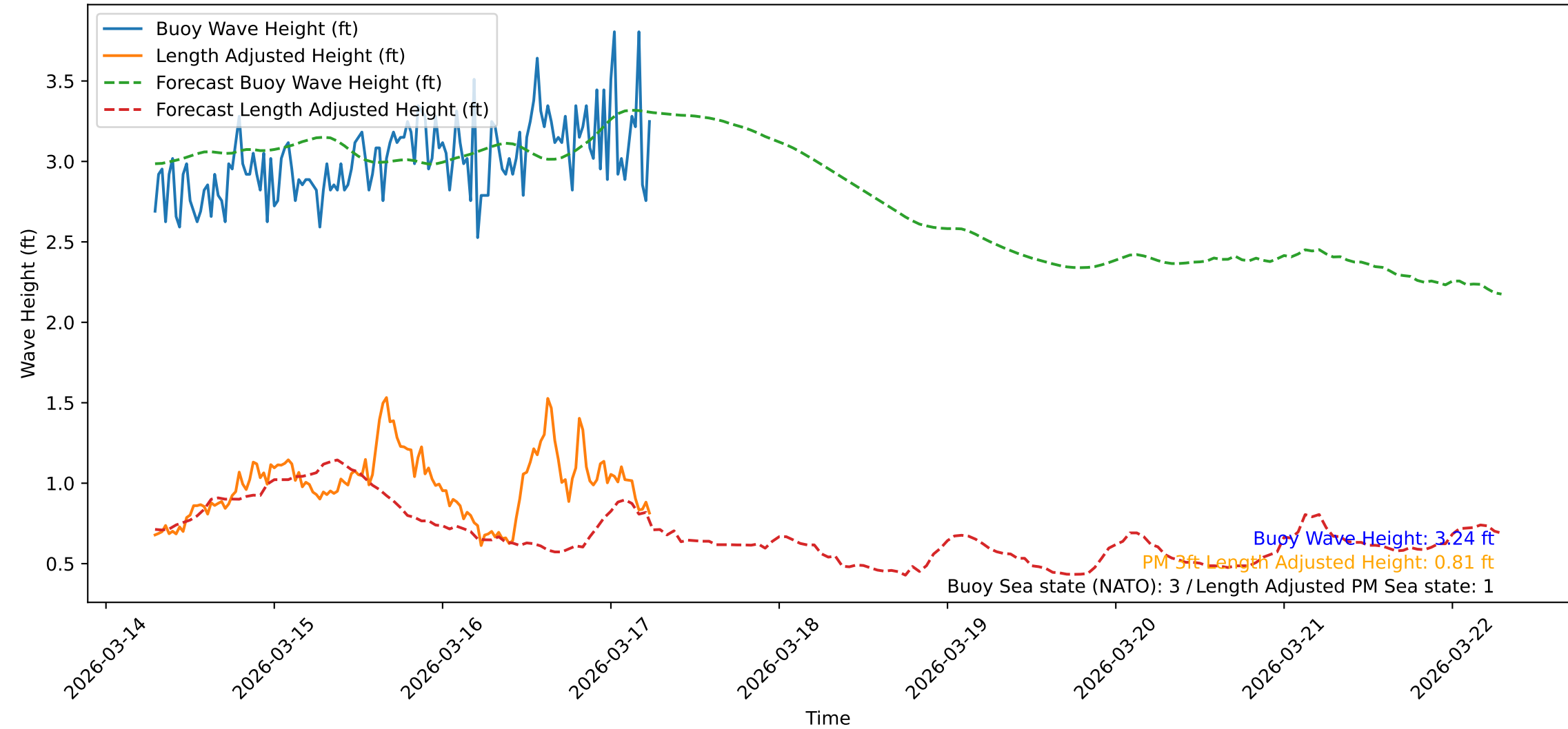
Wave Heights over Time for Red Beach at 2026-03-17 06:31:09
