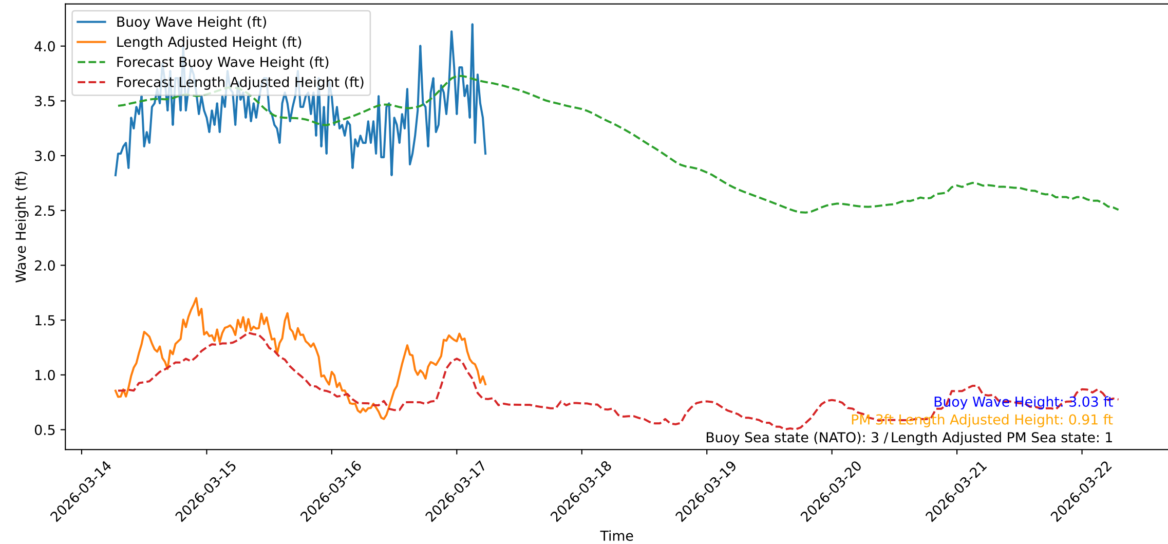
Wave Heights over Time for Green Beach at 2026-03-17 06:31:52
