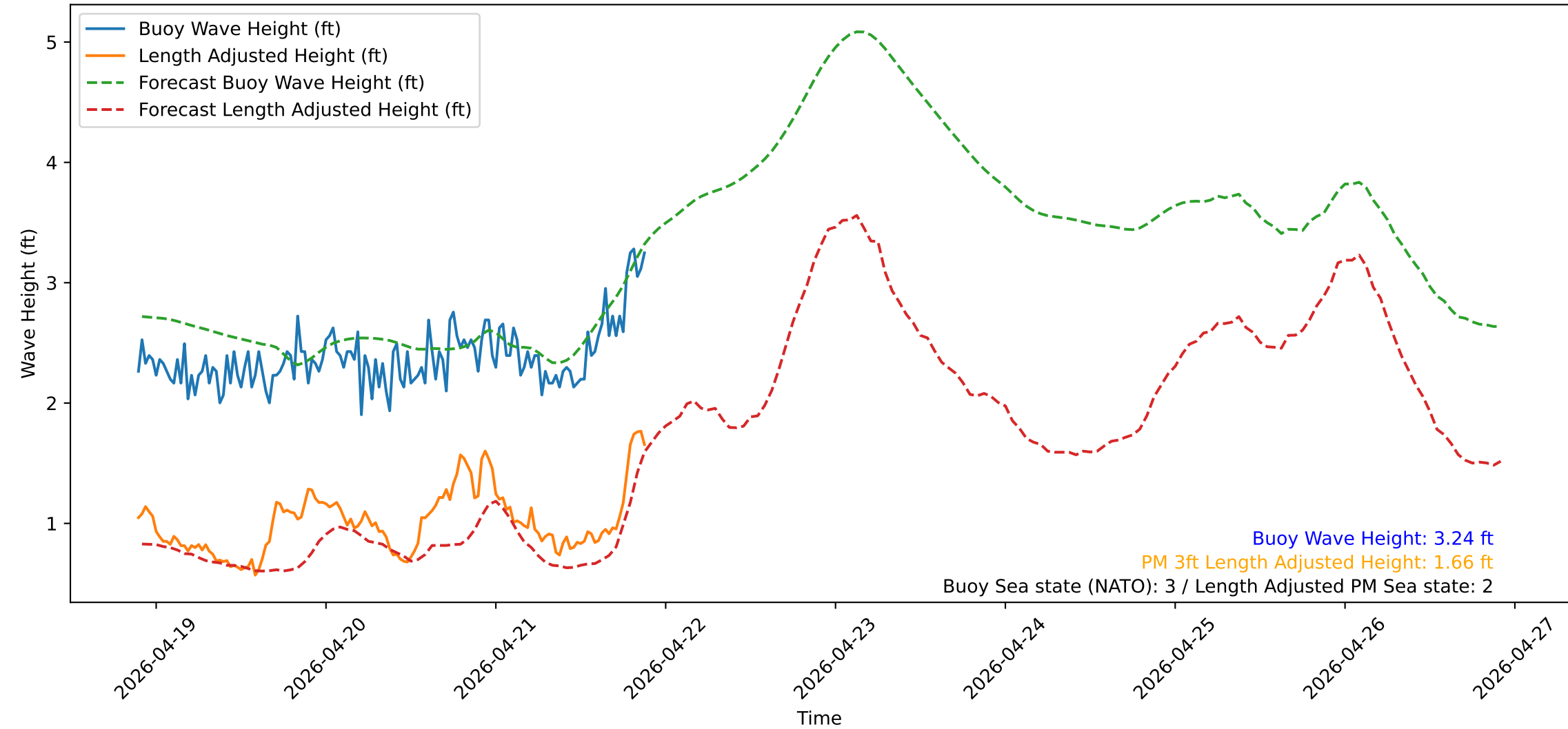
Wave Heights over Time for Oceanside Harbor at 2026-04-21 21:40:31
