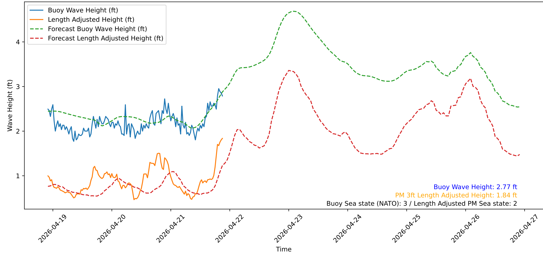
Wave Heights over Time for Red Beach at 2026-04-21 21:40:51
