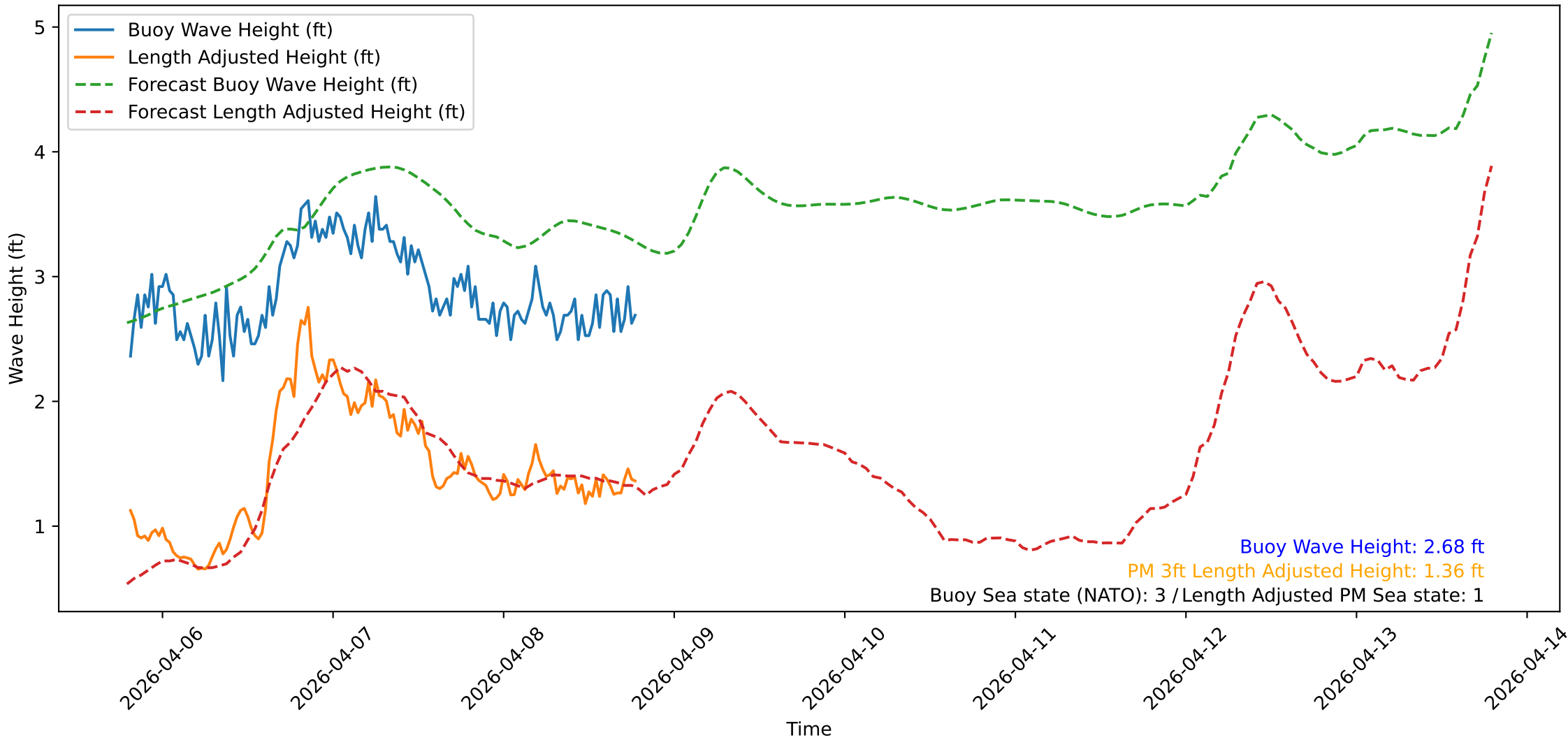
Wave Heights over Time for Oceanside Harbor at 2026-04-08 19:20:32
