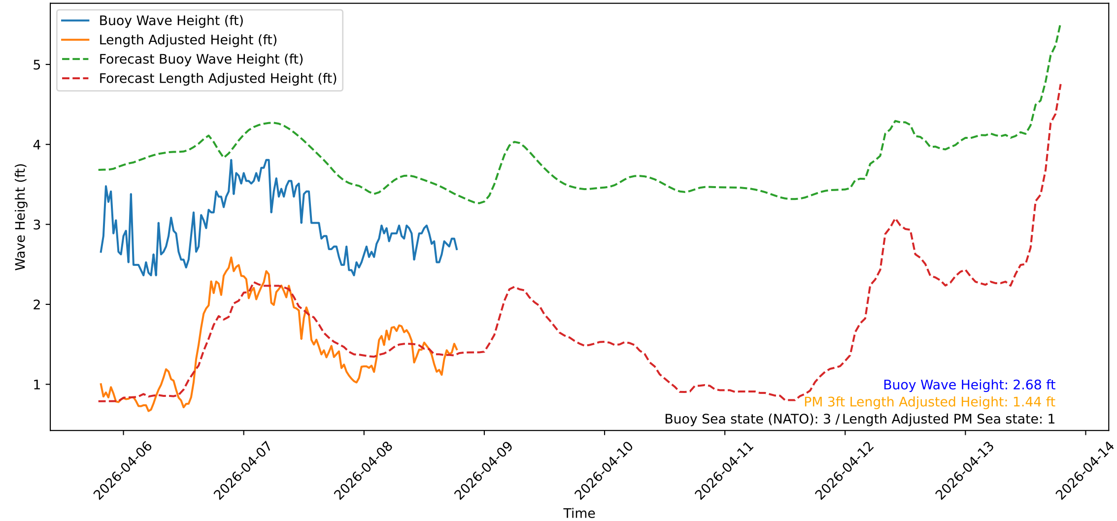
Wave Heights over Time for Green Beach at 2026-04-08 19:21:11
