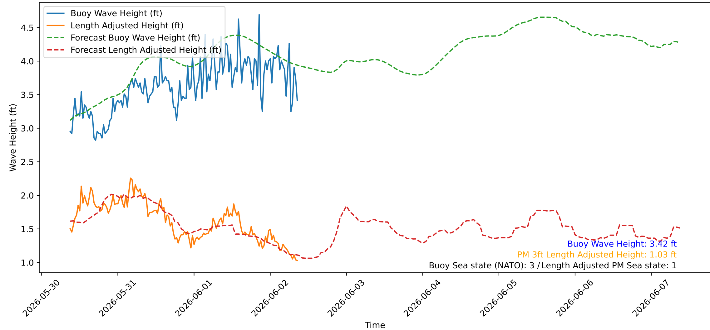
Wave Heights over Time for Oceanside Harbor at 2026-06-02 09:00:26
