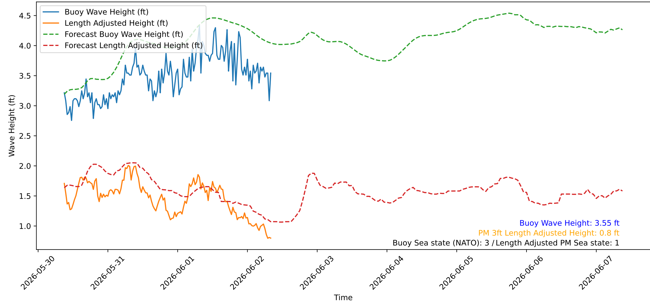
Wave Heights over Time for Green Beach at 2026-06-02 09:01:08
