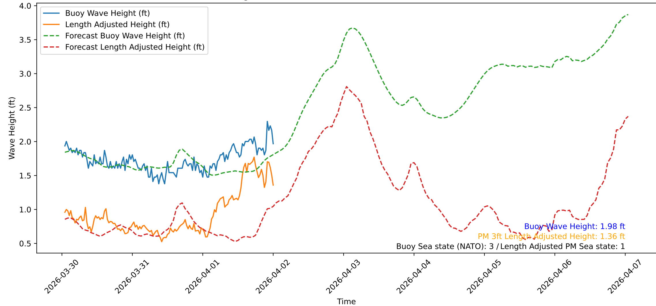
Wave Heights over Time for Red Beach at 2026-04-02 00:40:48
