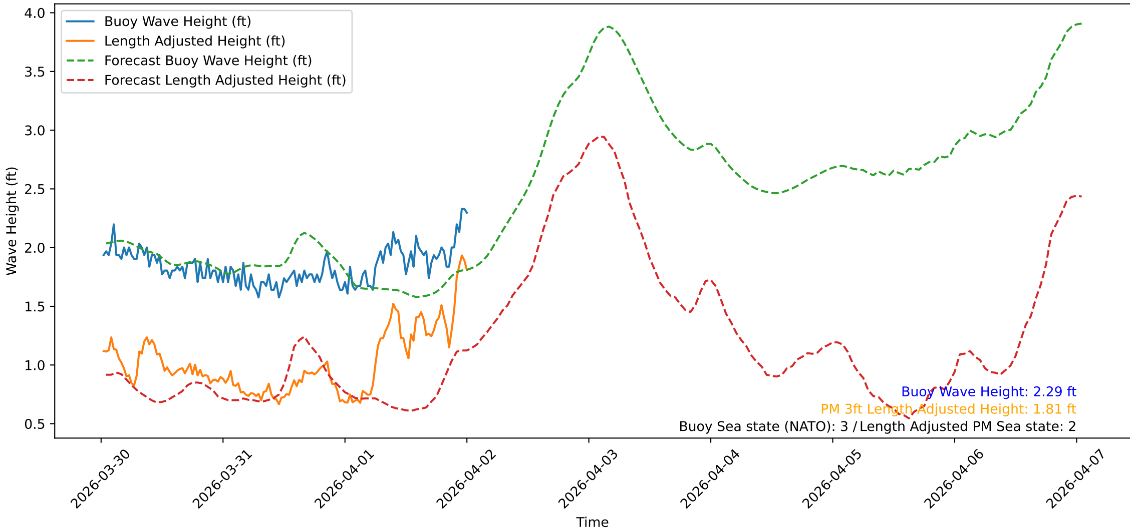
Wave Heights over Time for Oceanside Harbor at 2026-04-02 00:40:31
