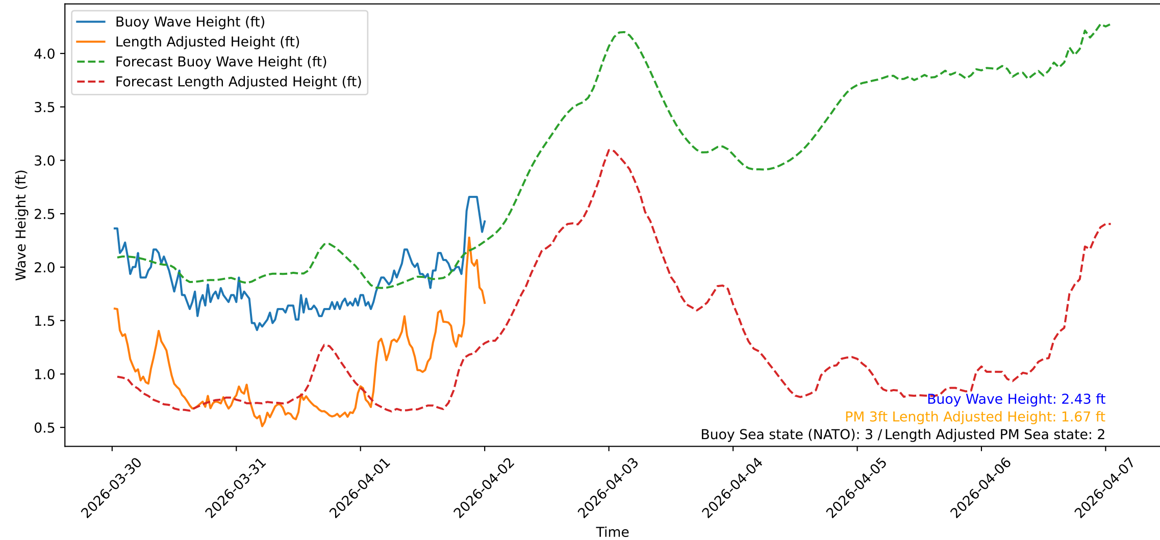
Wave Heights over Time for Green Beach at 2026-04-02 00:41:10
