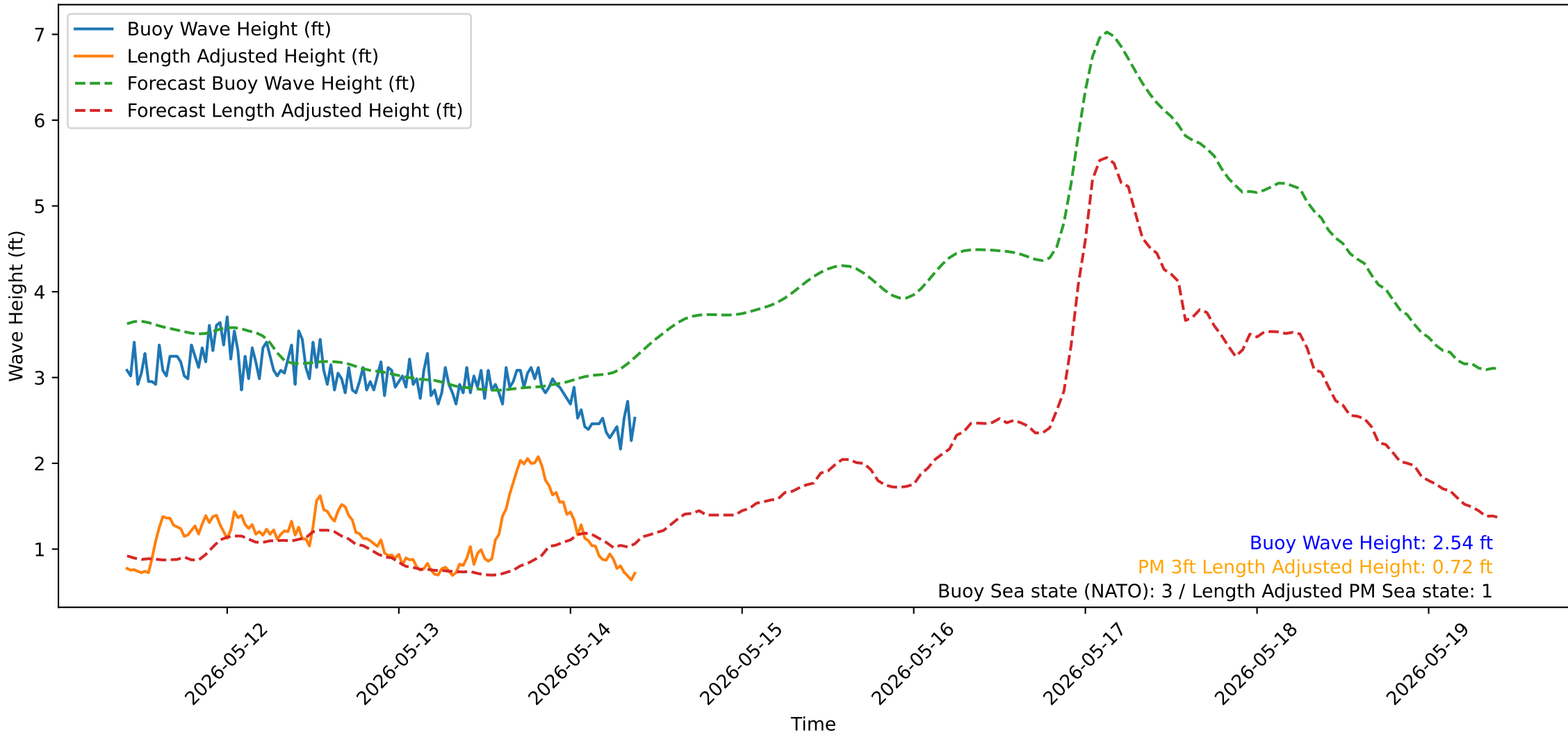
Wave Heights over Time for Oceanside Harbor at 2026-05-14 10:00:32
