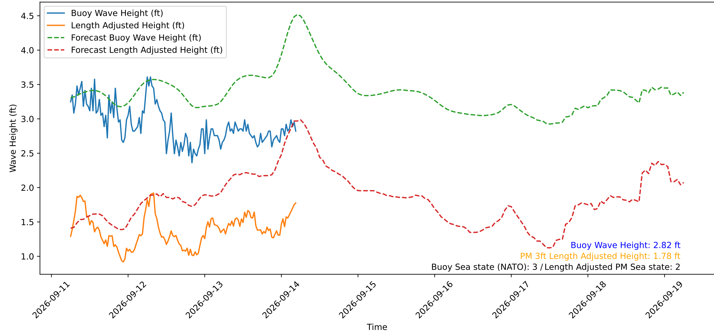
Wave Heights over Time for Green Beach at 2026-09-14 05:31:11
