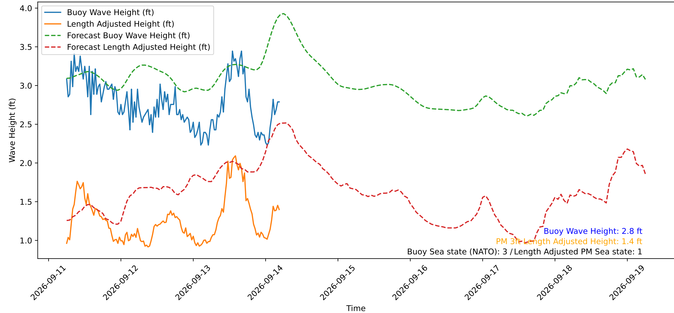
Wave Heights over Time for Red Beach at 2026-09-14 05:30:49
