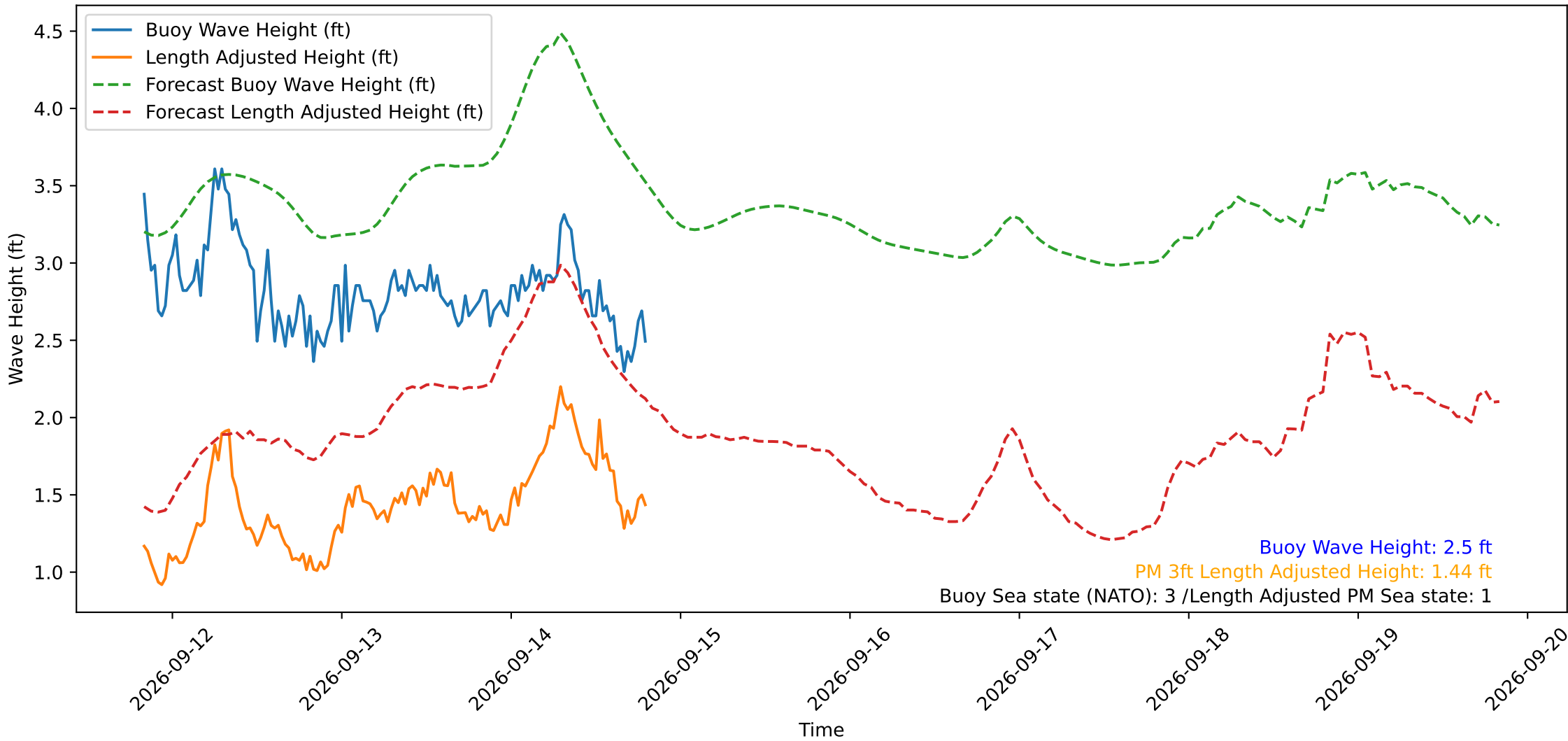
Wave Heights over Time for Green Beach at 2026-09-14 19:51:15
