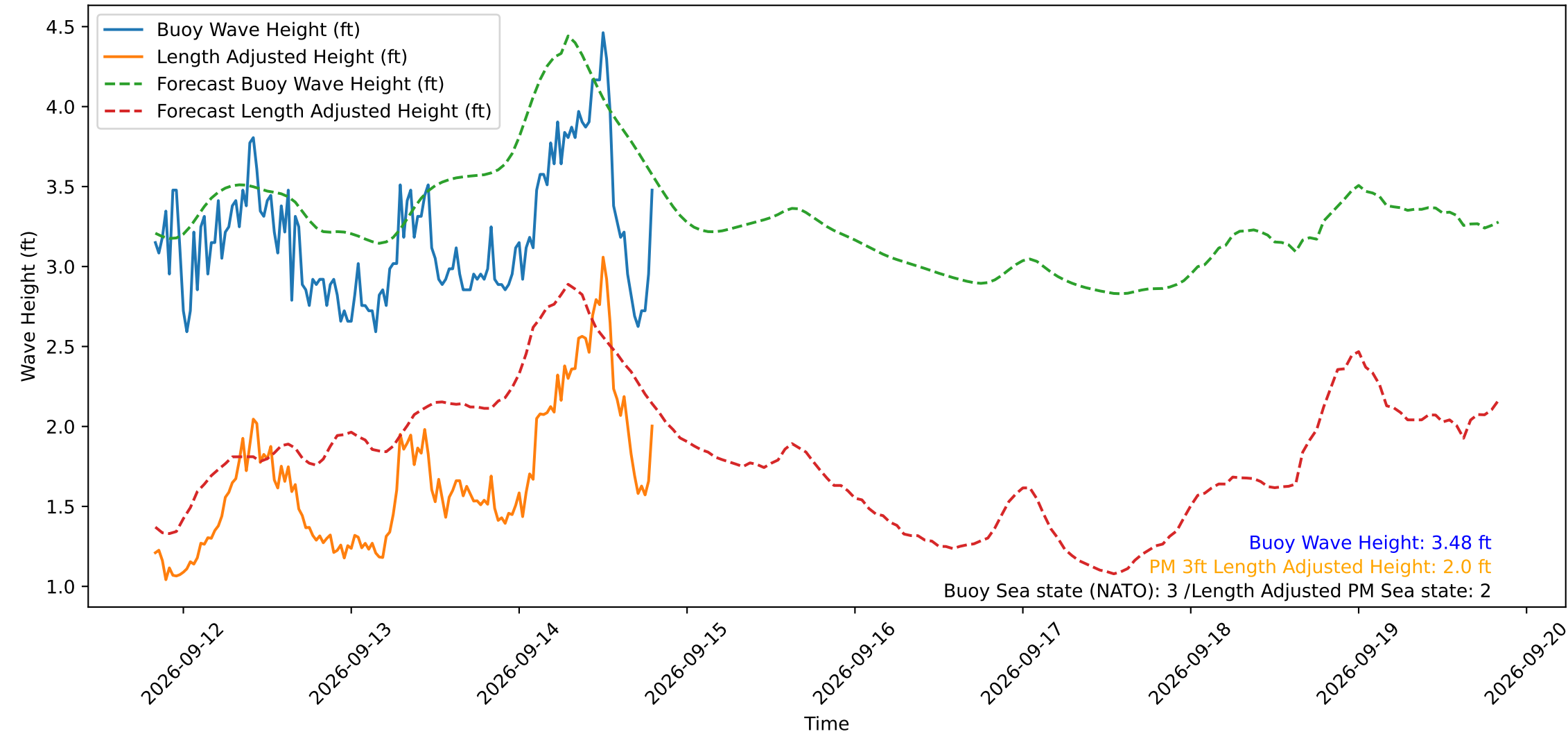
Wave Heights over Time for Oceanside Harbor at 2026-09-14 19:50:30
