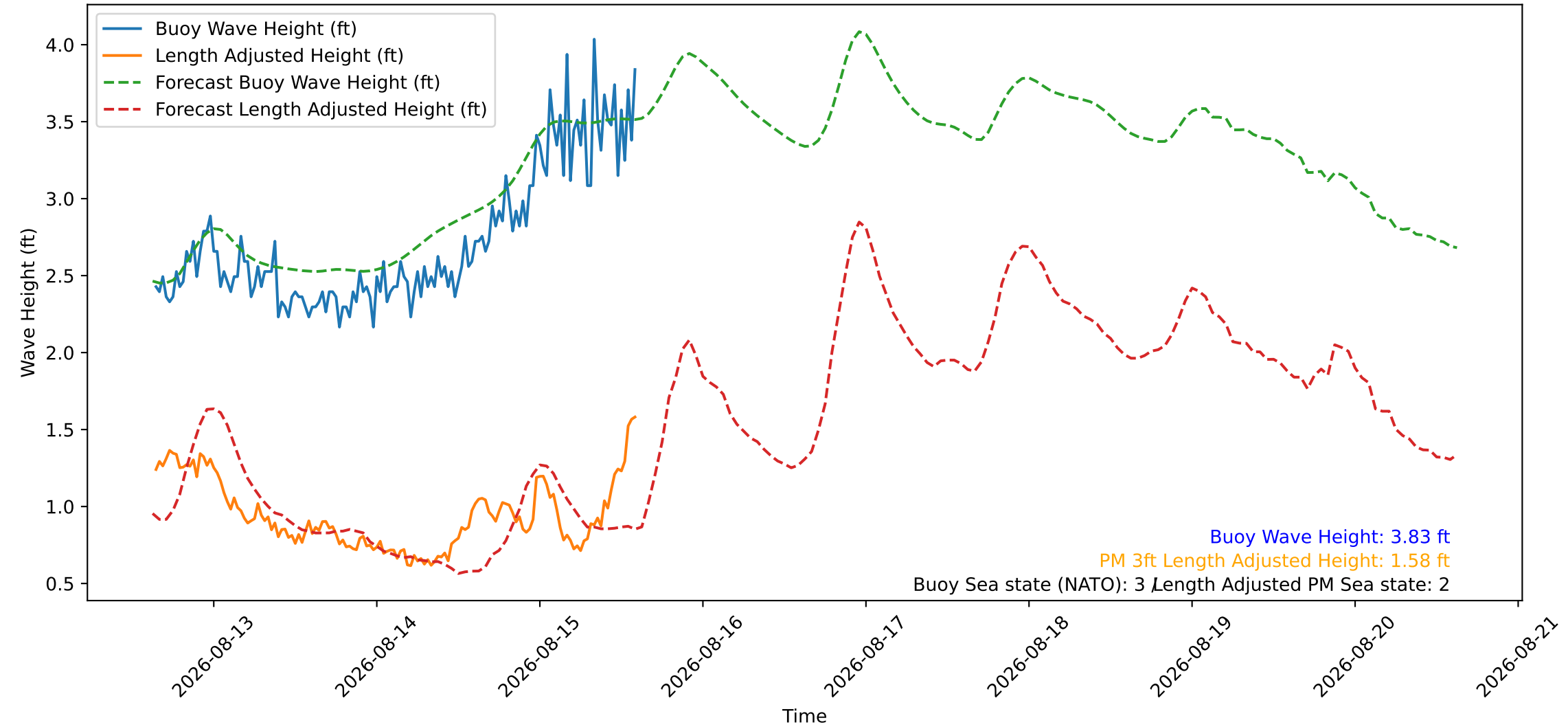
Wave Heights over Time for Red Beach at 2026-08-15 15:00:46
