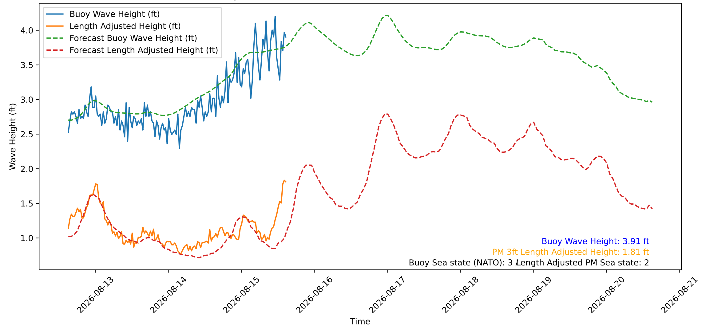
Wave Heights over Time for Oceanside Harbor at 2026-08-15 15:00:27
