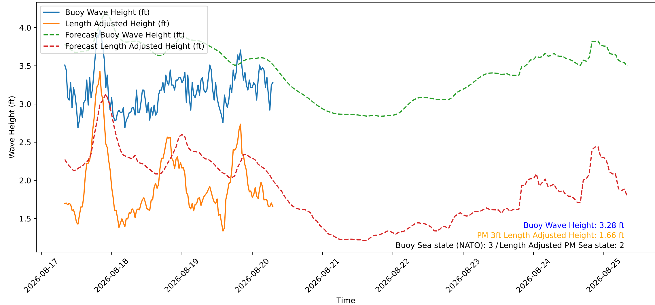
Wave Heights over Time for Green Beach at 2026-08-20 07:41:09
