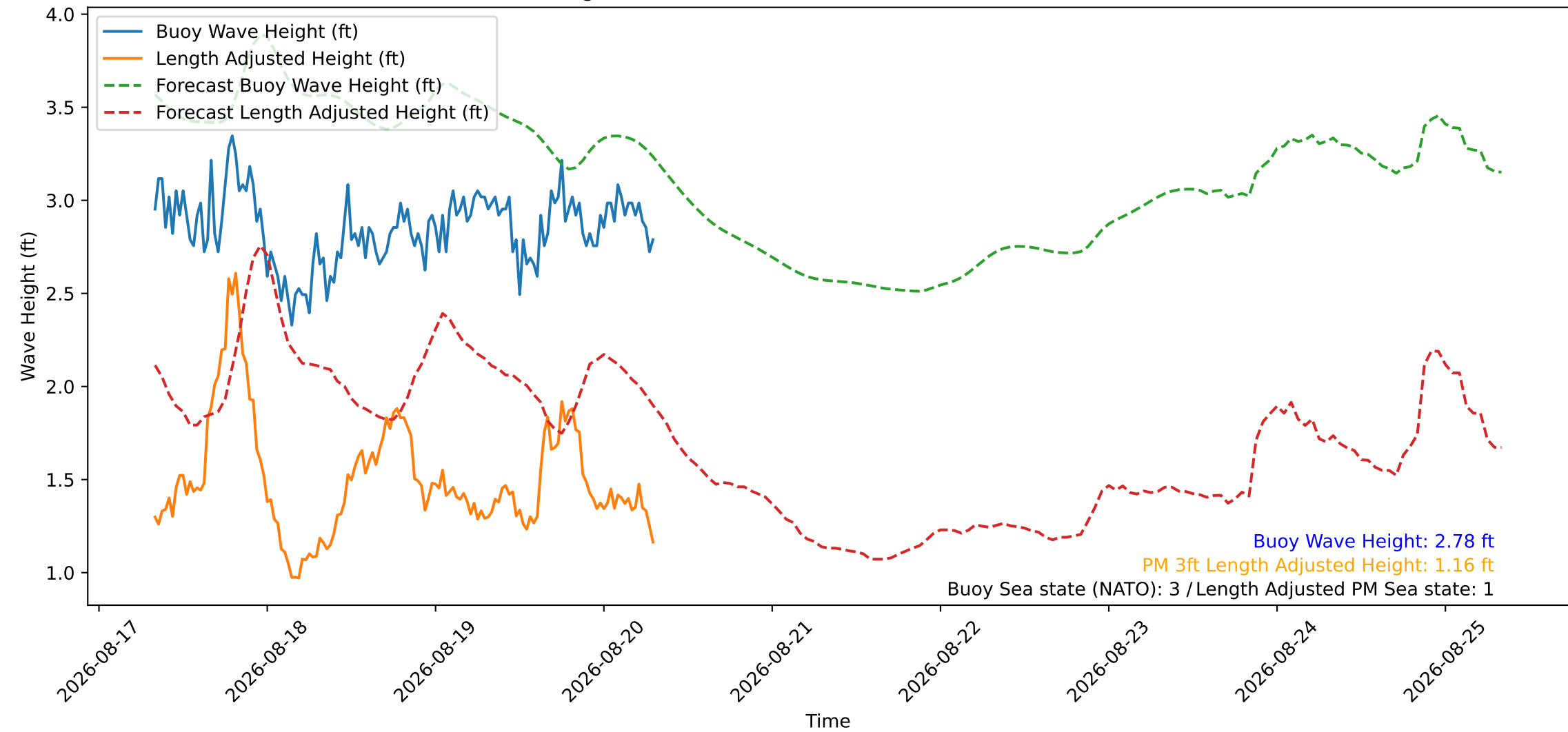
Wave Heights over Time for Red Beach at 2026-08-20 07:40:47
