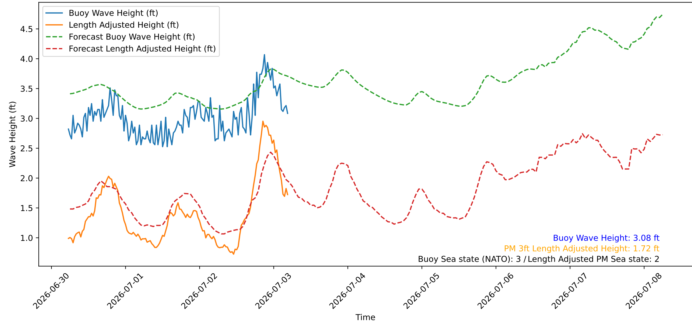
Wave Heights over Time for Green Beach at 2026-07-03 05:31:08
