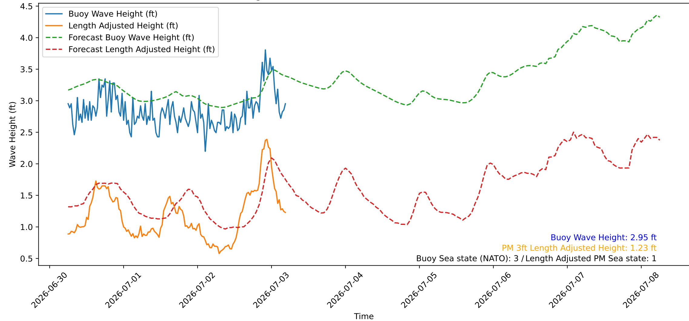
Wave Heights over Time for Red Beach at 2026-07-03 05:30:46
