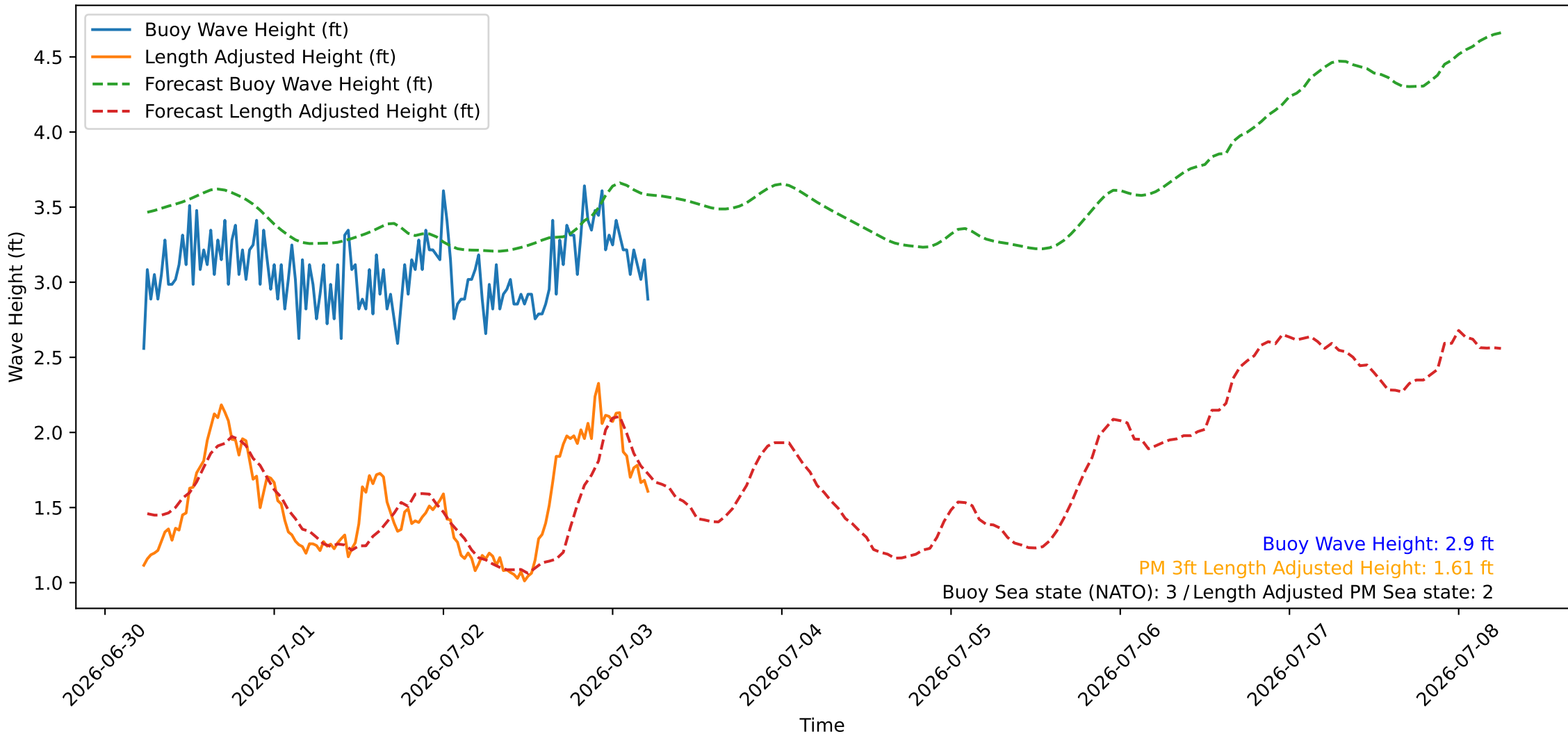
Wave Heights over Time for Oceanside Harbor at 2026-07-03 05:30:26
