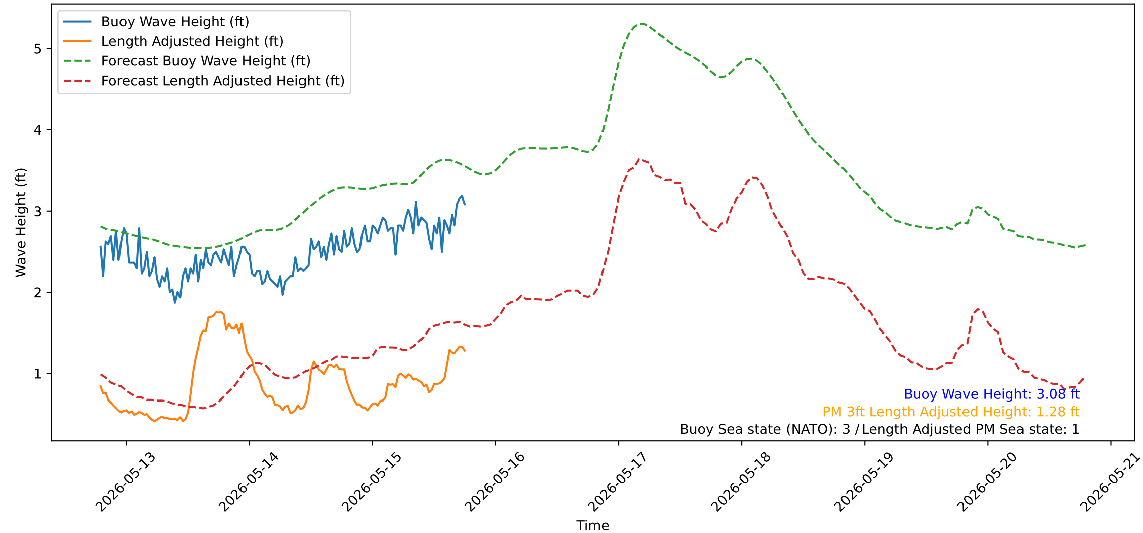
Wave Heights over Time for Red Beach at 2026-05-15 18:40:50
