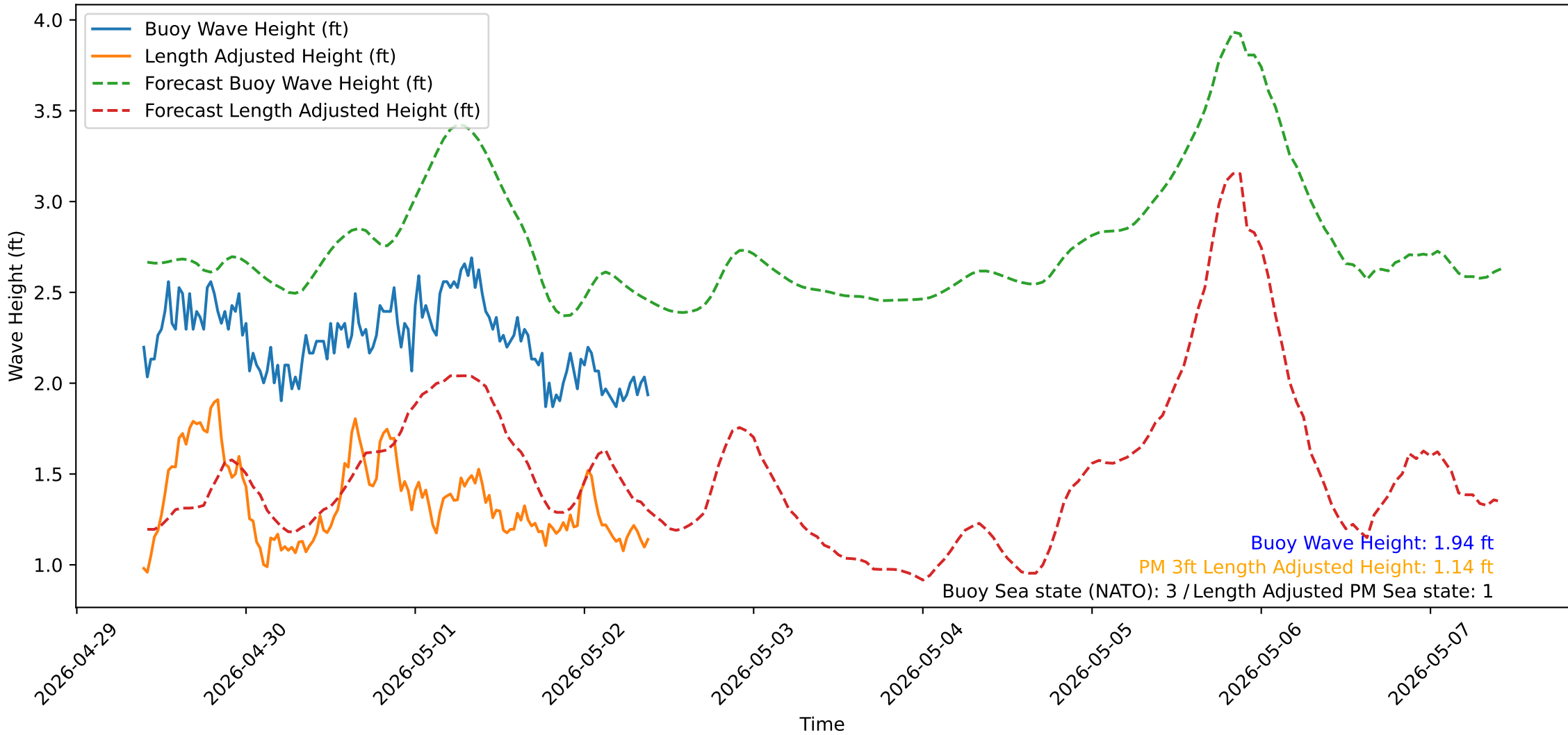
Wave Heights over Time for Oceanside Harbor at 2026-05-02 09:40:32
