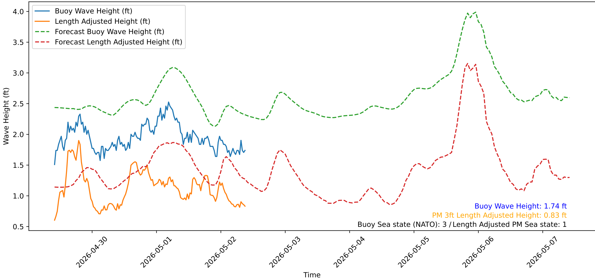
Wave Heights over Time for Red Beach at 2026-05-02 09:40:51
