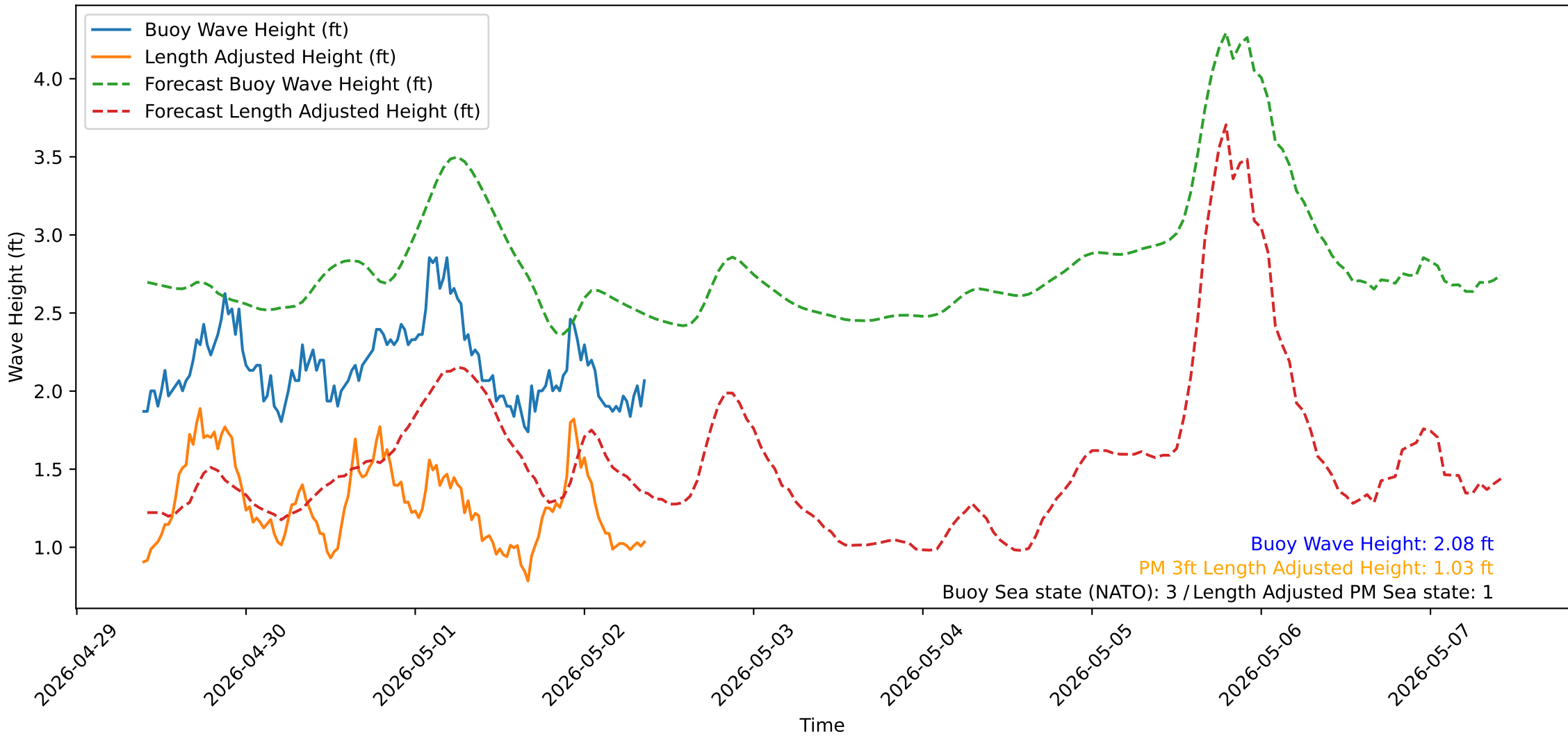
Wave Heights over Time for Green Beach at 2026-05-02 09:41:13
