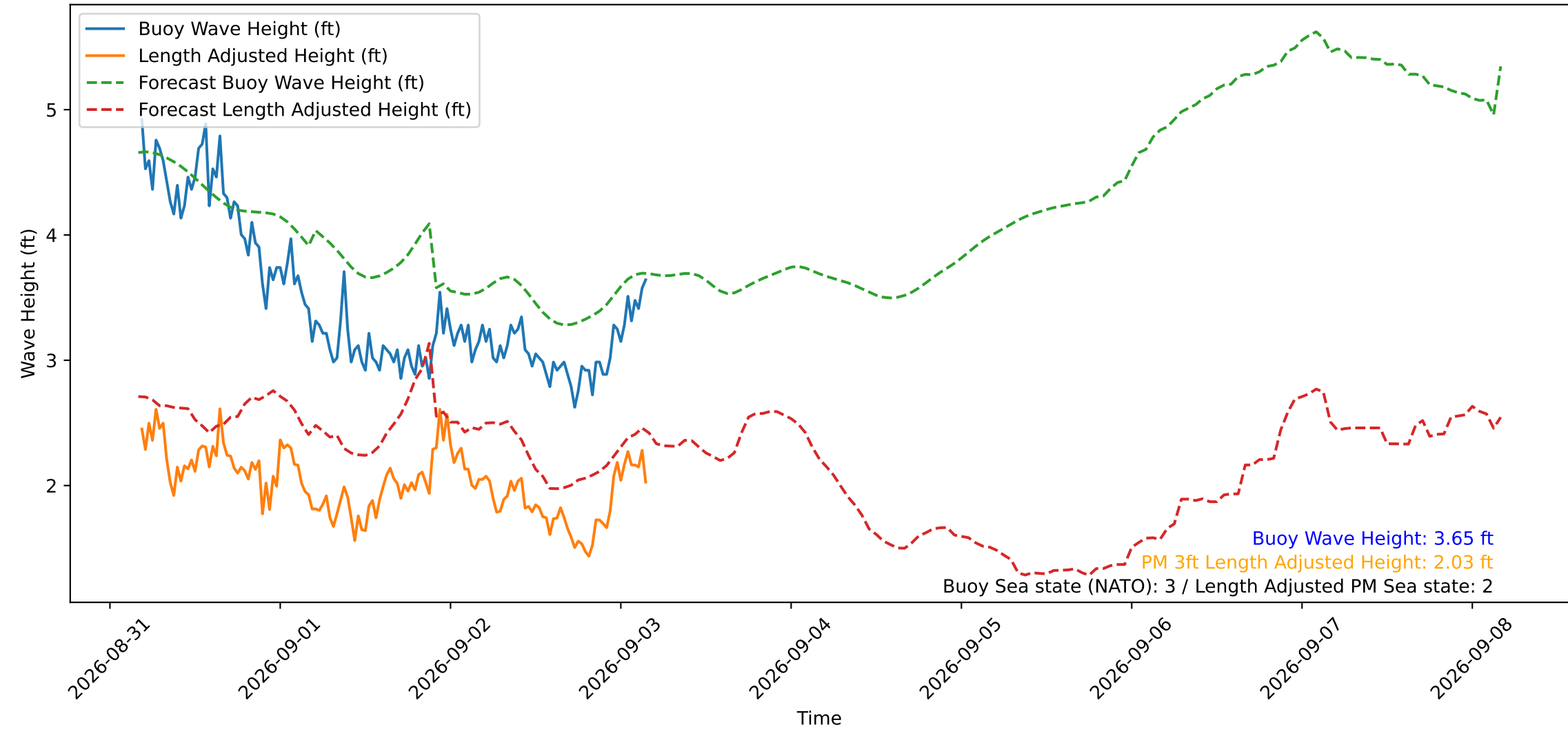
Wave Heights over Time for Oceanside Harbor at 2026-09-03 04:20:29
