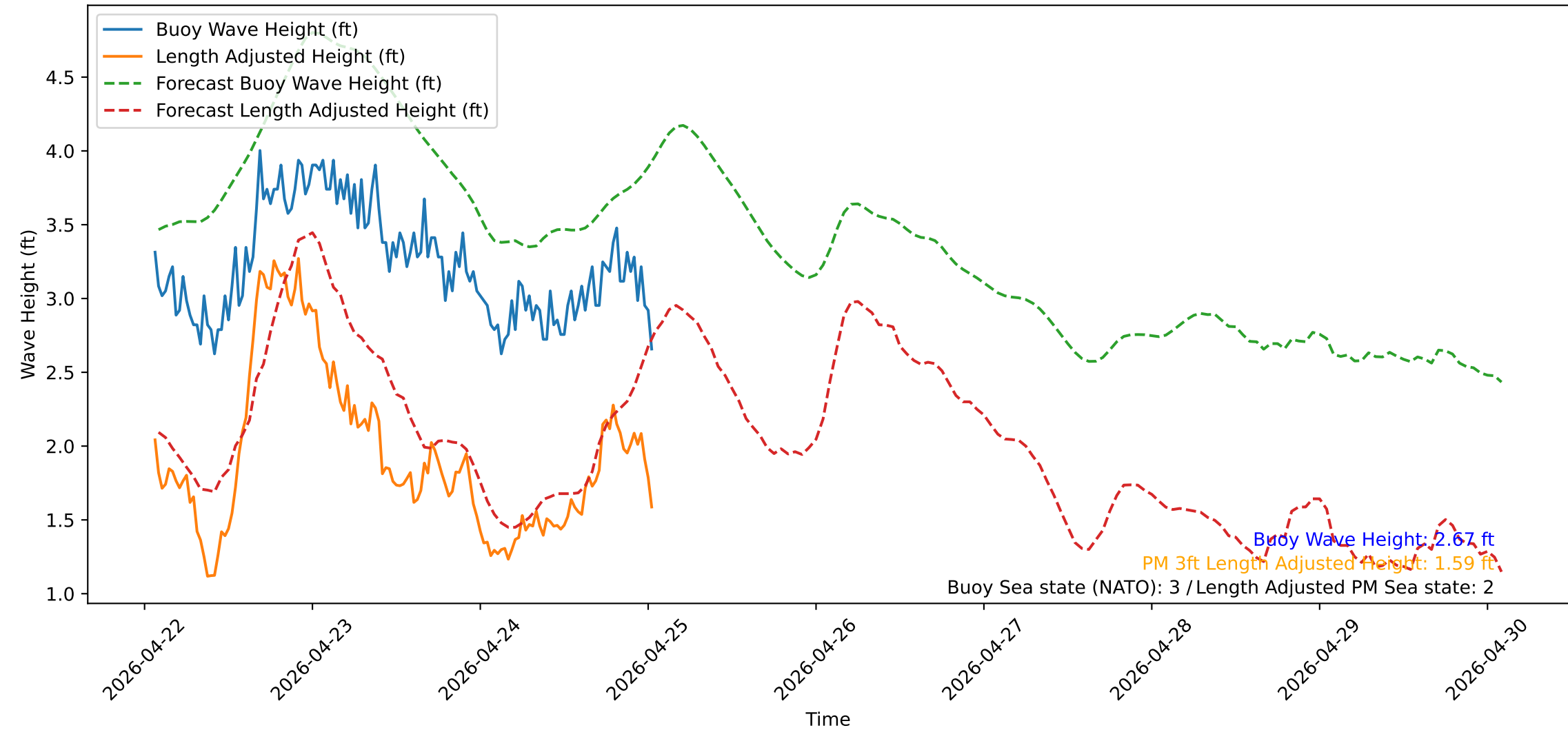
Wave Heights over Time for Green Beach at 2026-04-25 01:41:13
