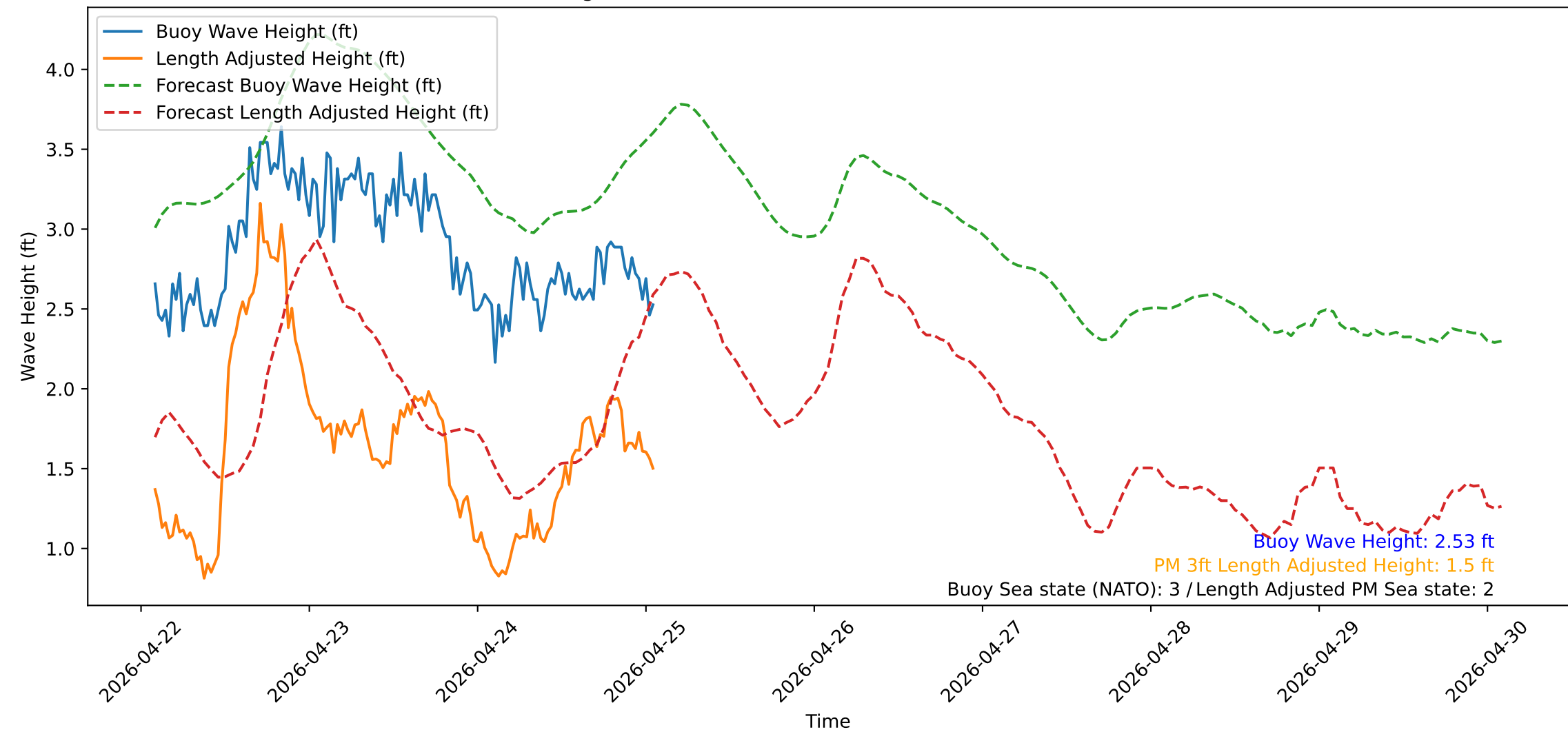
Wave Heights over Time for Red Beach at 2026-04-25 01:40:51
