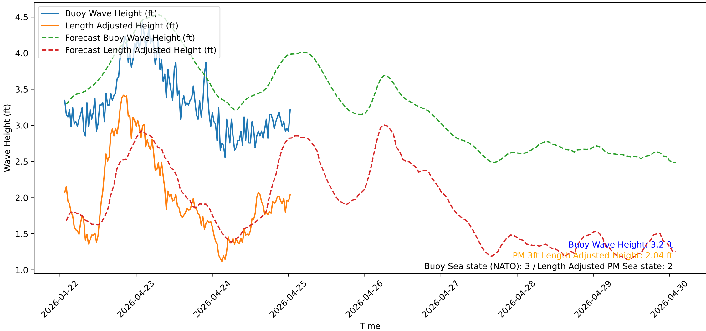
Wave Heights over Time for Oceanside Harbor at 2026-04-25 01:40:31
