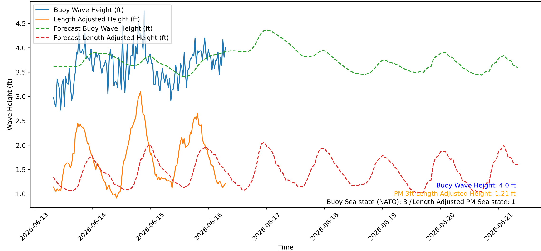
Wave Heights over Time for Red Beach at 2026-06-16 07:50:47
