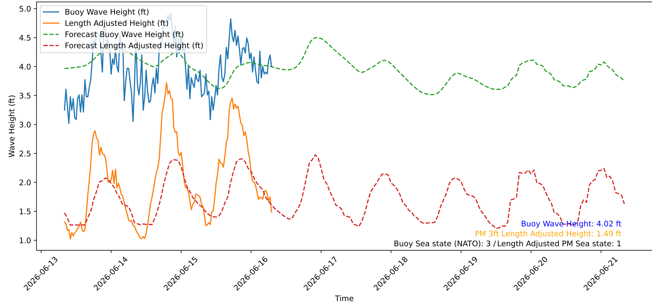
Wave Heights over Time for Green Beach at 2026-06-16 07:51:10
