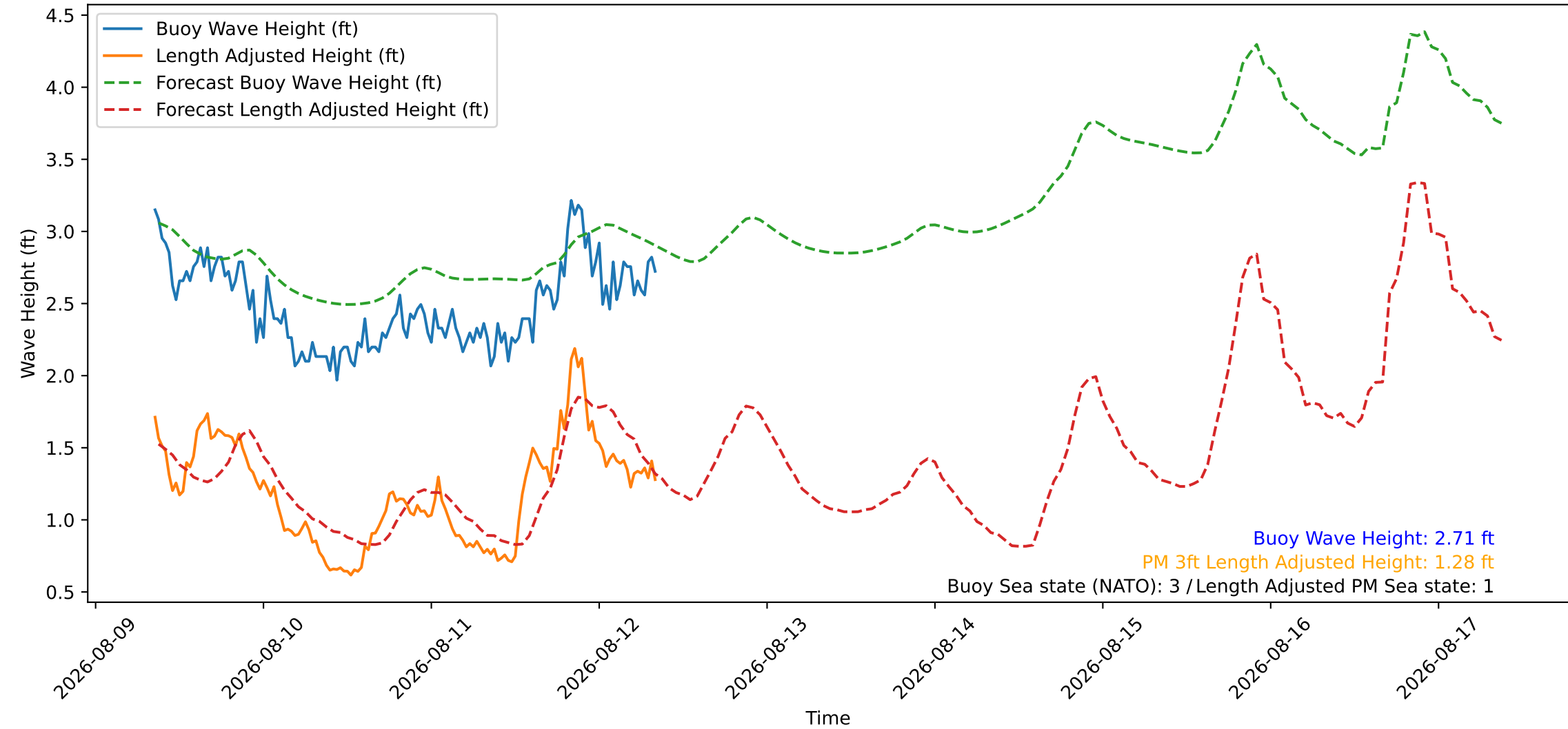
Wave Heights over Time for Green Beach at 2026-08-12 08:41:07
