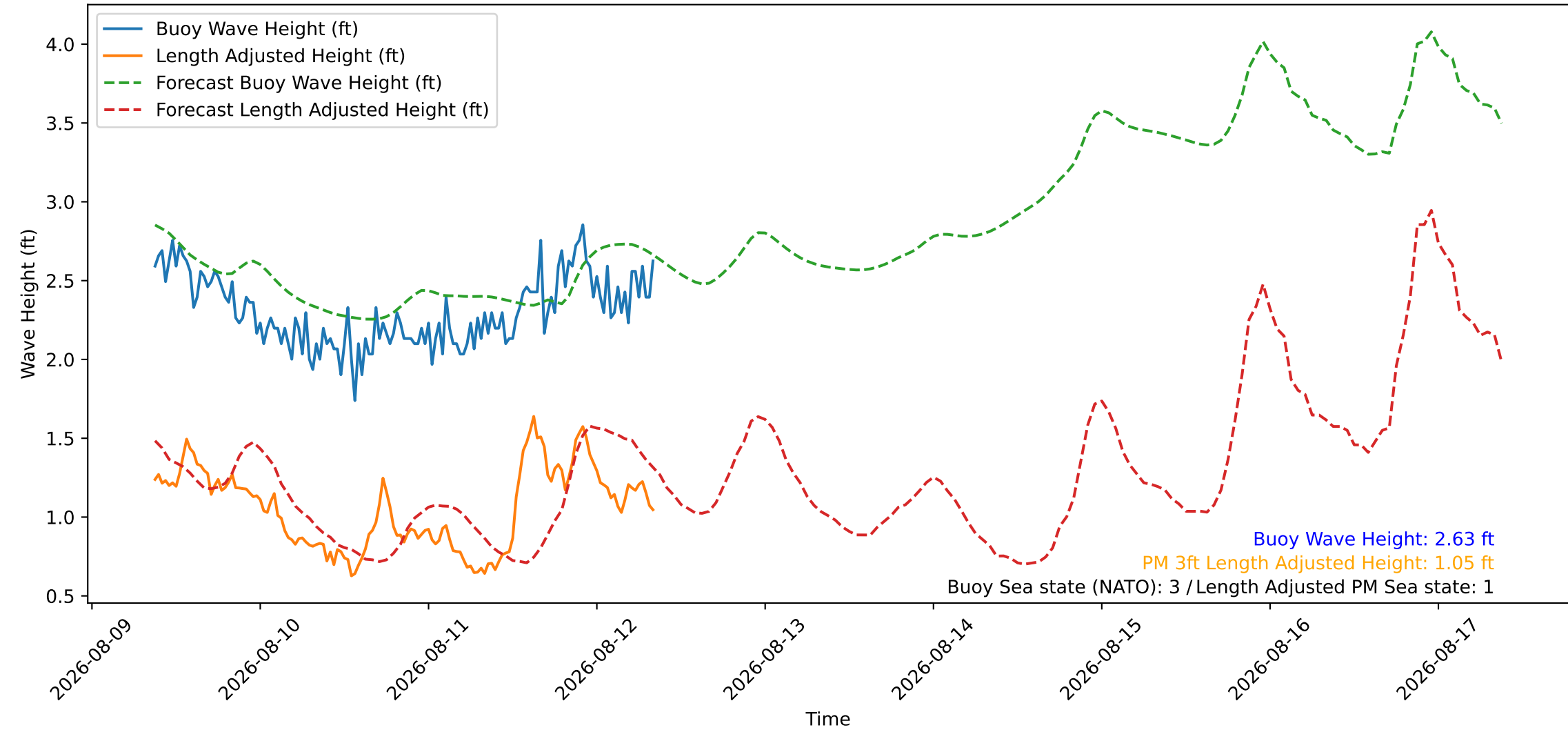
Wave Heights over Time for Red Beach at 2026-08-12 08:40:45
