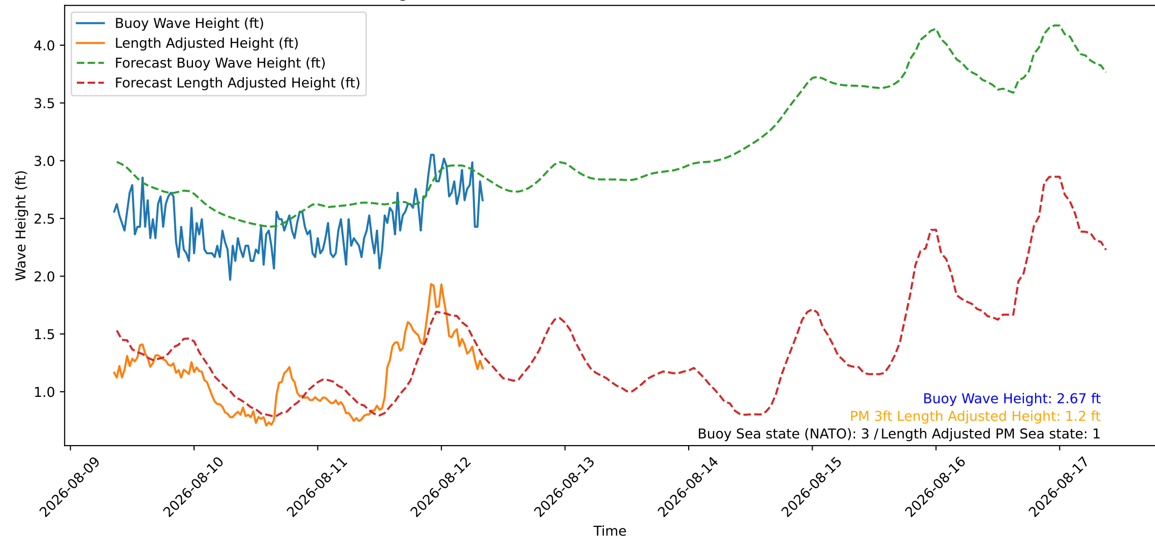
Wave Heights over Time for Oceanside Harbor at 2026-08-12 08:40:26
