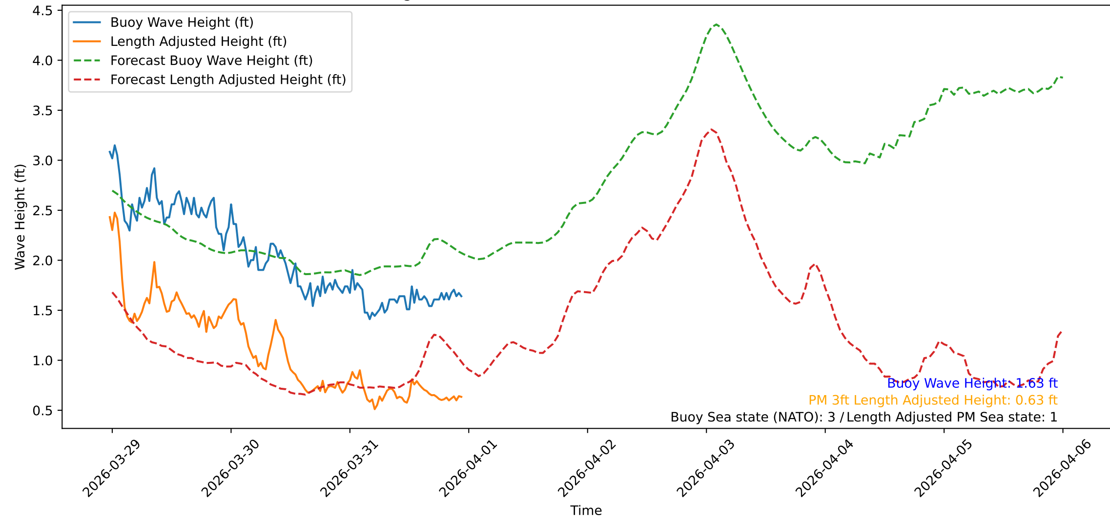
Wave Heights over Time for Green Beach at 2026-03-31 23:31:10
