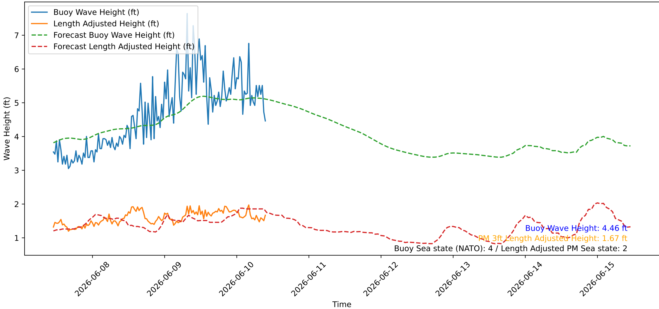
Wave Heights over Time for Red Beach at 2026-06-10 10:50:48
