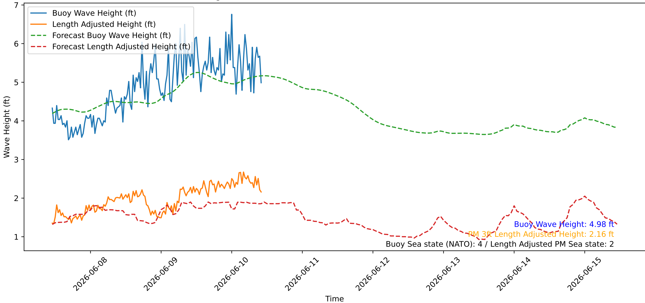
Wave Heights over Time for Oceanside Harbor at 2026-06-10 10:50:26
