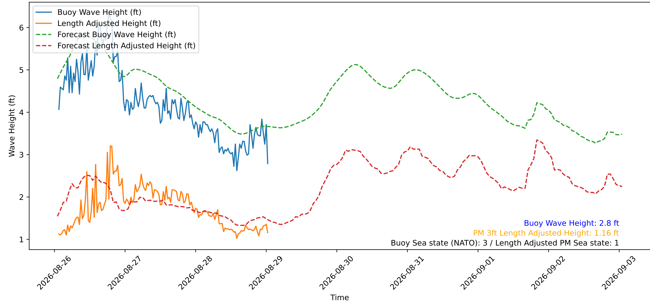
Wave Heights over Time for Green Beach at 2026-08-29 01:11:13
