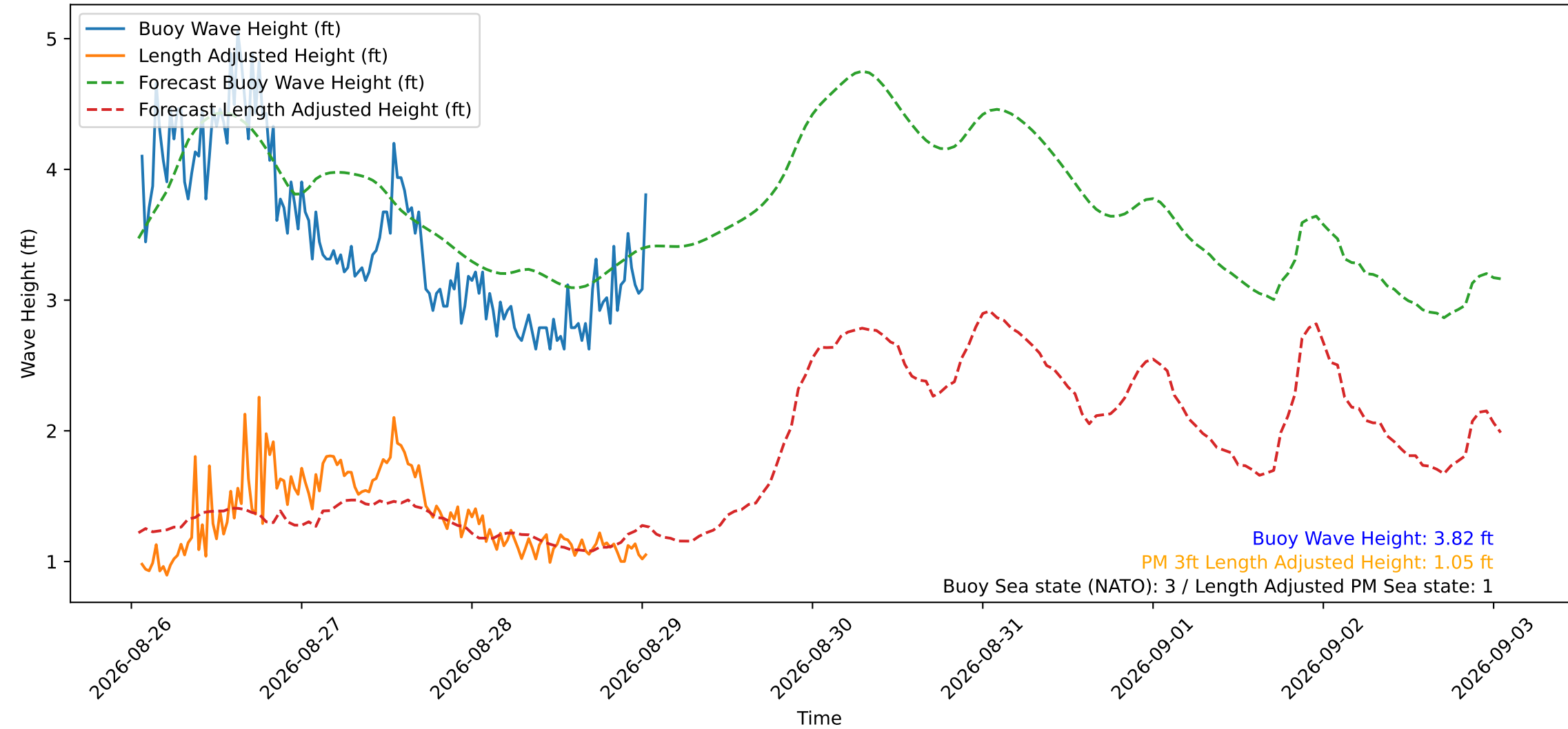
Wave Heights over Time for Red Beach at 2026-08-29 01:10:50
