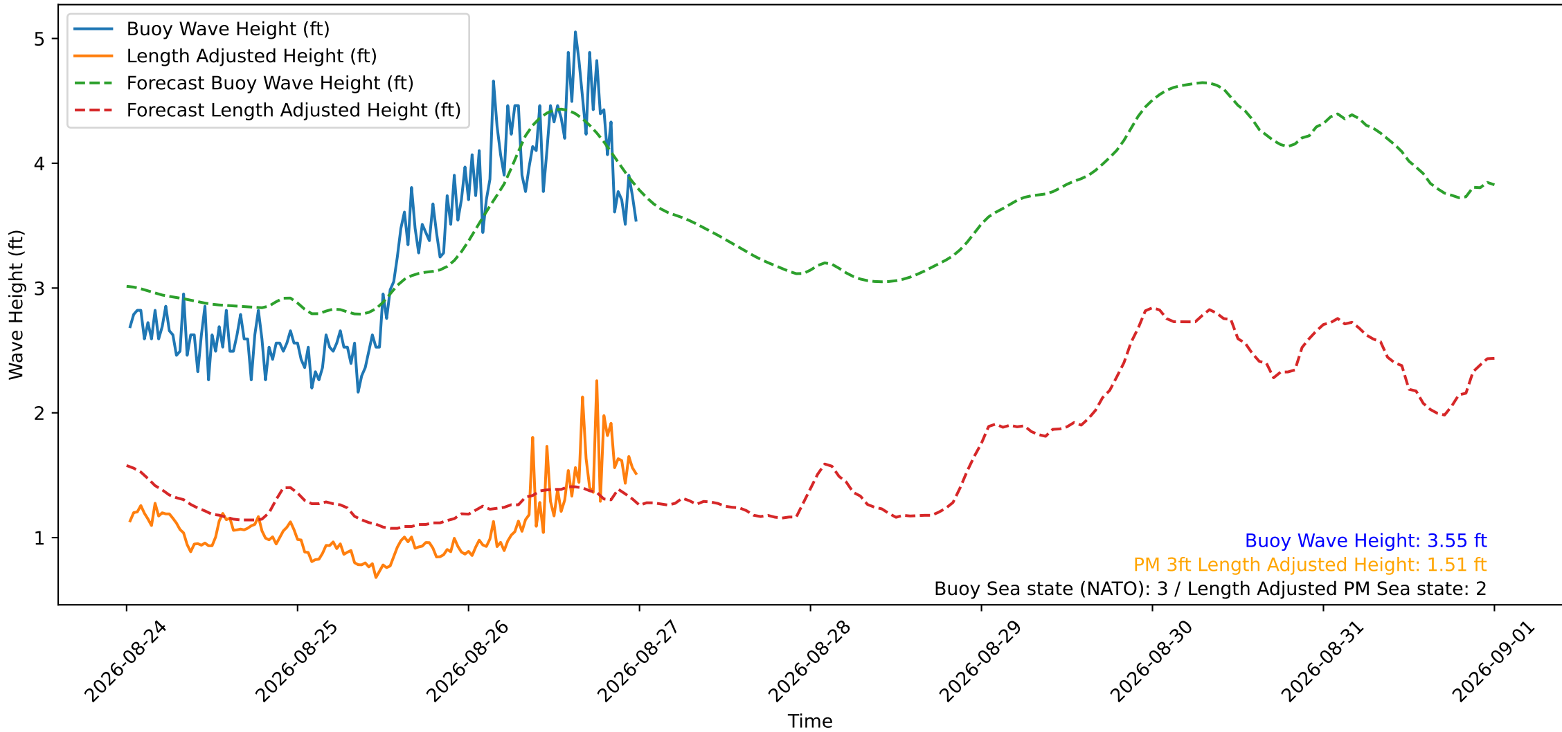
Wave Heights over Time for Red Beach at 2026-08-27 00:20:50
