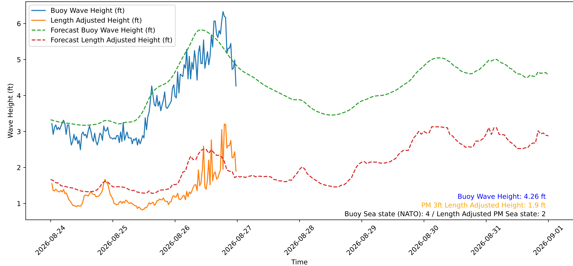
Wave Heights over Time for Green Beach at 2026-08-27 00:21:14
