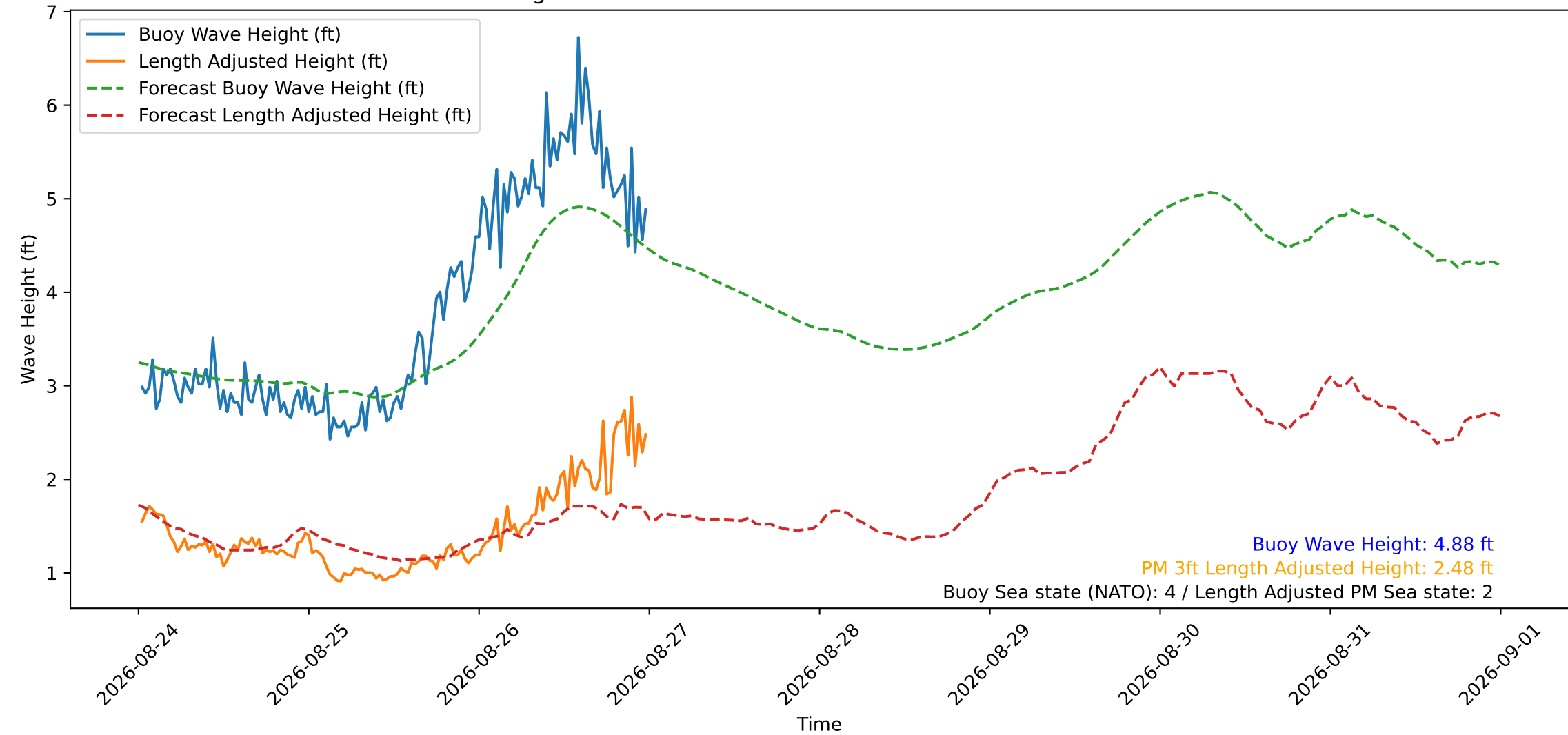
Wave Heights over Time for Oceanside Harbor at 2026-08-27 00:20:29
