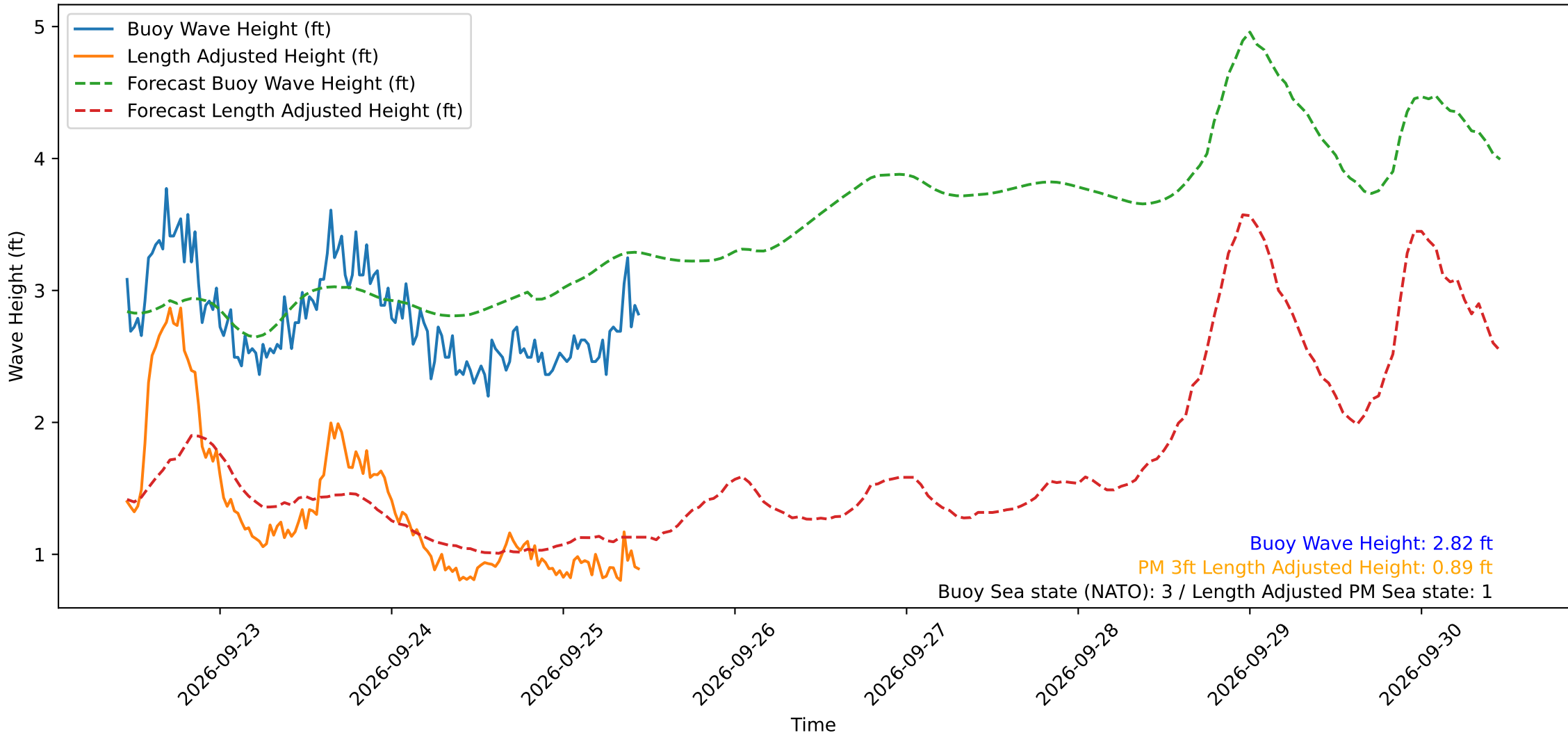
Wave Heights over Time for Oceanside Harbor at 2026-09-25 11:00:29
