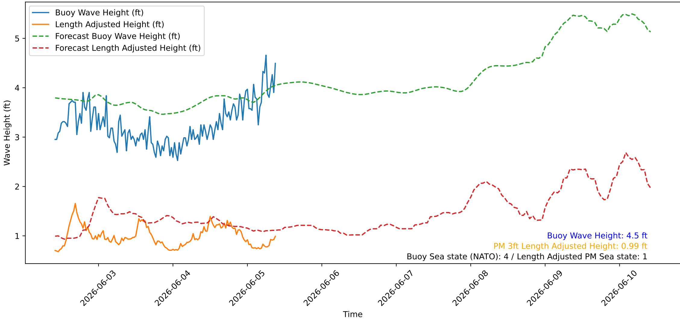
Wave Heights over Time for Red Beach at 2026-06-05 09:40:46
