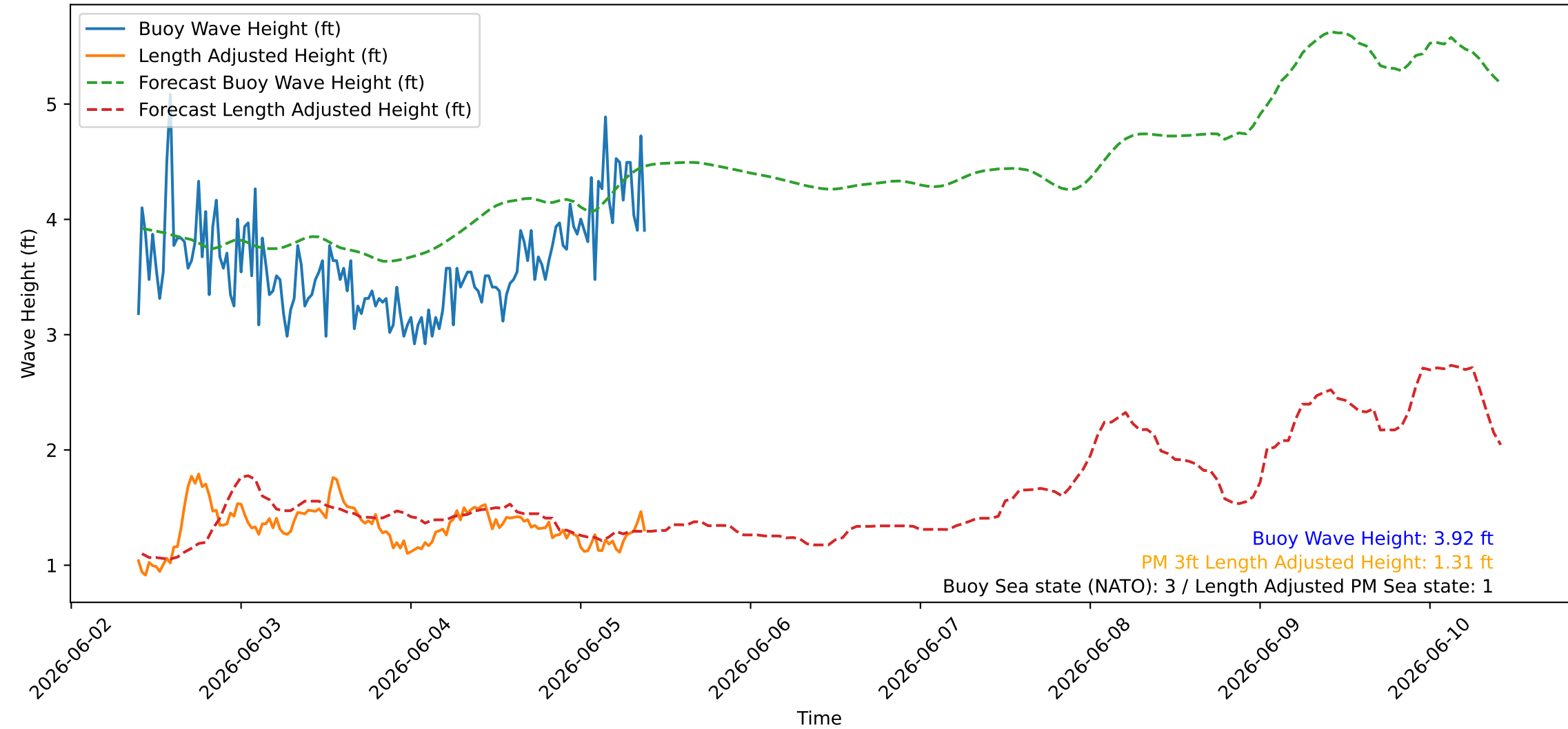
Wave Heights over Time for Oceanside Harbor at 2026-06-05 09:40:25
