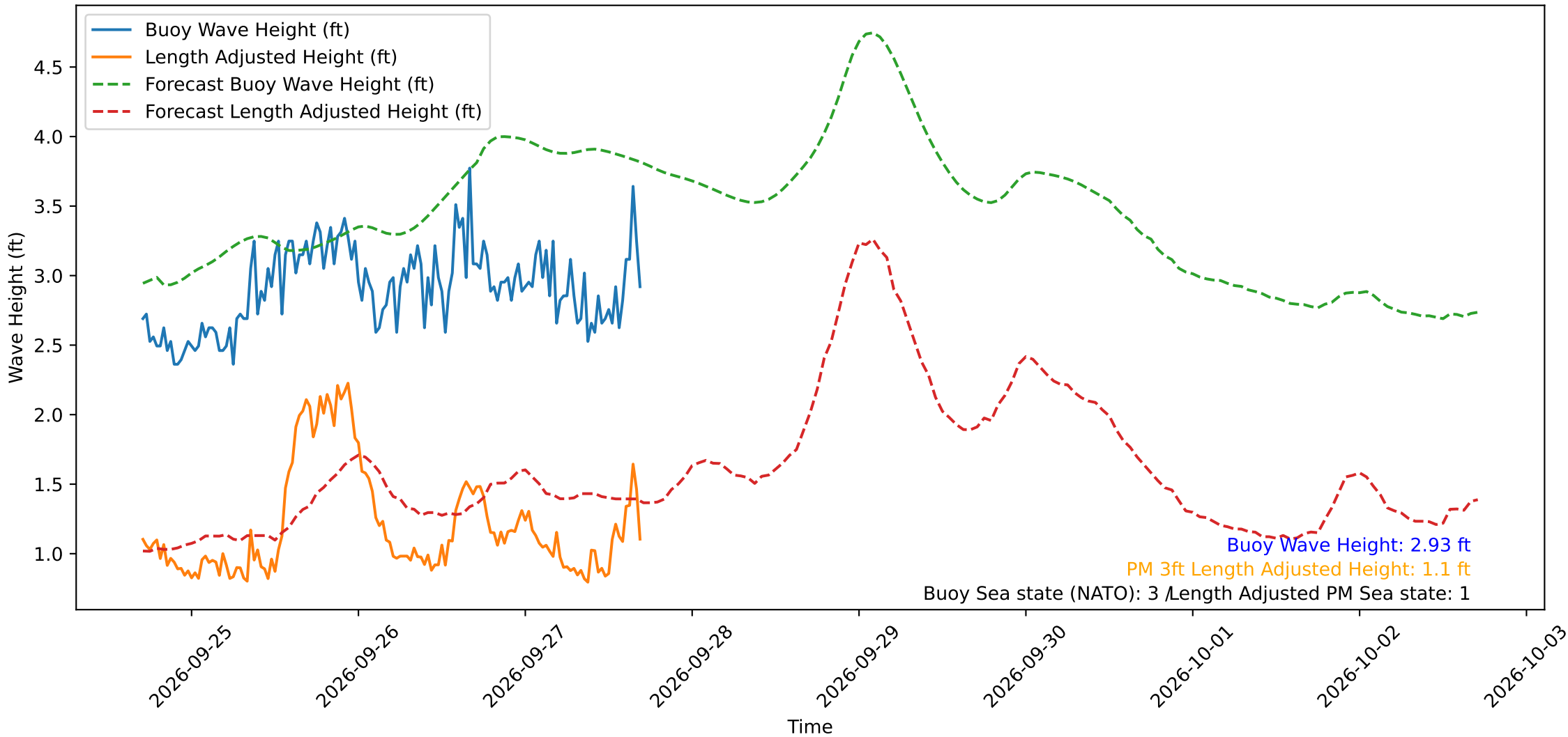
Wave Heights over Time for Oceanside Harbor at 2026-09-27 17:10:30
