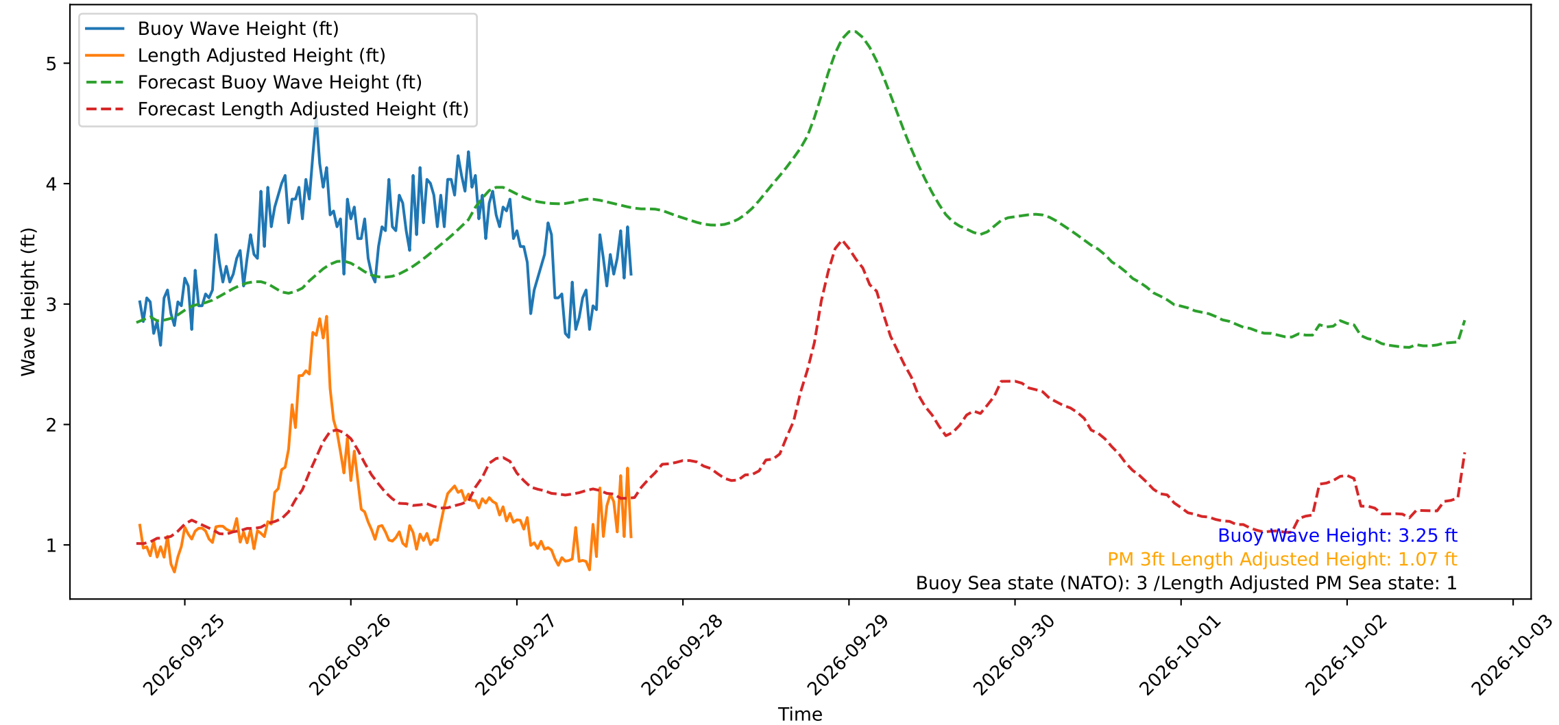
Wave Heights over Time for Green Beach at 2026-09-27 17:11:12
