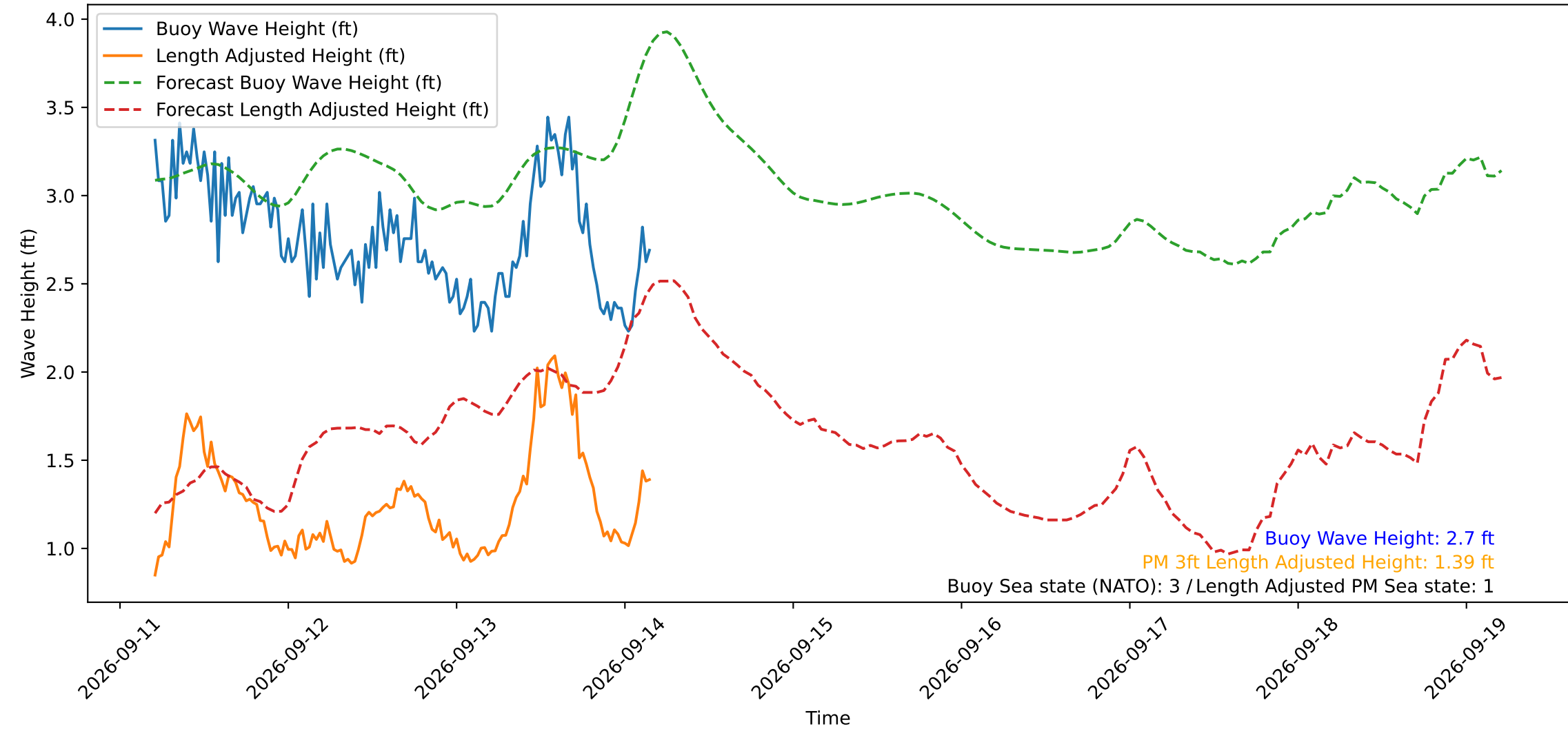
Wave Heights over Time for Red Beach at 2026-09-14 04:30:49
