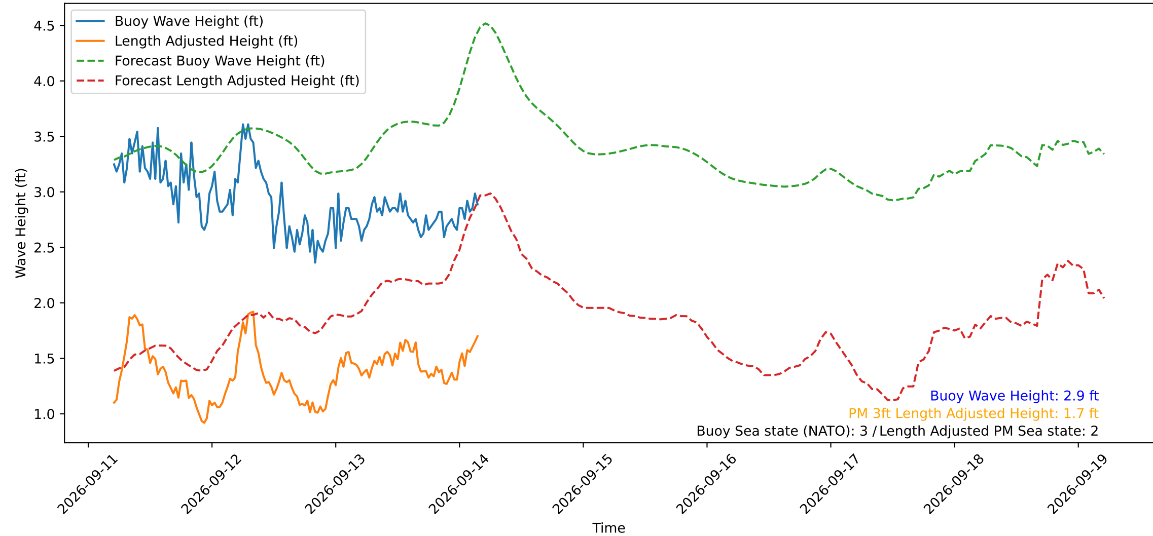
Wave Heights over Time for Green Beach at 2026-09-14 04:31:11
