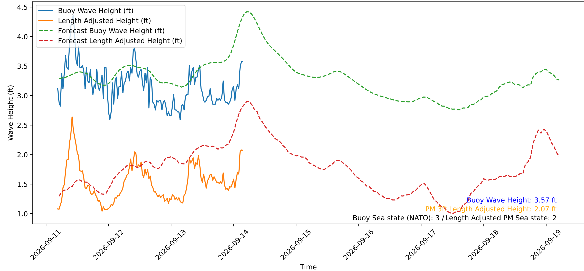
Wave Heights over Time for Oceanside Harbor at 2026-09-14 04:30:30
