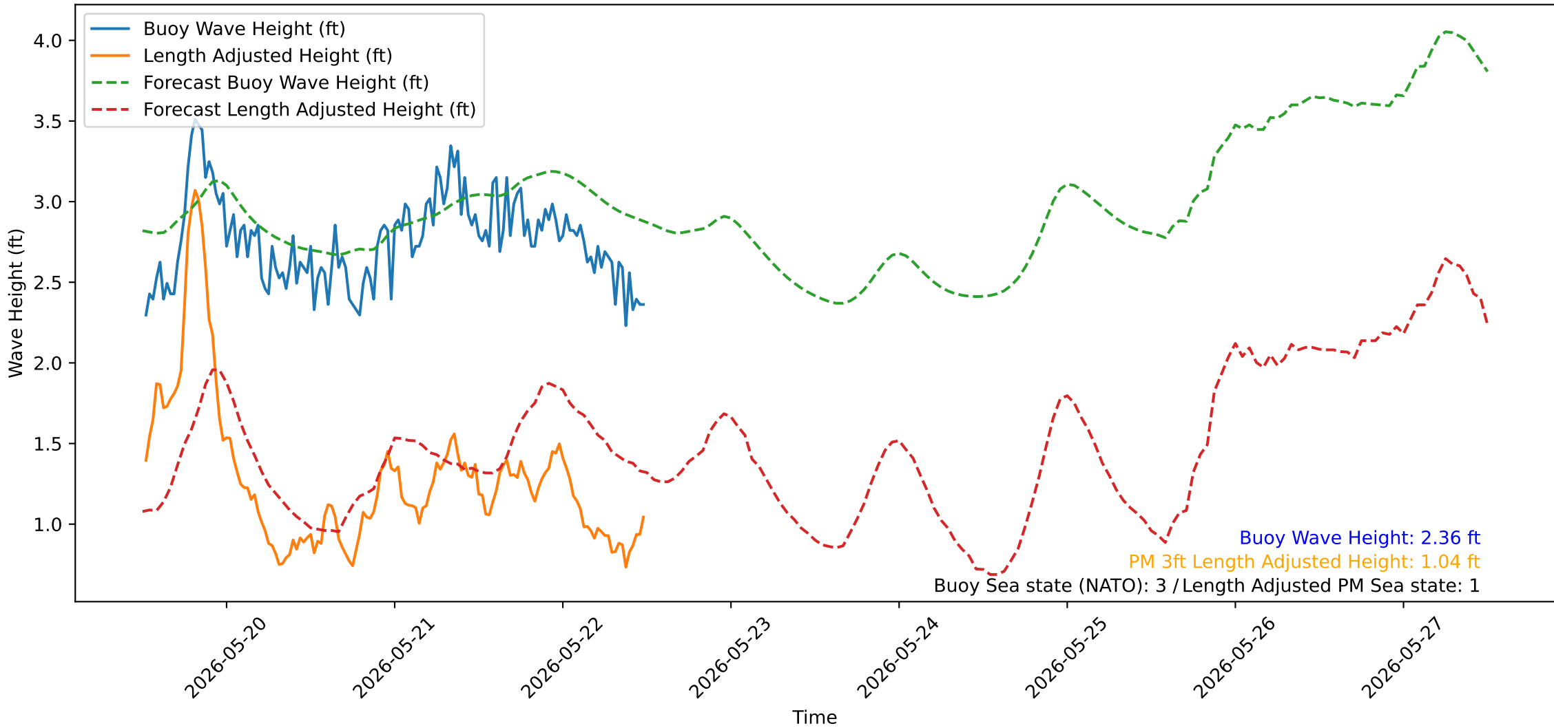
Wave Heights over Time for Red Beach at 2026-05-22 12:20:52
