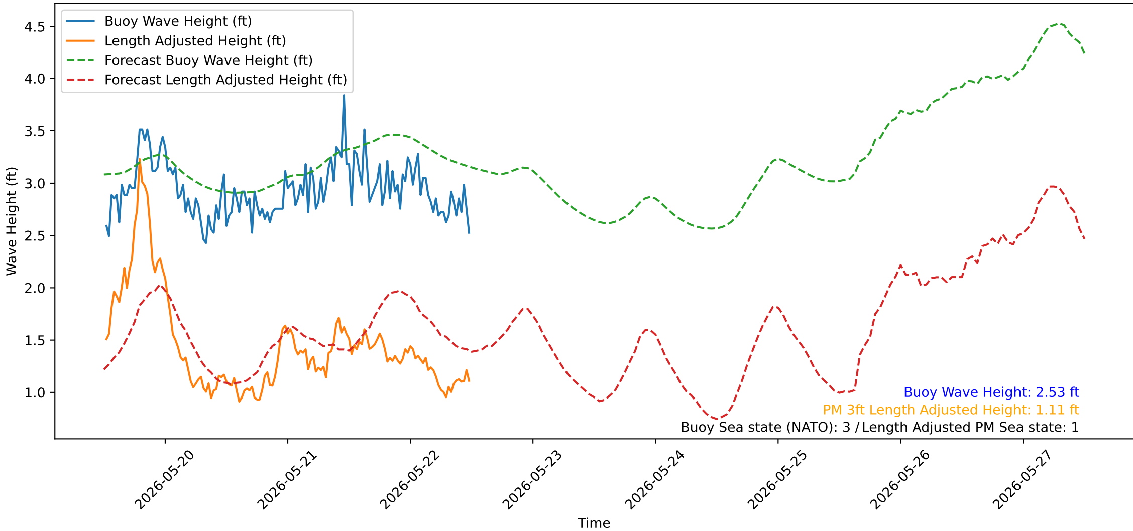
Wave Heights over Time for Oceanside Harbor at 2026-05-22 12:20:32
