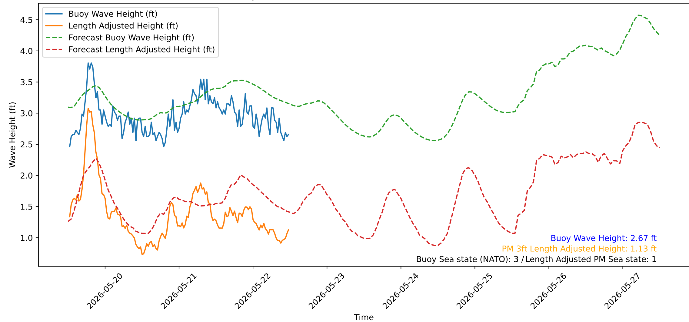
Wave Heights over Time for Green Beach at 2026-05-22 12:21:15
