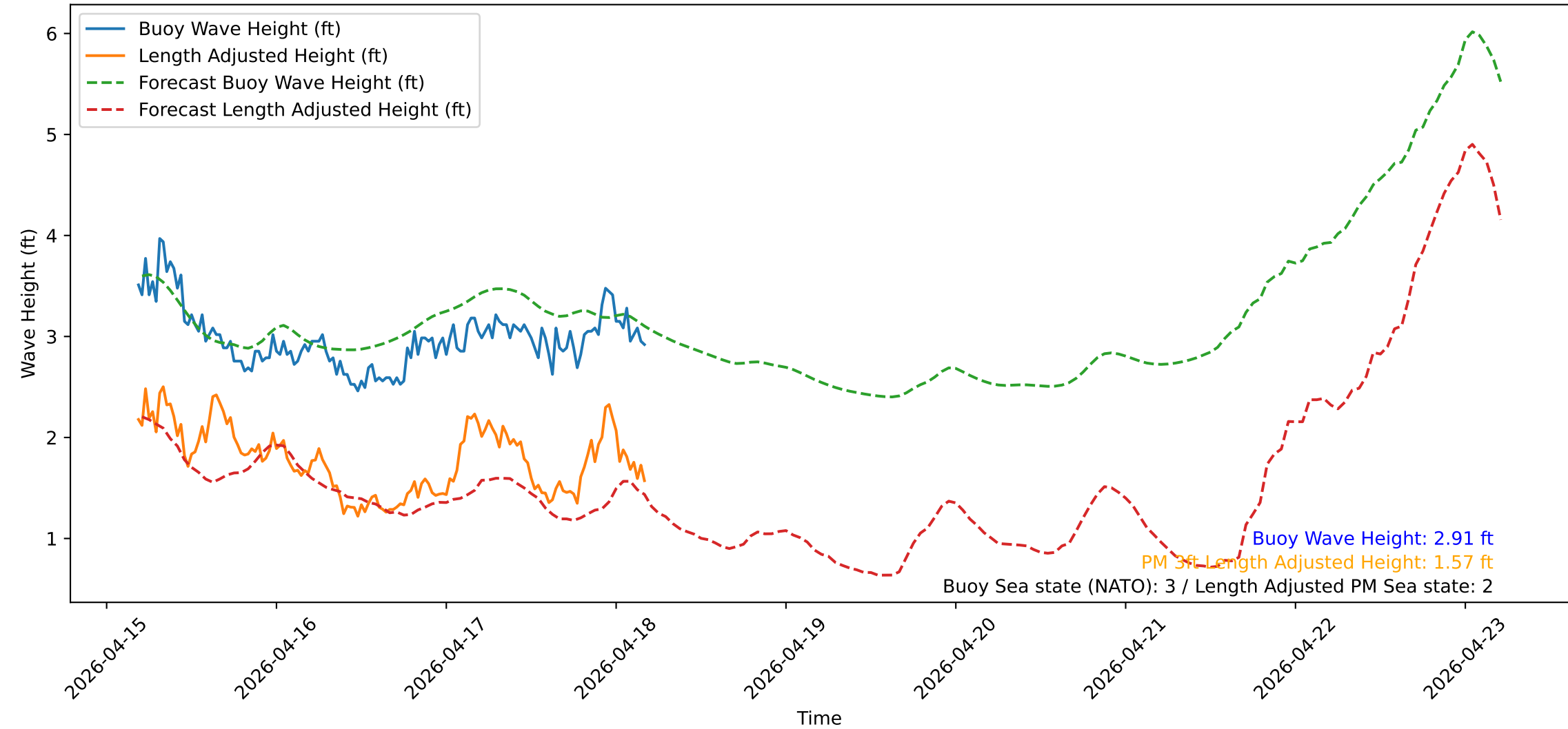
Wave Heights over Time for Green Beach at 2026-04-18 04:41:13
