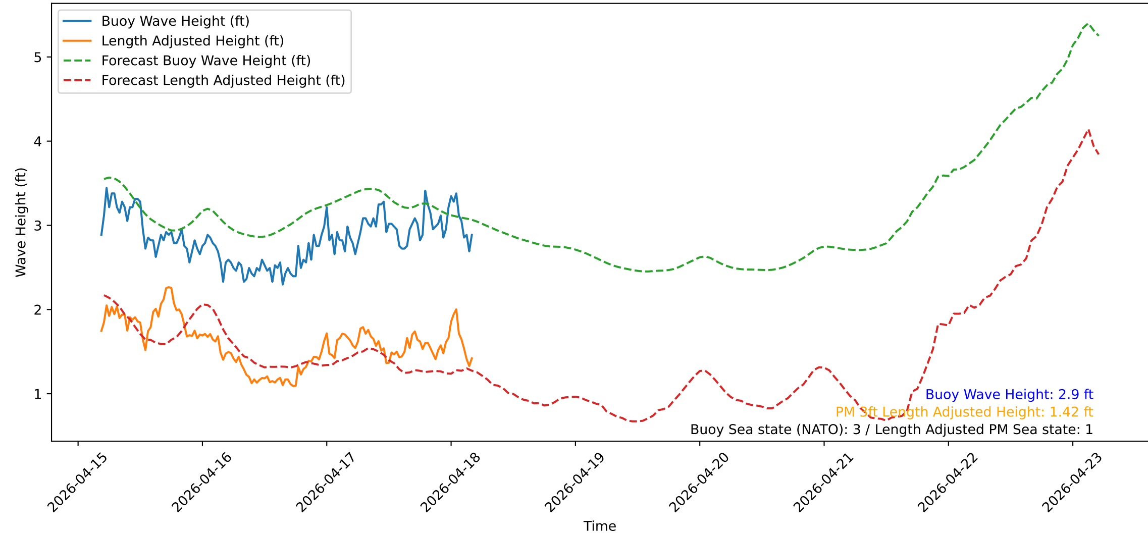
Wave Heights over Time for Oceanside Harbor at 2026-04-18 04:40:32
