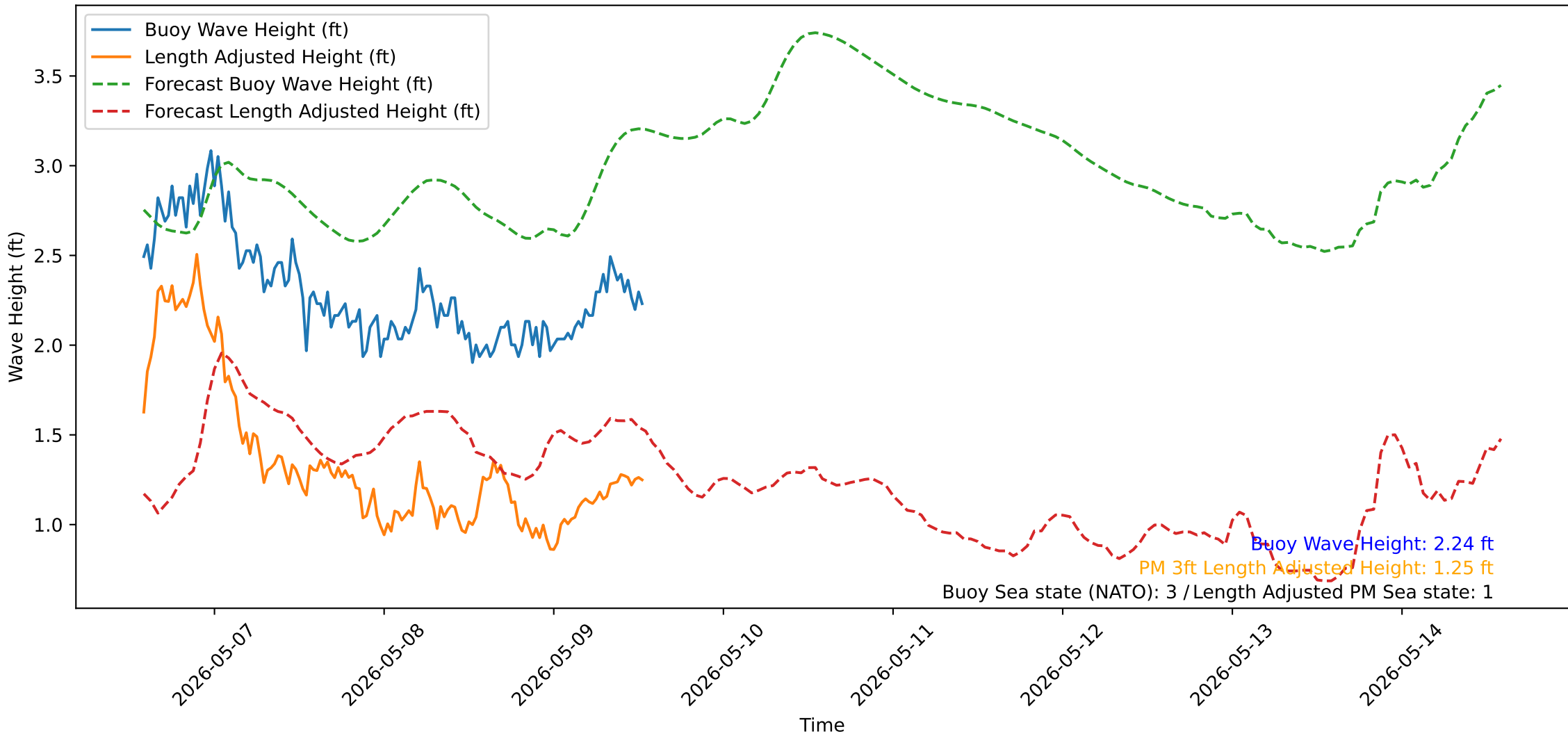
Wave Heights over Time for Red Beach at 2026-05-09 13:30:50
