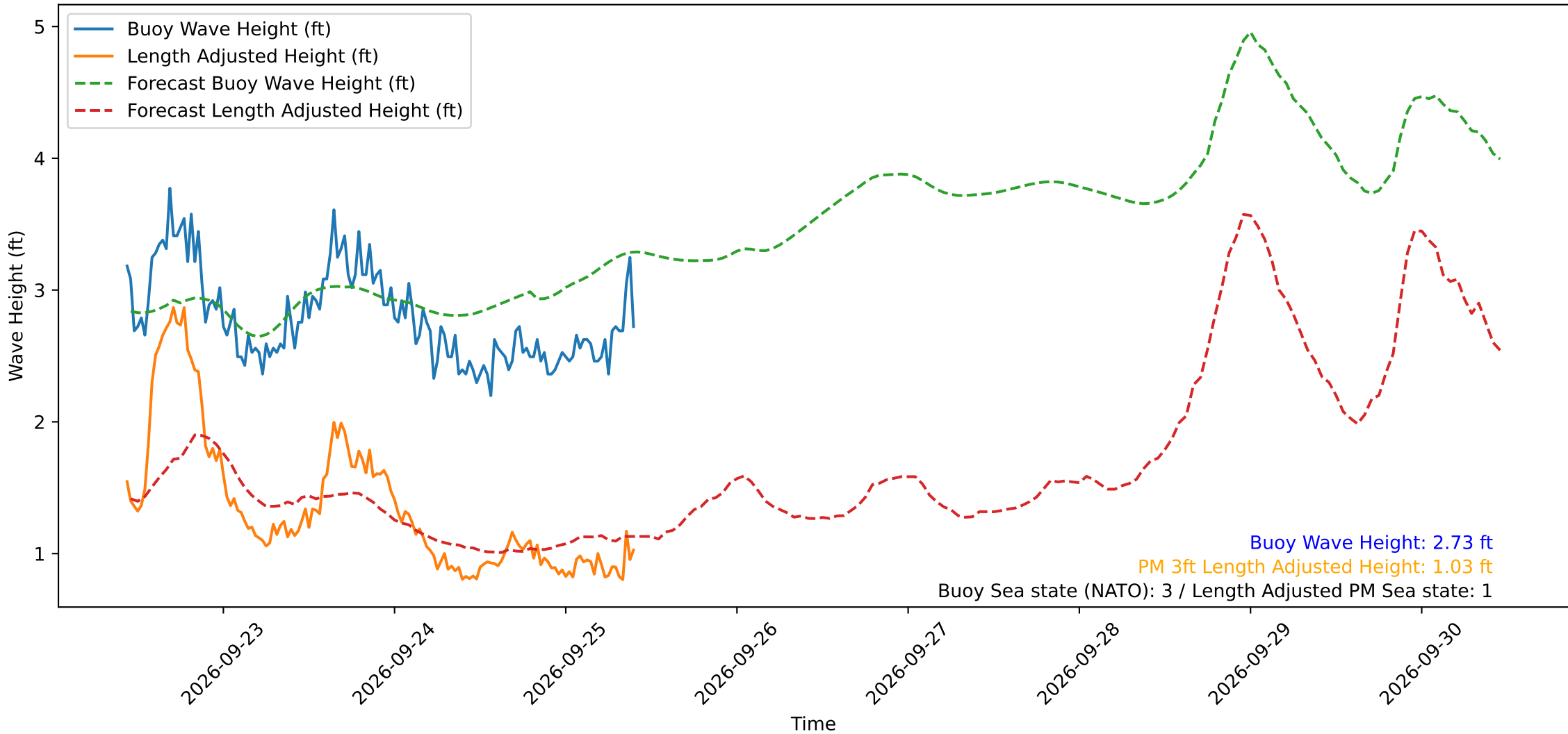
Wave Heights over Time for Oceanside Harbor at 2026-09-25 10:30:29
