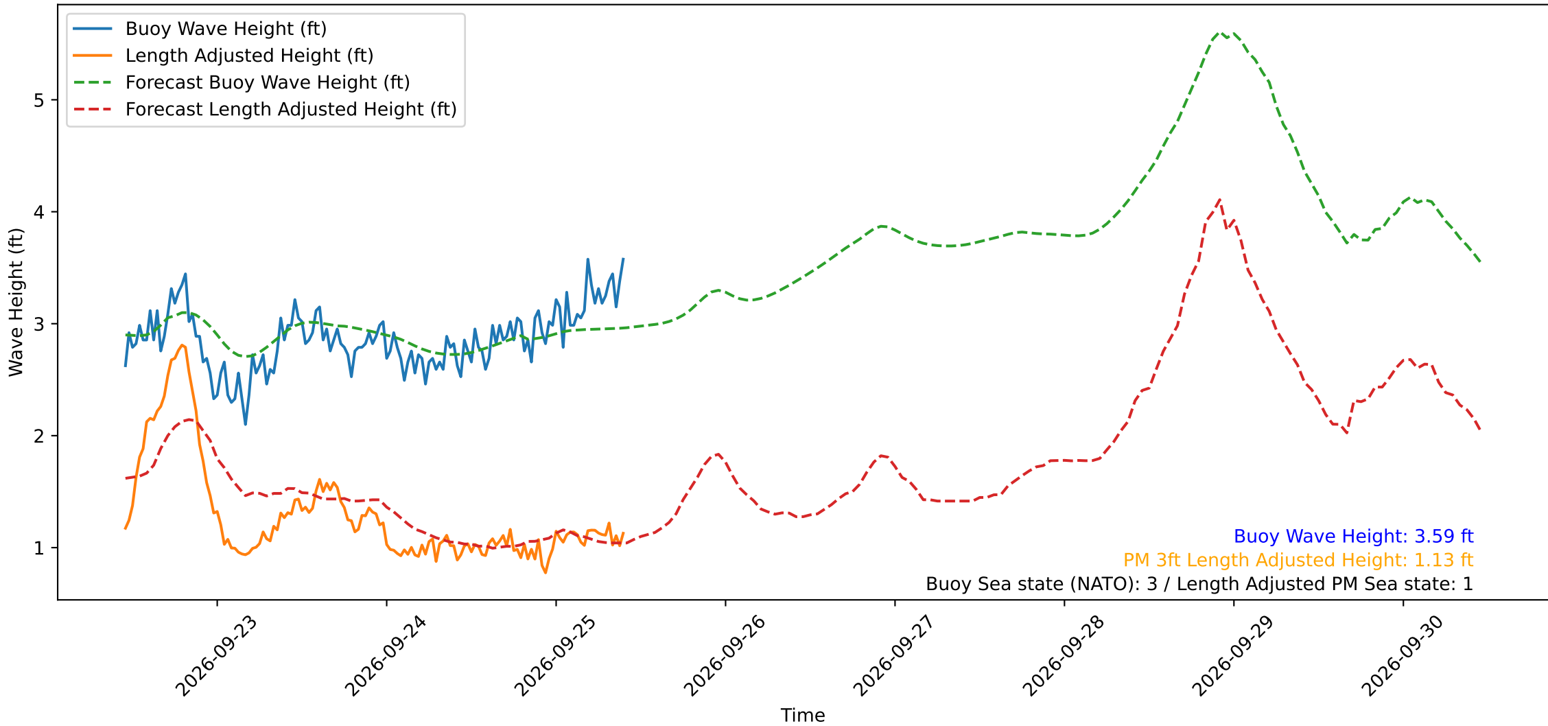
Wave Heights over Time for Green Beach at 2026-09-25 10:31:10
