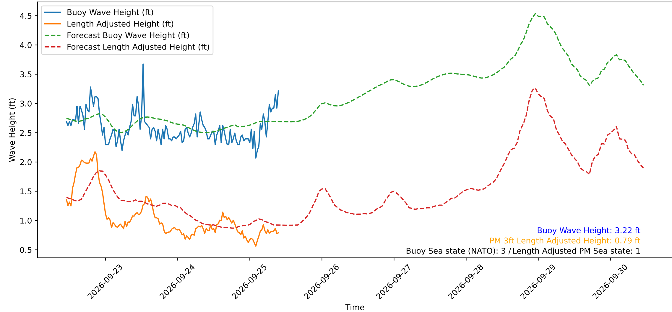
Wave Heights over Time for Red Beach at 2026-09-25 10:30:48
