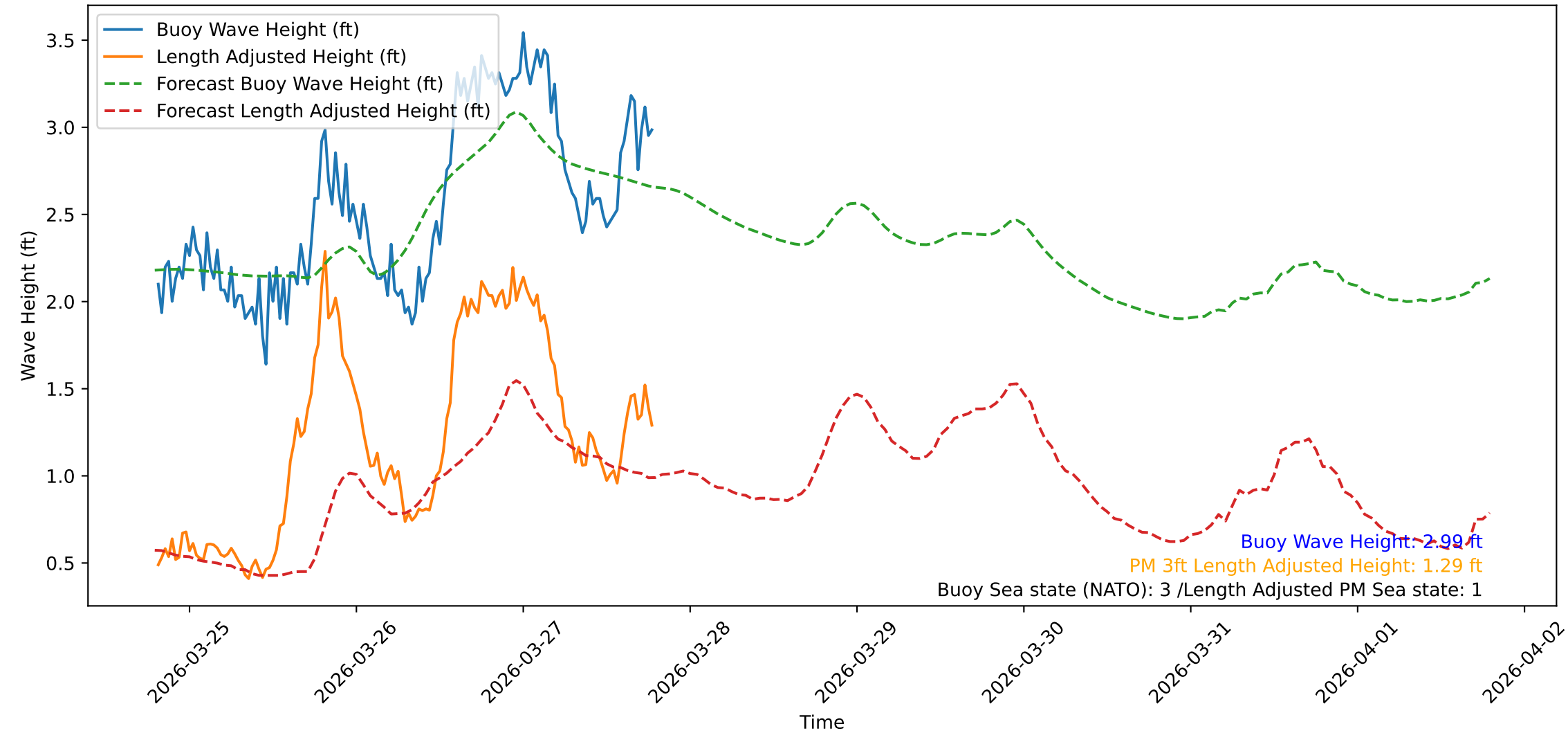
Wave Heights over Time for Green Beach at 2026-03-27 19:21:10
