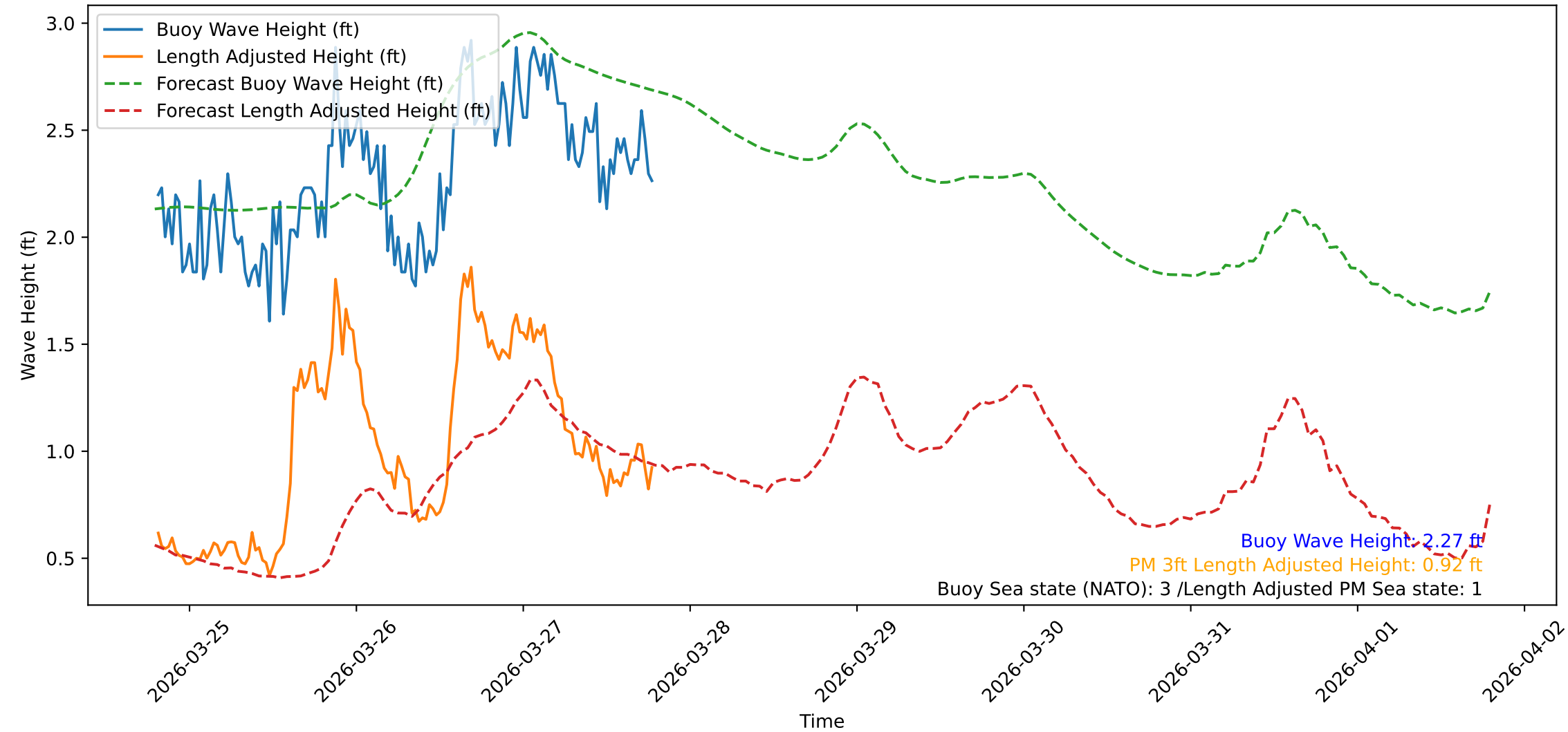
Wave Heights over Time for Oceanside Harbor at 2026-03-27 19:20:31
