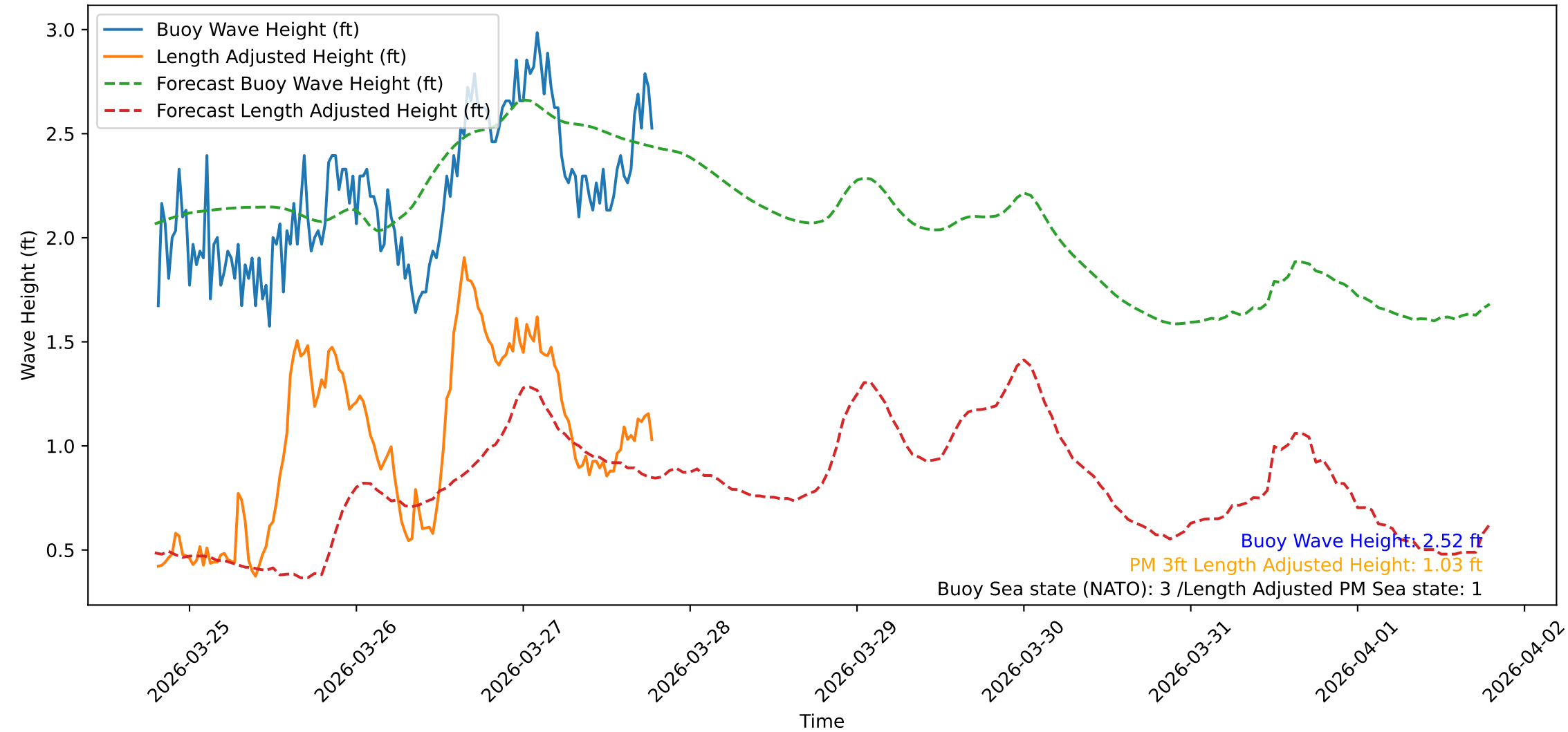
Wave Heights over Time for Red Beach at 2026-03-27 19:20:48
