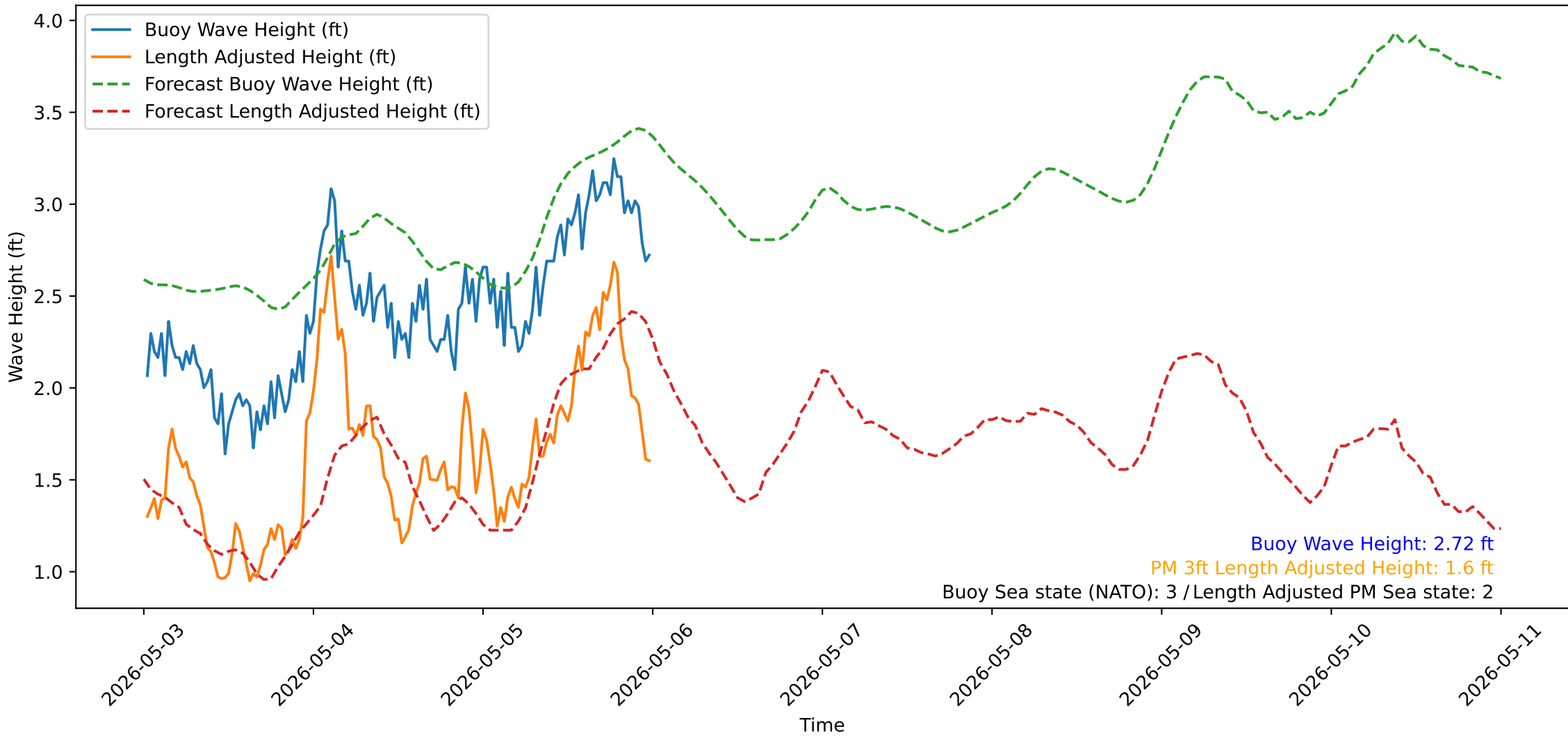
Wave Heights over Time for Oceanside Harbor at 2026-05-06 00:20:31
