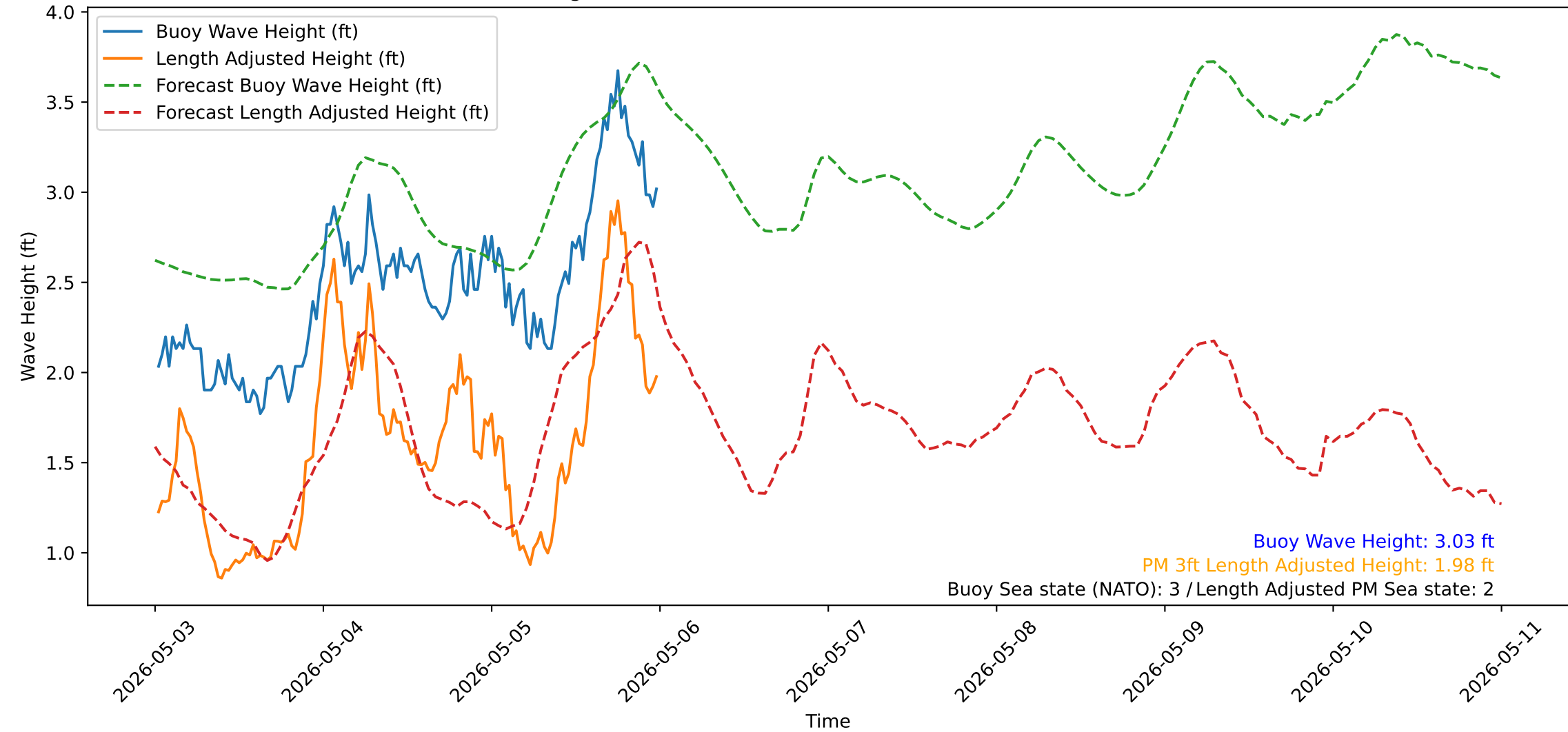
Wave Heights over Time for Green Beach at 2026-05-06 00:21:14
