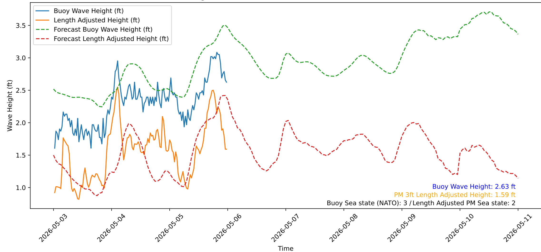
Wave Heights over Time for Red Beach at 2026-05-06 00:20:52
