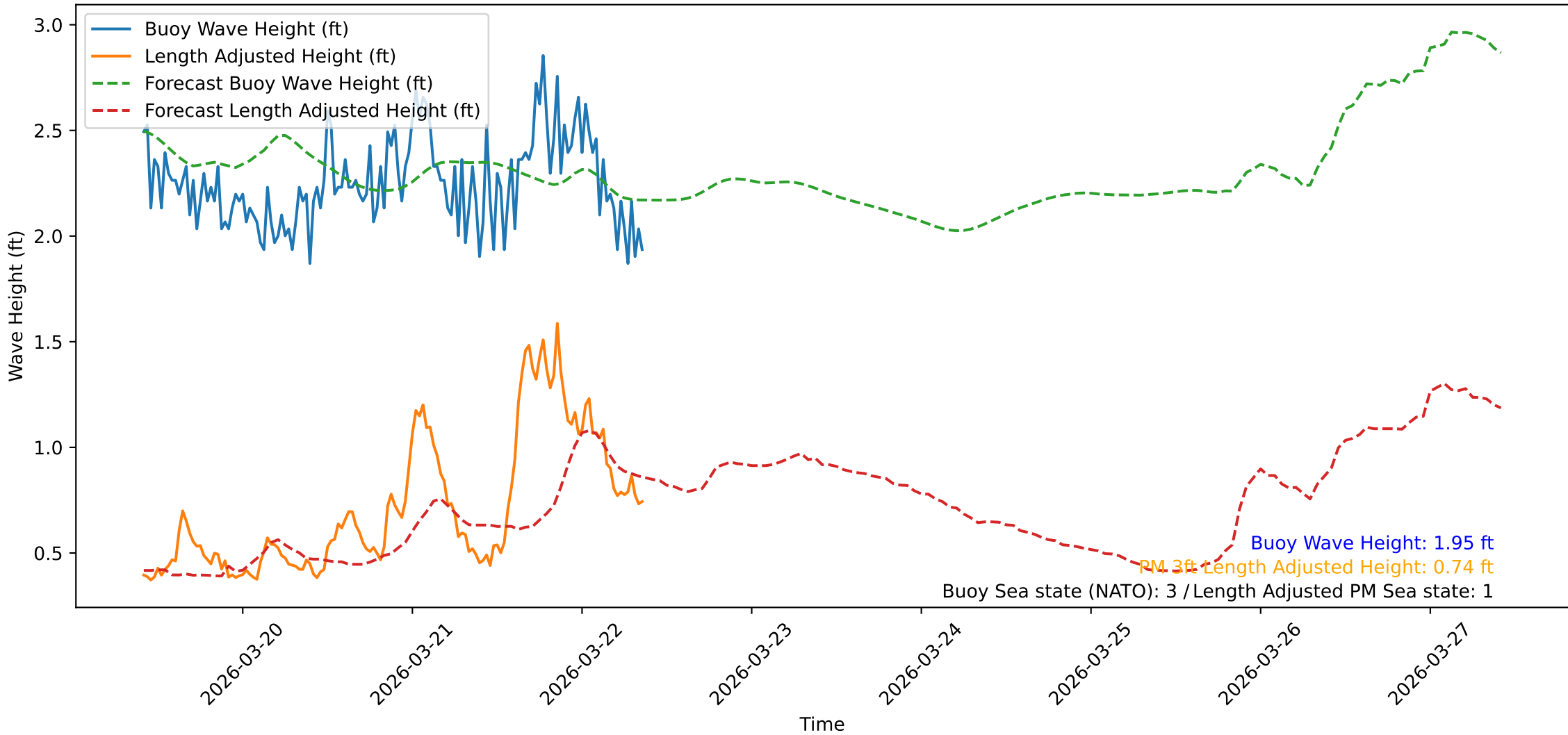
Wave Heights over Time for Red Beach at 2026-03-22 09:30:47
