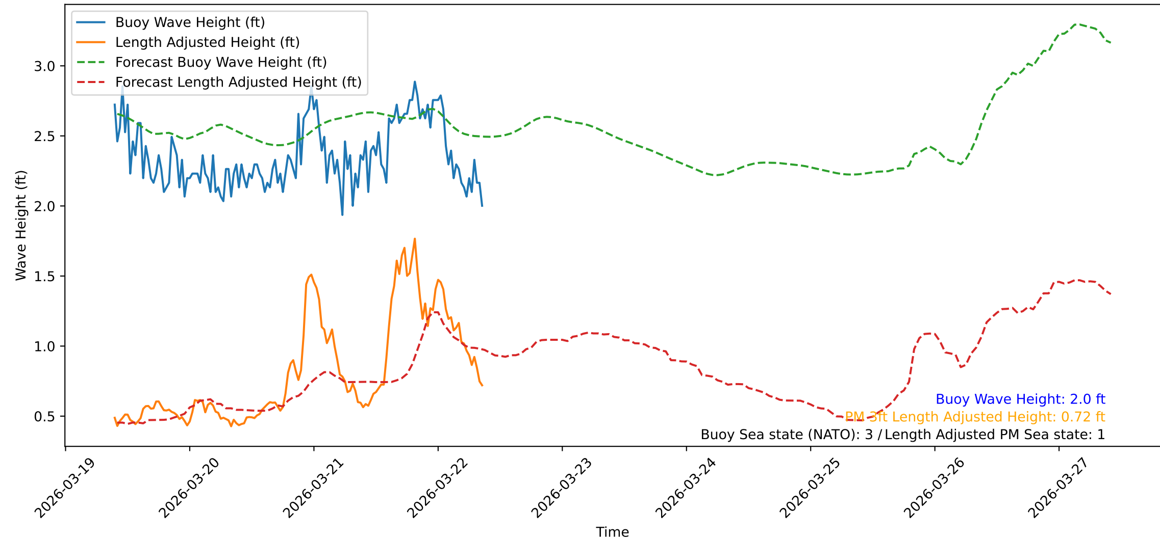
Wave Heights over Time for Green Beach at 2026-03-22 09:31:09
