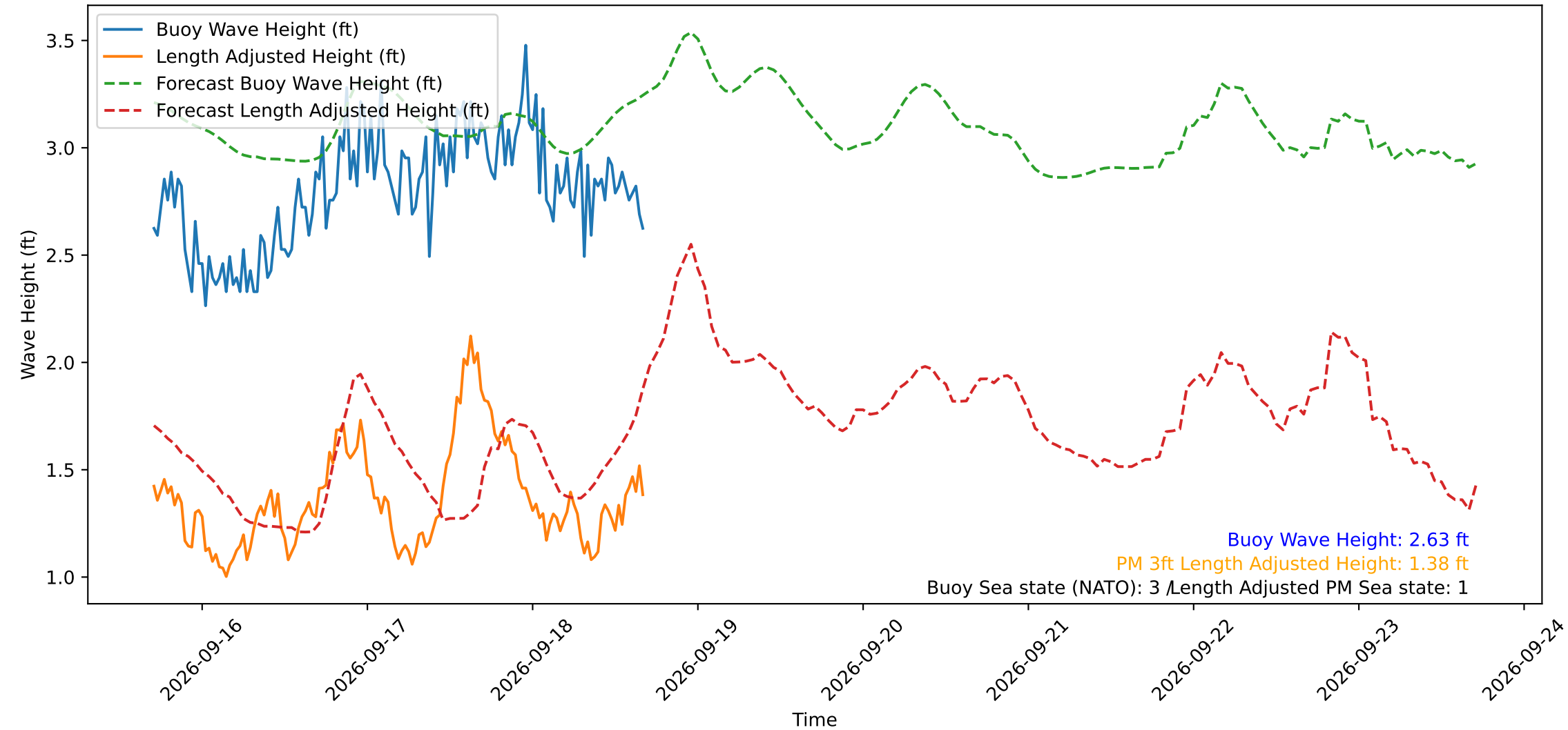
Wave Heights over Time for Green Beach at 2026-09-18 16:41:14
