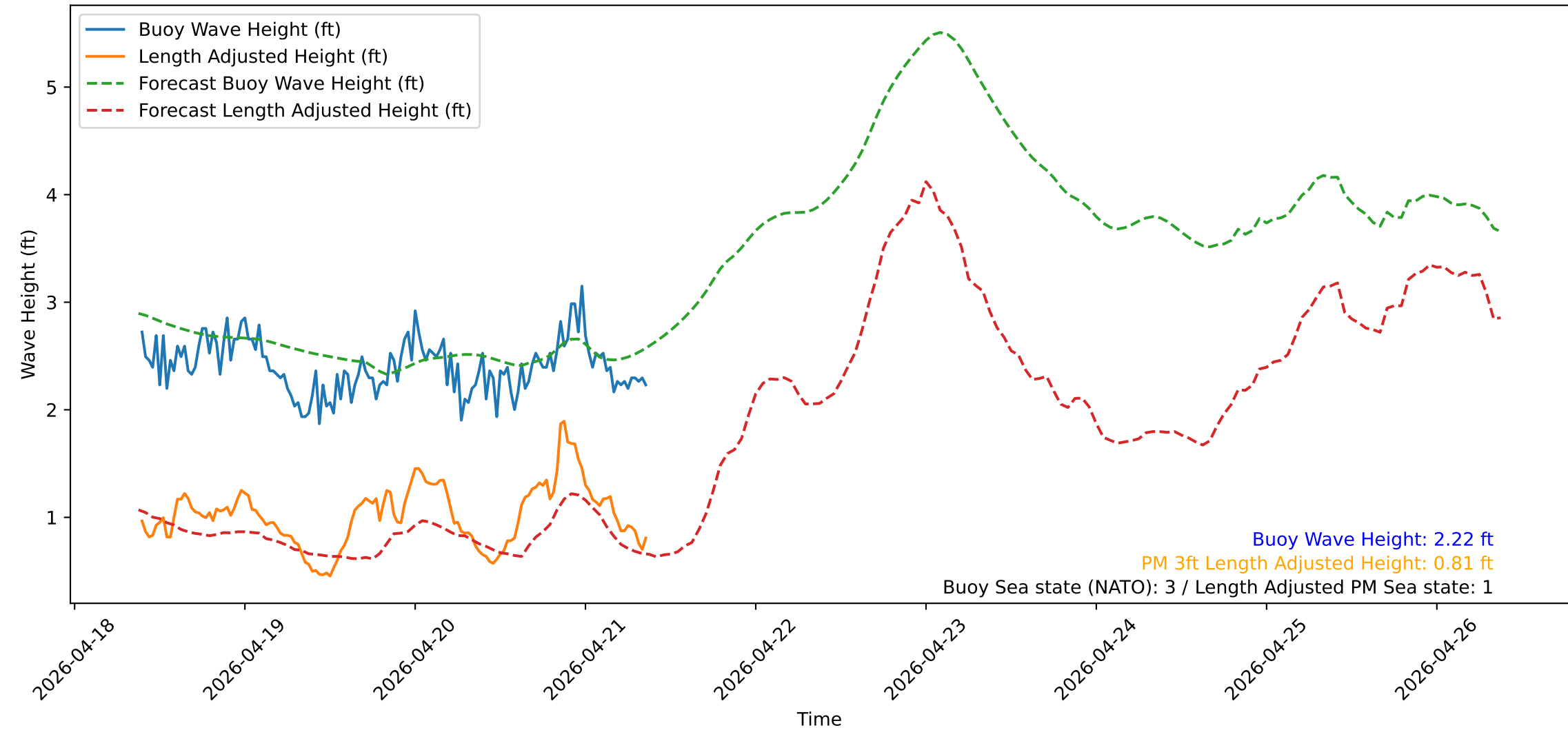
Wave Heights over Time for Green Beach at 2026-04-21 09:21:15
