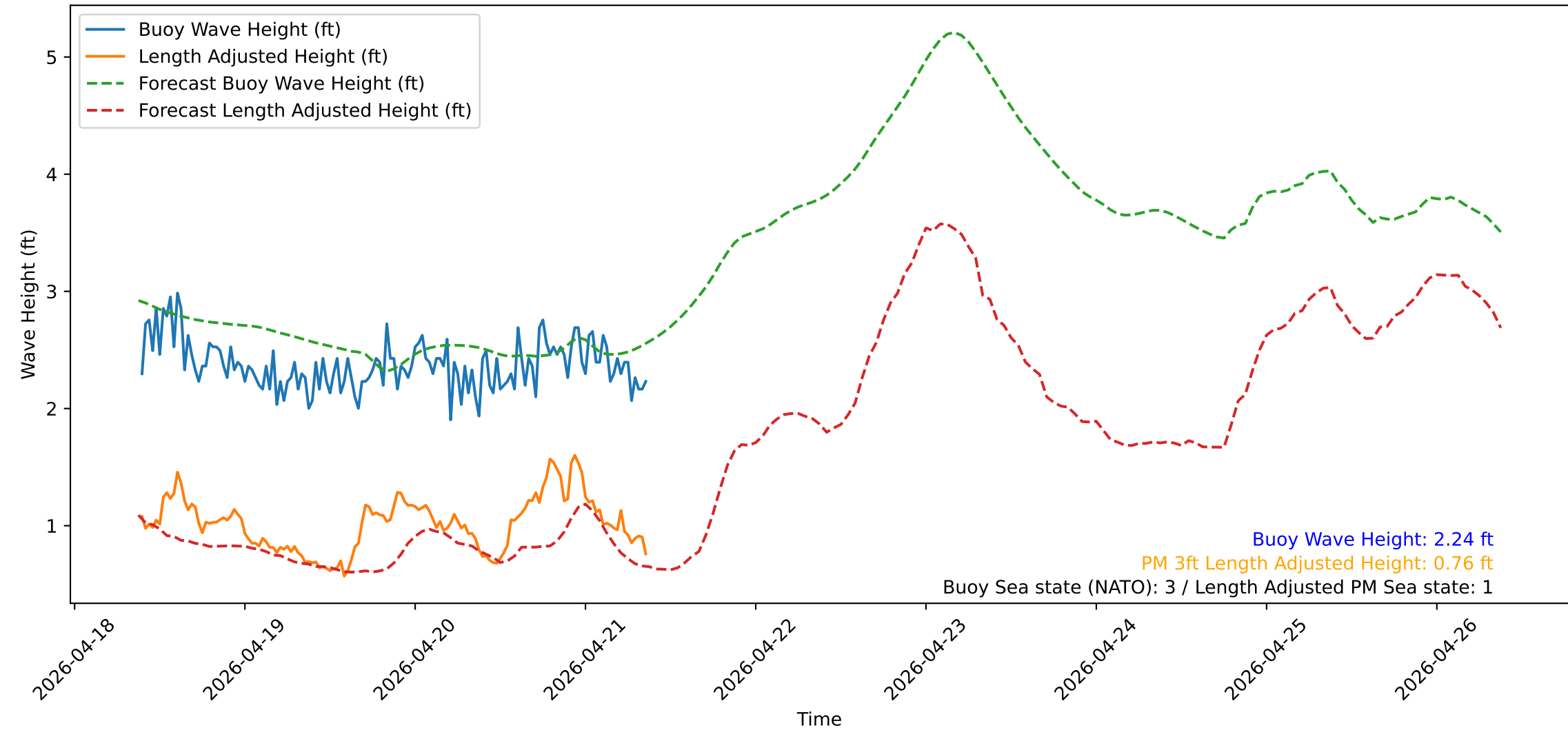
Wave Heights over Time for Oceanside Harbor at 2026-04-21 09:20:32
