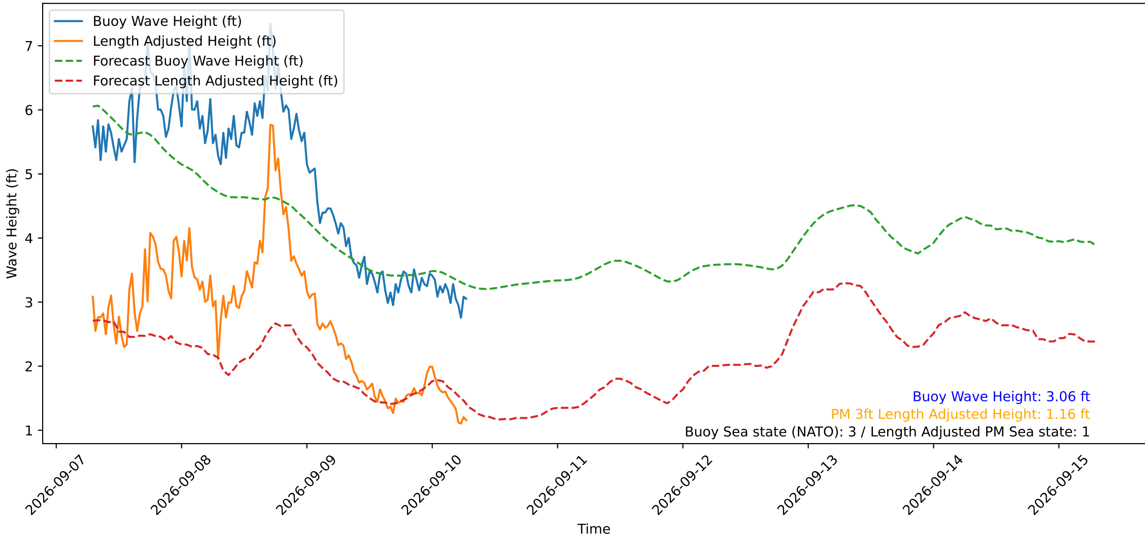
Wave Heights over Time for Oceanside Harbor at 2026-09-10 07:00:30
