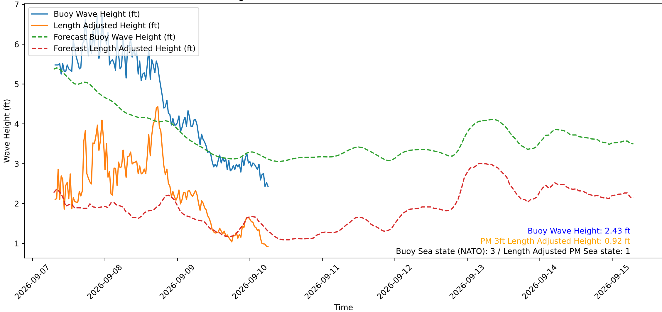
Wave Heights over Time for Red Beach at 2026-09-10 07:00:50
