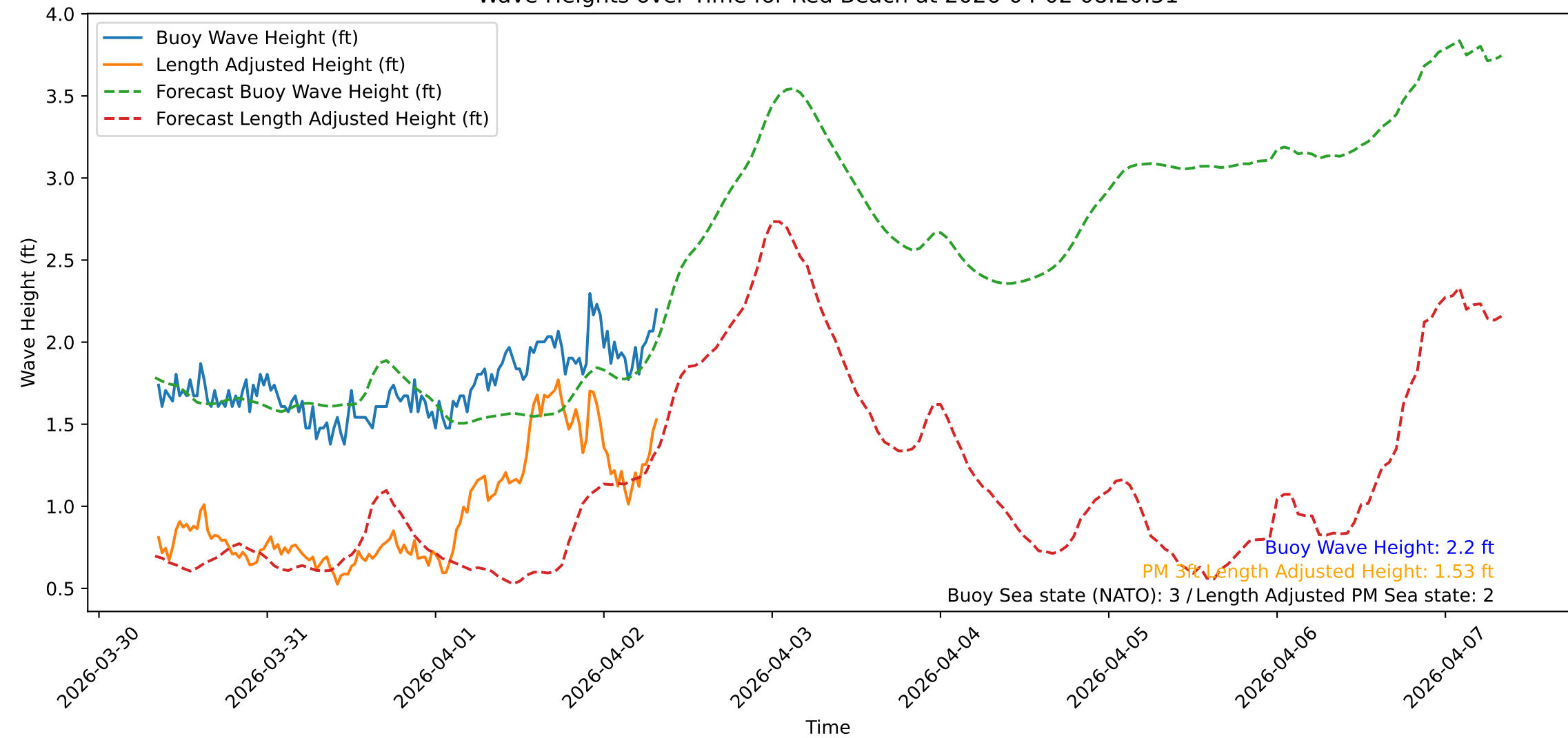
Wave Heights over Time for Red Beach at 2026-04-02 08:20:51
