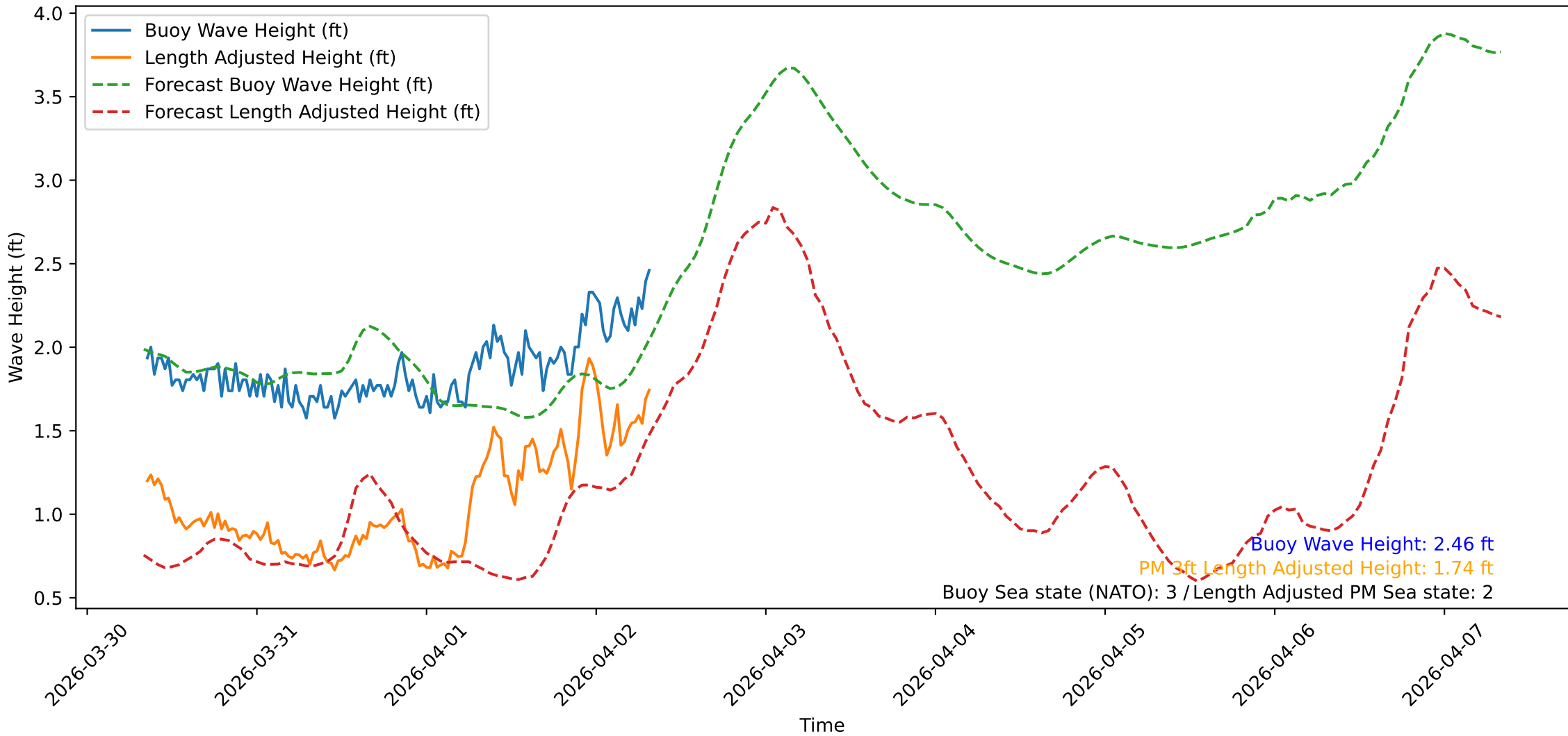
Wave Heights over Time for Oceanside Harbor at 2026-04-02 08:20:35
