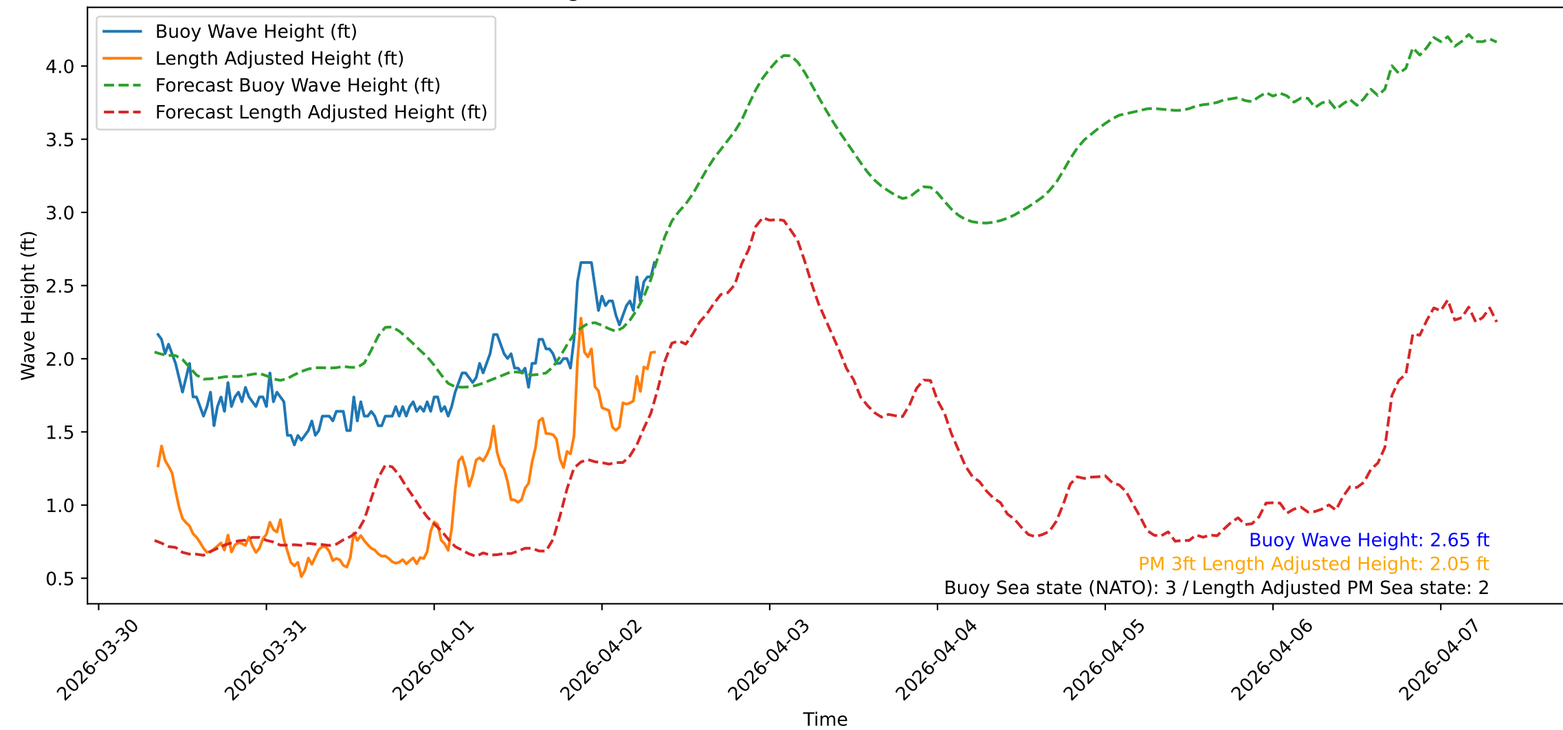
Wave Heights over Time for Green Beach at 2026-04-02 08:21:13
