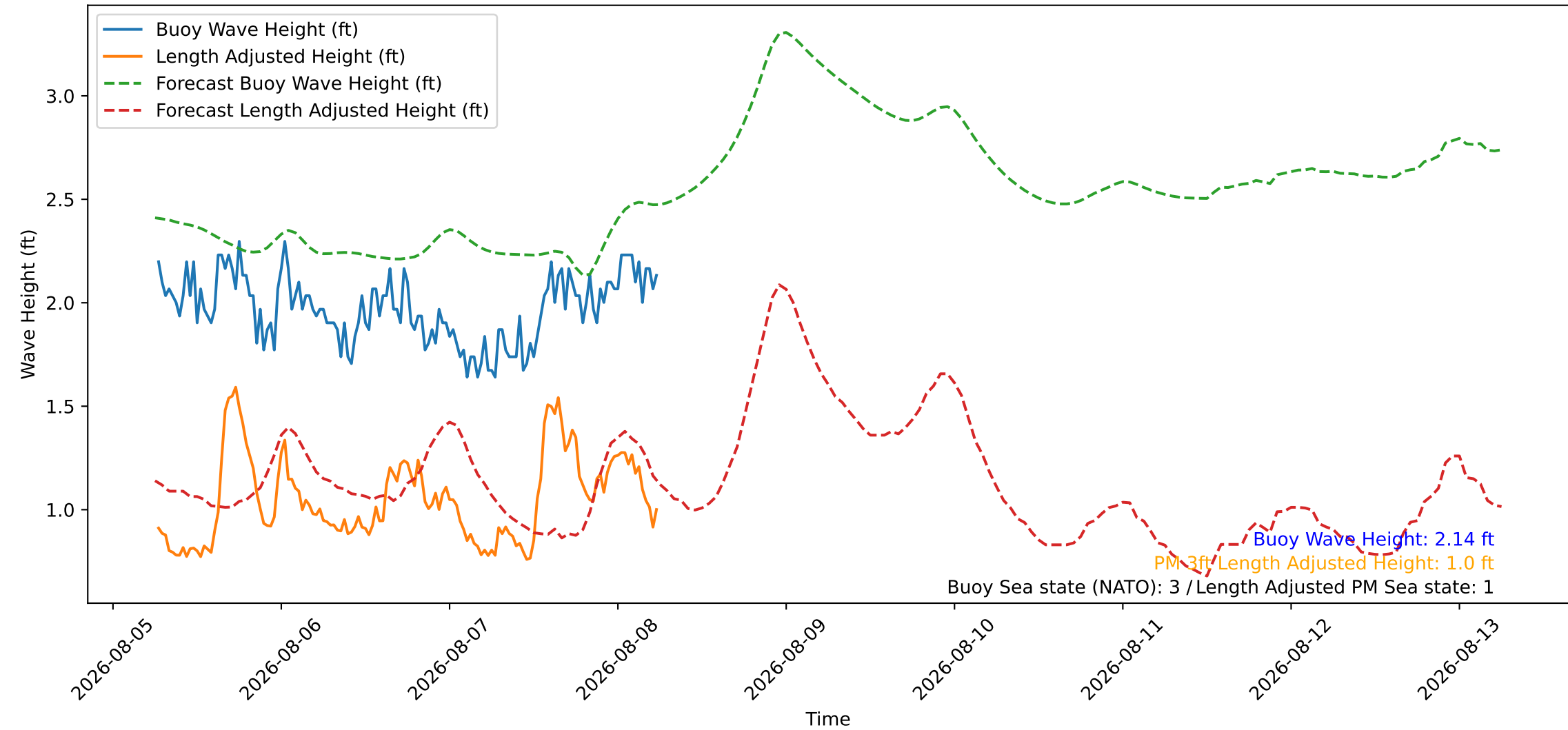
Wave Heights over Time for Oceanside Harbor at 2026-08-08 06:20:26
