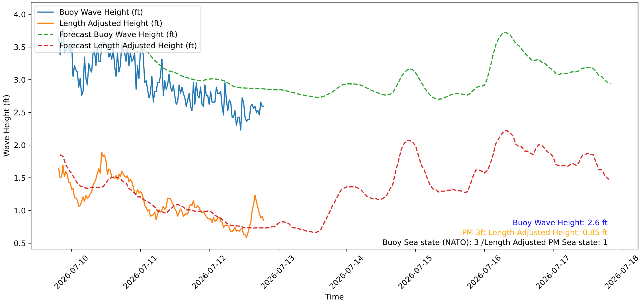
Wave Heights over Time for Green Beach at 2026-07-12 19:41:08
