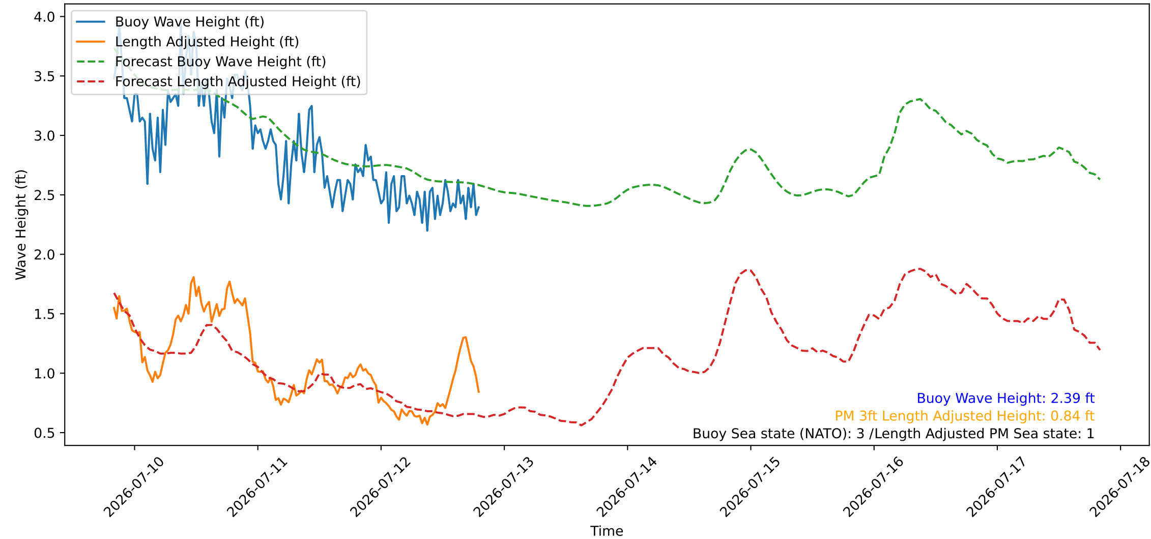
Wave Heights over Time for Red Beach at 2026-07-12 19:40:45
