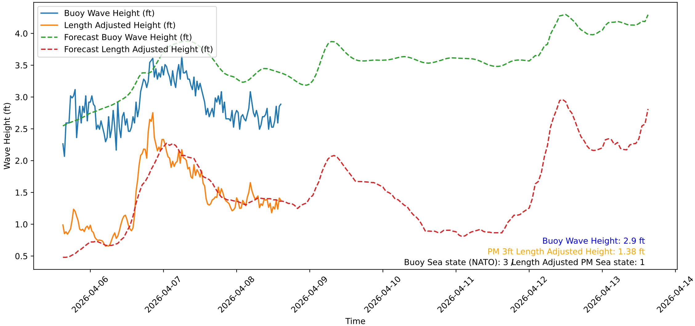
Wave Heights over Time for Oceanside Harbor at 2026-04-08 15:10:31
