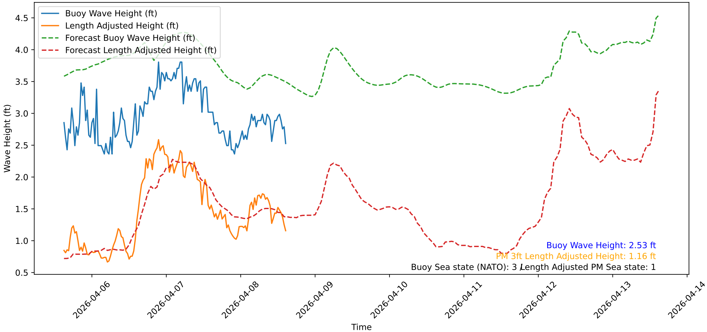
Wave Heights over Time for Green Beach at 2026-04-08 15:11:10
