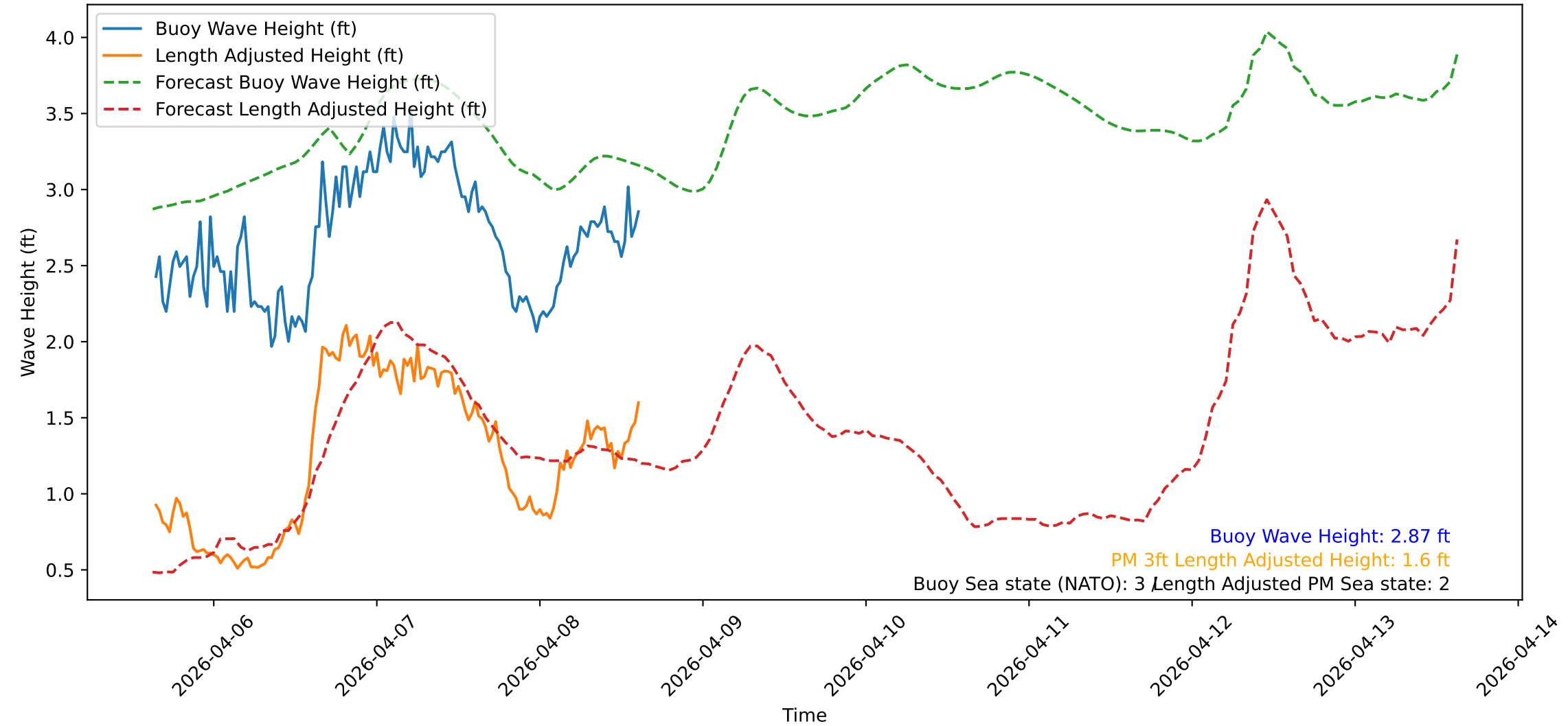
Wave Heights over Time for Red Beach at 2026-04-08 15:10:47
