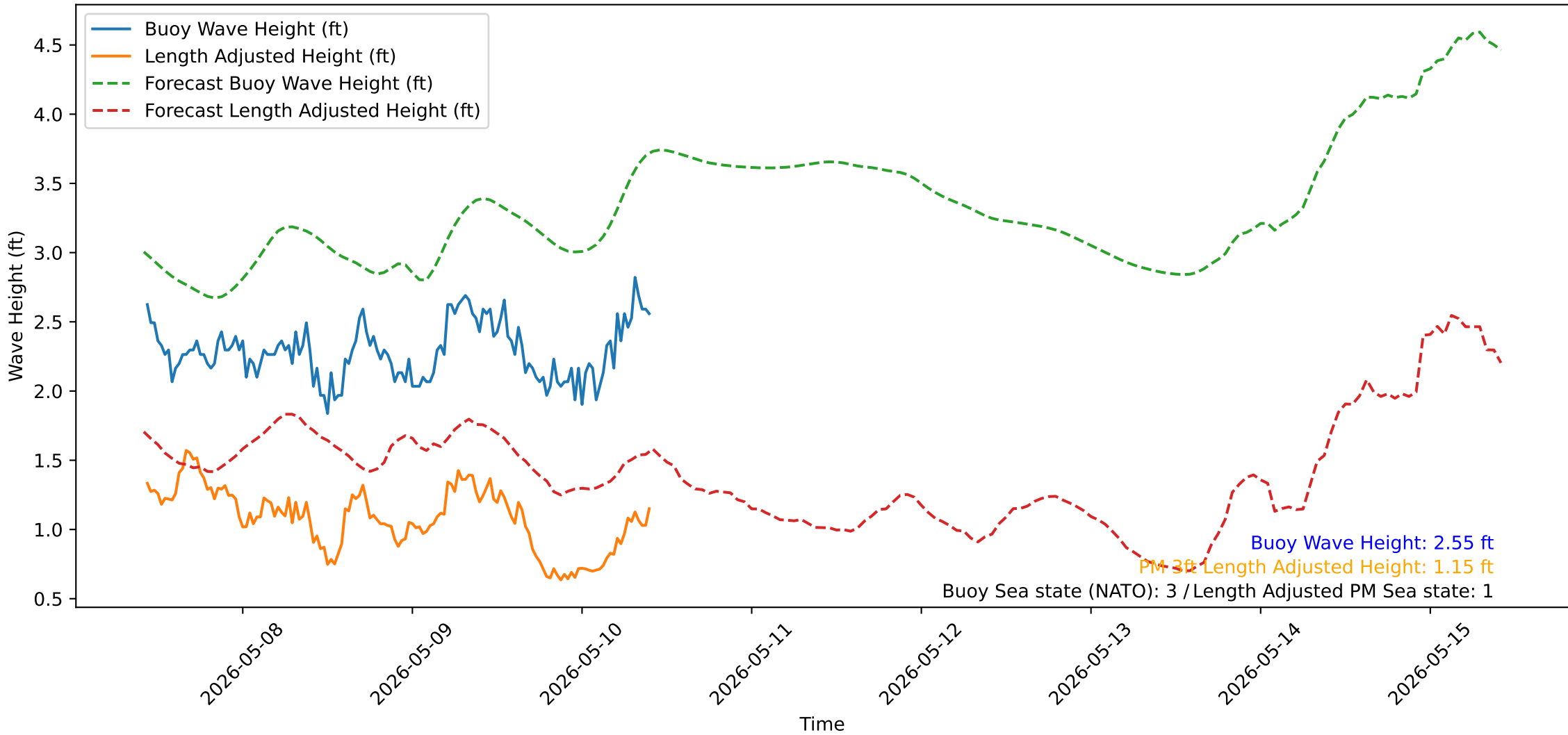
Wave Heights over Time for Green Beach at 2026-05-10 10:21:15
