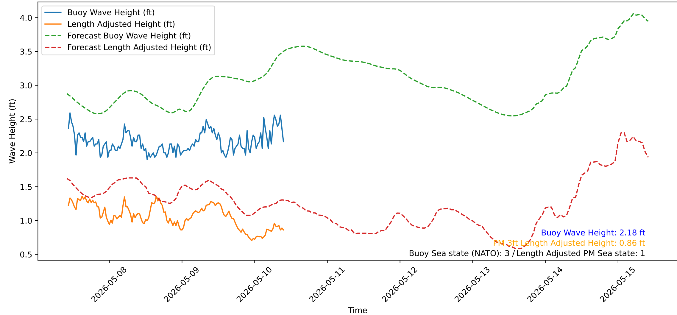
Wave Heights over Time for Red Beach at 2026-05-10 10:20:52
