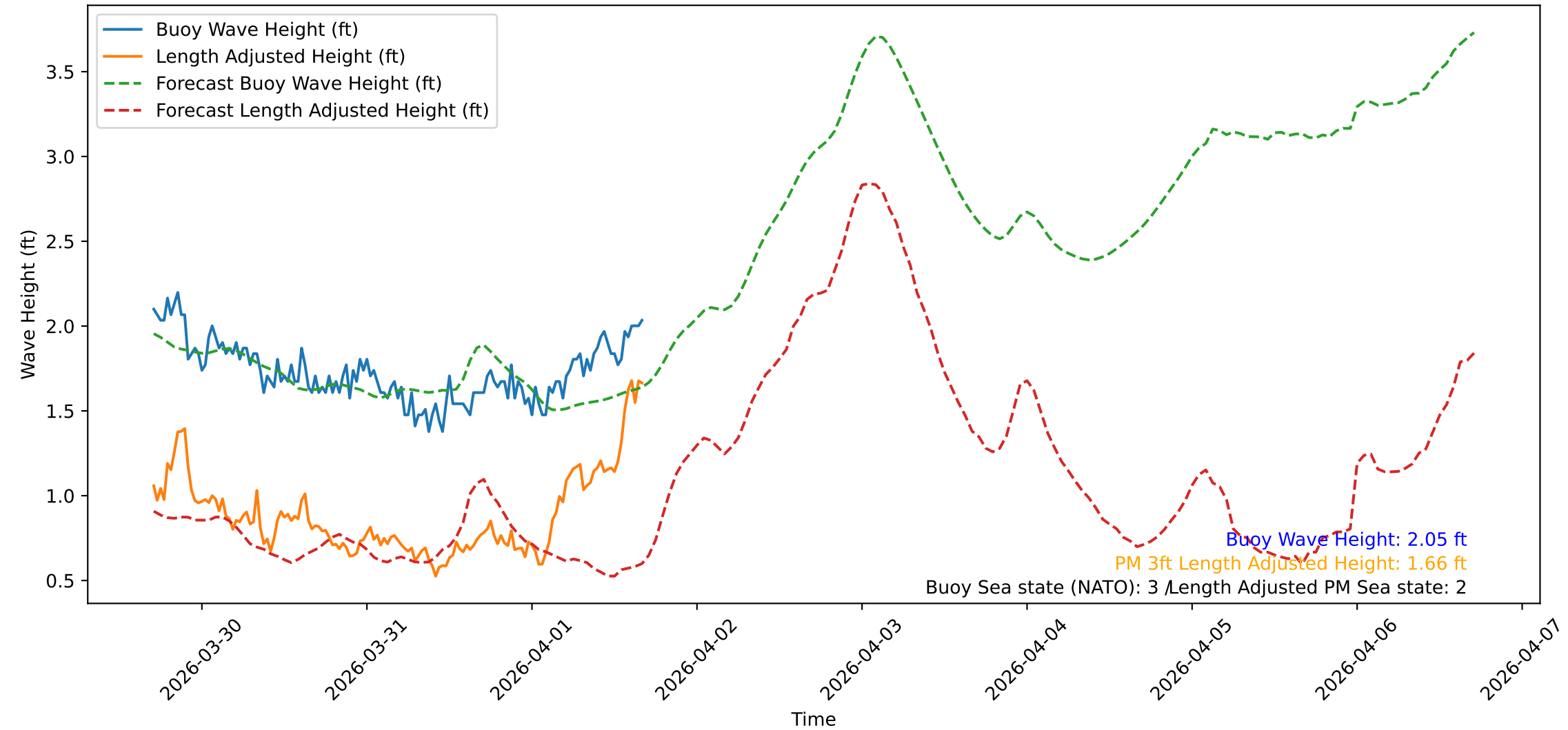
Wave Heights over Time for Red Beach at 2026-04-01 16:50:48
