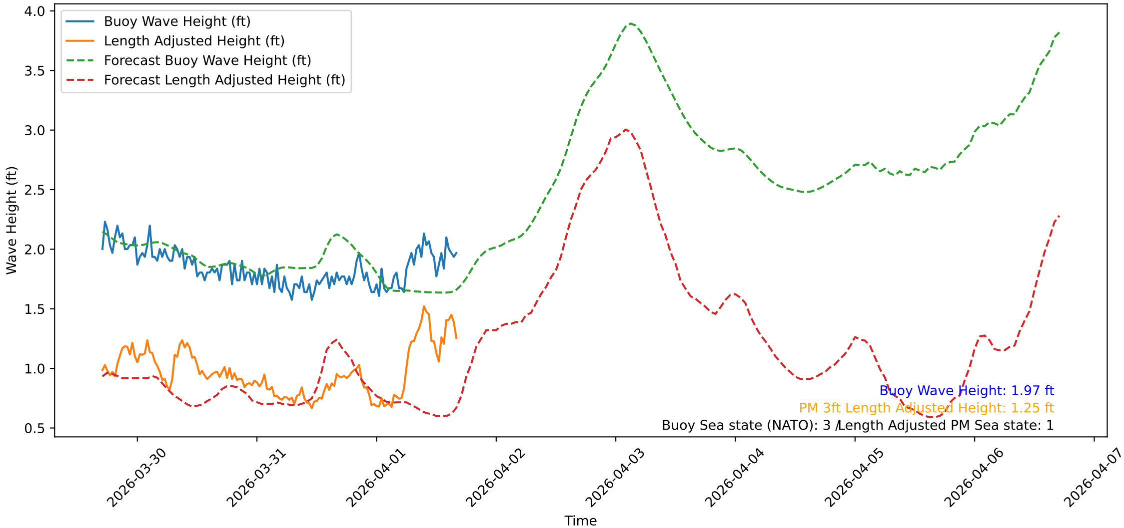
Wave Heights over Time for Oceanside Harbor at 2026-04-01 16:50:31
