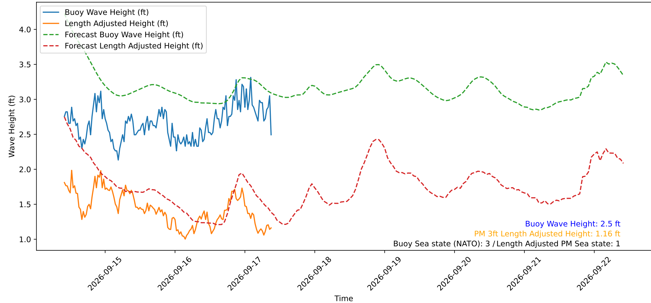
Wave Heights over Time for Green Beach at 2026-09-17 09:41:11
