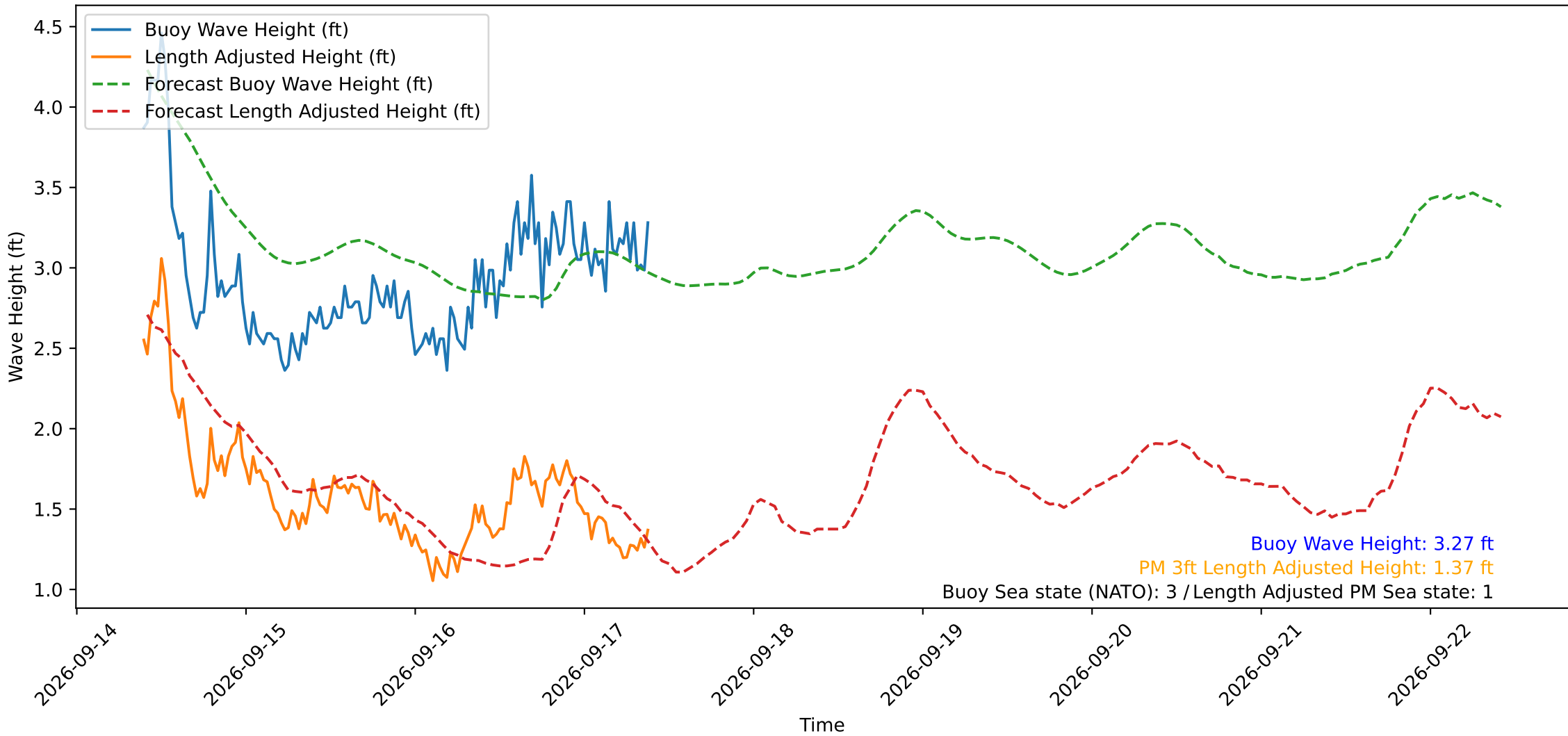
Wave Heights over Time for Oceanside Harbor at 2026-09-17 09:40:29
