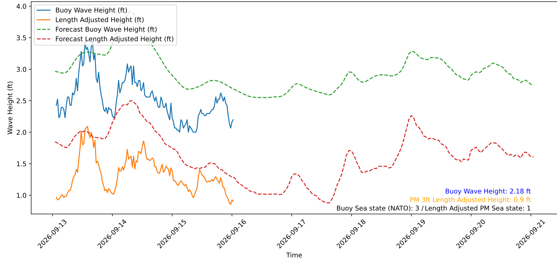
Wave Heights over Time for Red Beach at 2026-09-16 01:20:50
