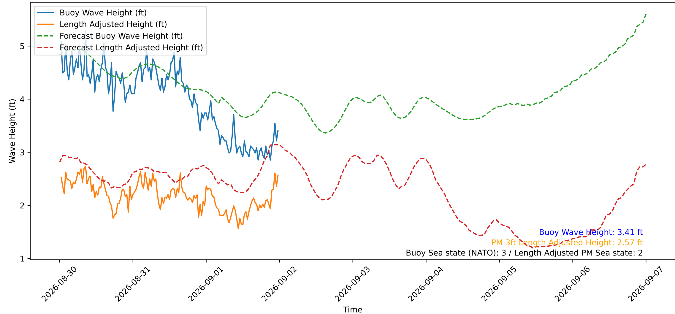
Wave Heights over Time for Oceanside Harbor at 2026-09-02 00:20:30
