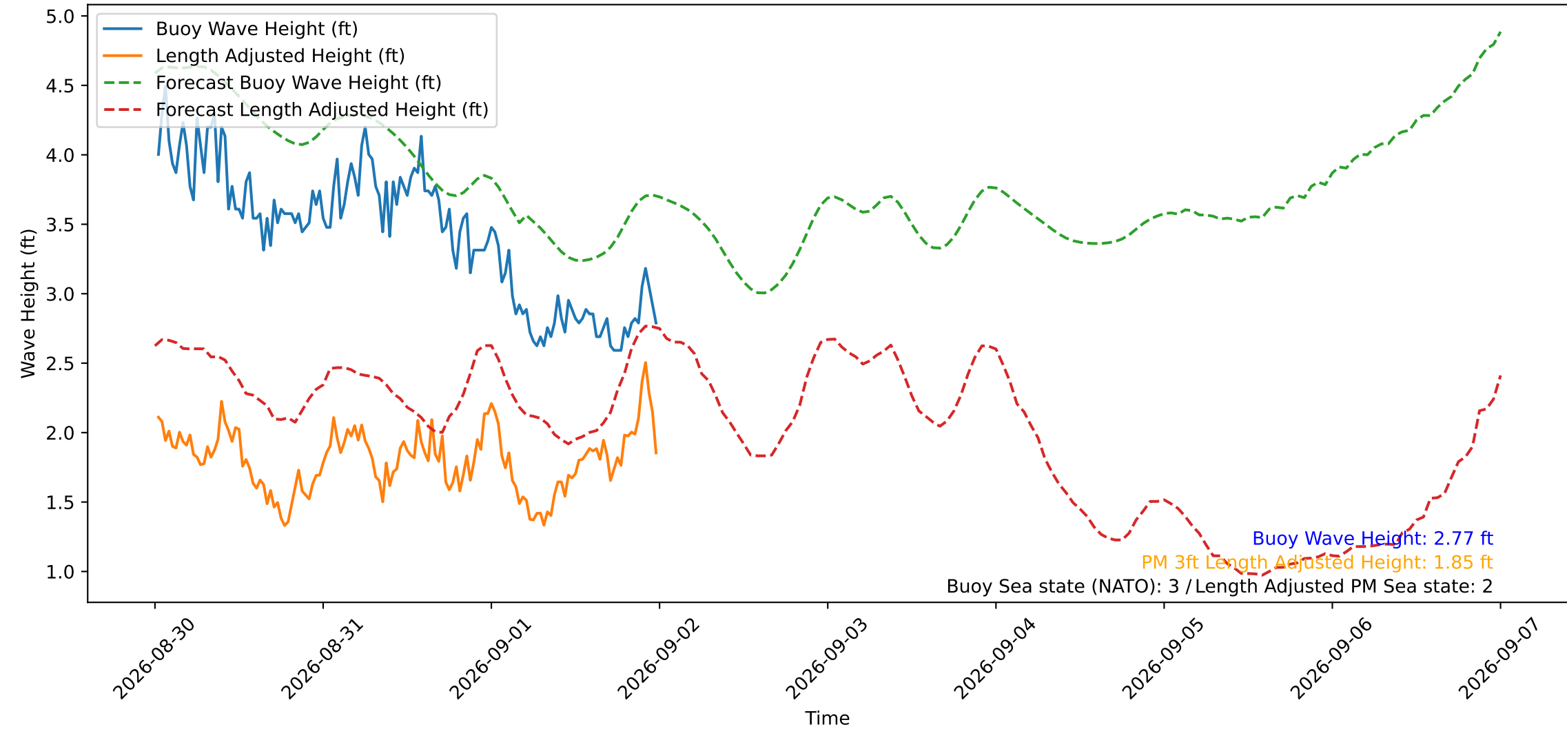
Wave Heights over Time for Red Beach at 2026-09-02 00:20:51
