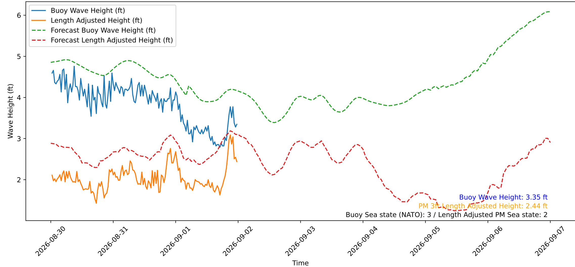
Wave Heights over Time for Green Beach at 2026-09-02 00:21:15
