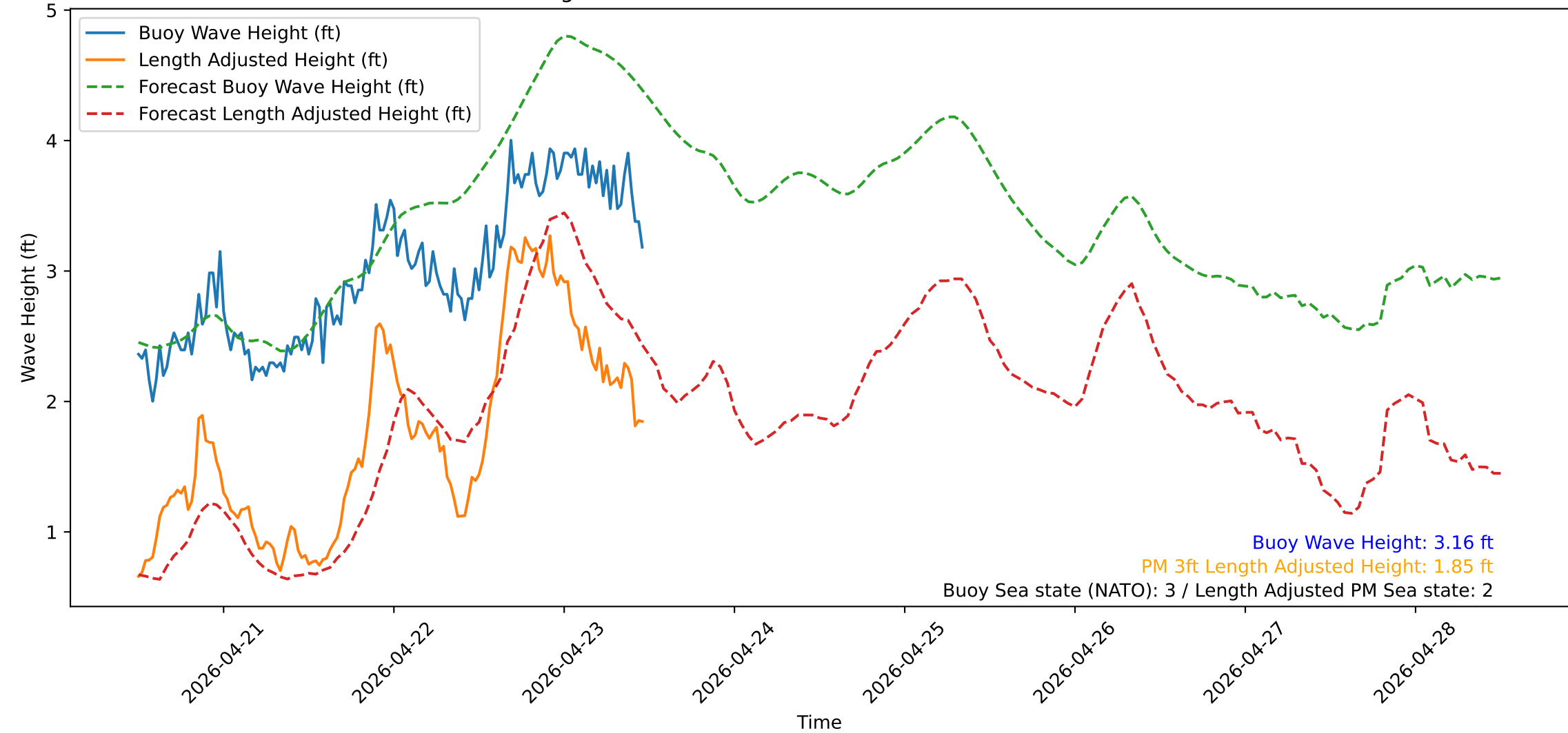
Wave Heights over Time for Green Beach at 2026-04-23 11:51:13
