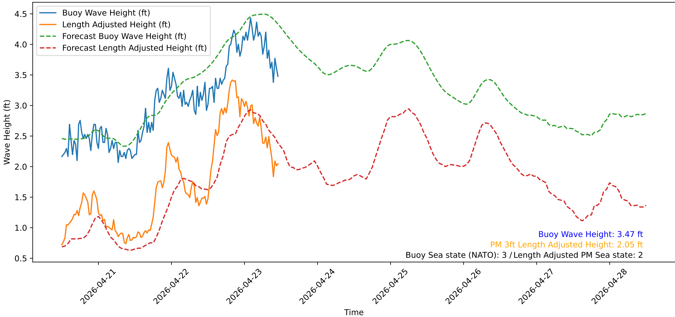
Wave Heights over Time for Oceanside Harbor at 2026-04-23 11:50:31
