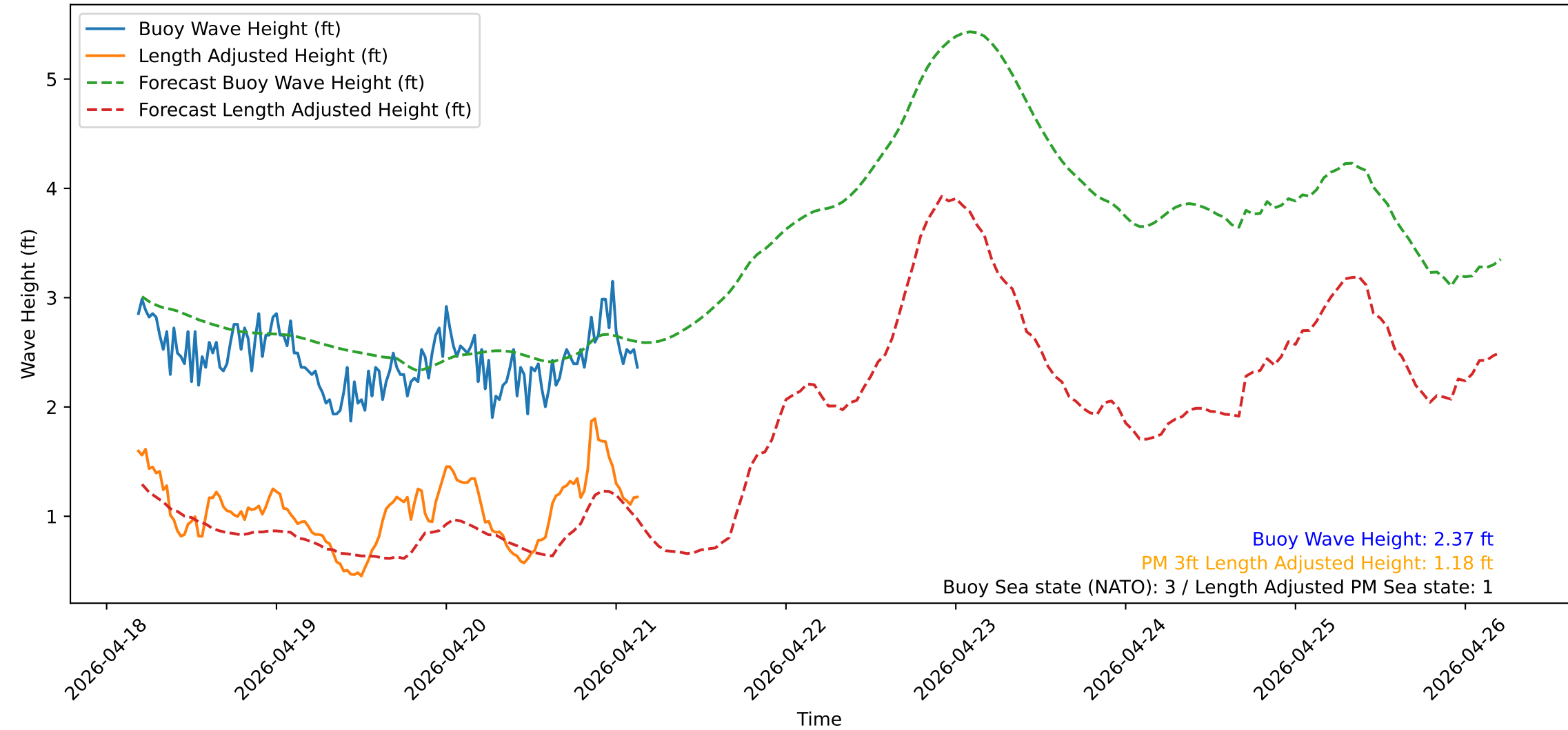
Wave Heights over Time for Green Beach at 2026-04-21 04:31:13
