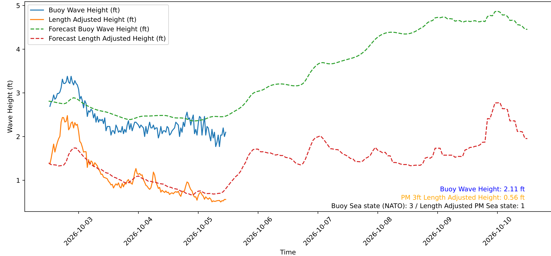
Wave Heights over Time for Green Beach at 2026-10-05 12:01:11
