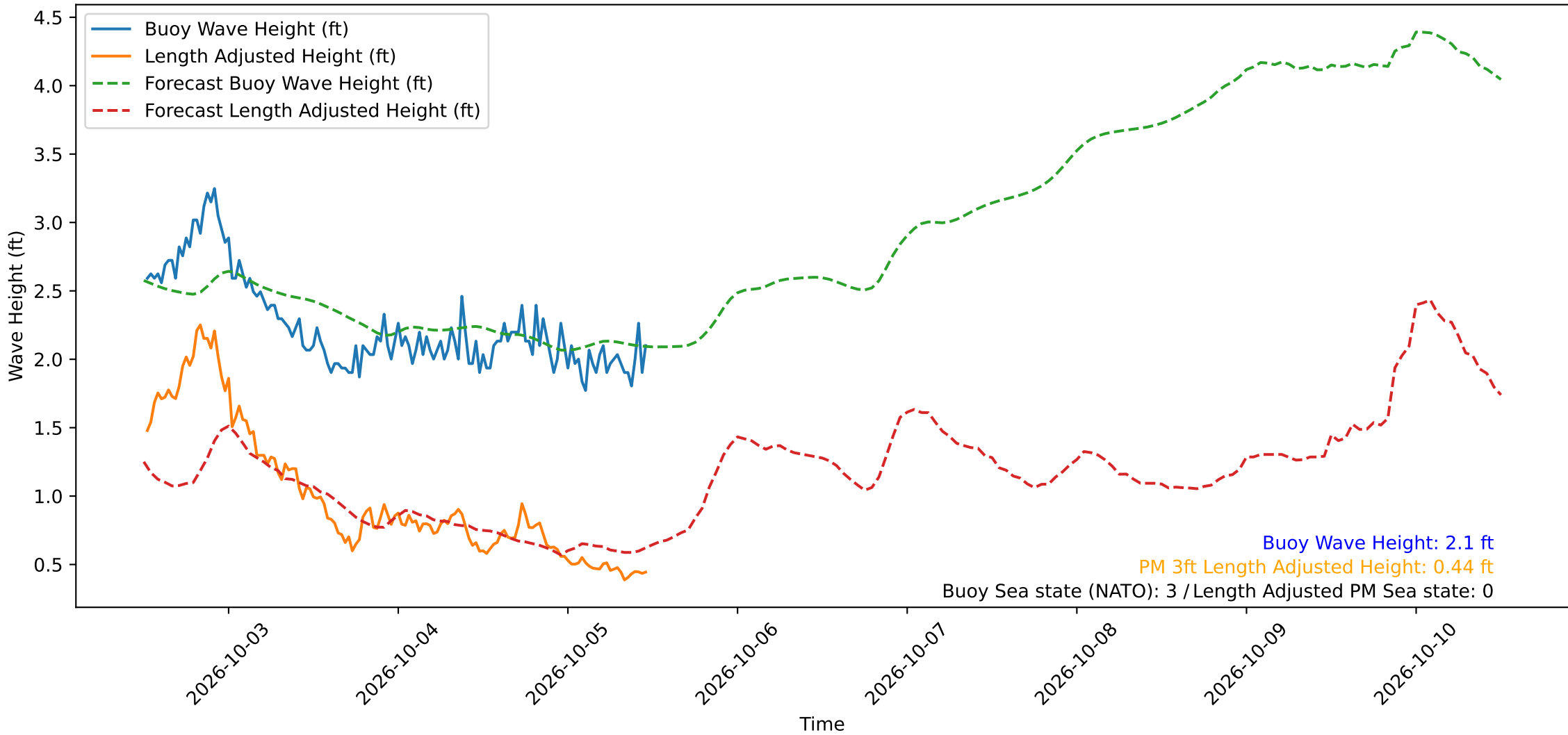
Wave Heights over Time for Red Beach at 2026-10-05 12:00:48
